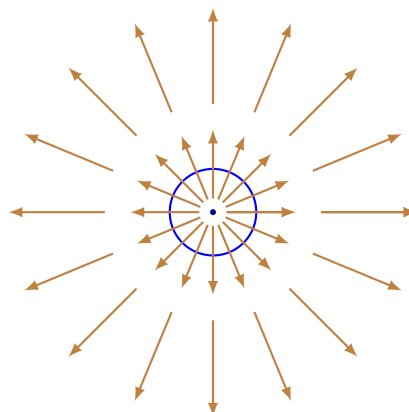
Figure 4. One isolated equilibrium (source) inside the closed curve \Rightarrow index = 1
