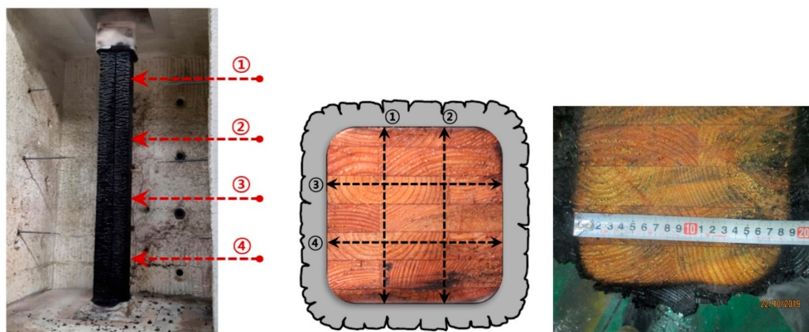
Figure 5. Charring depth measurement of sample: (a) measurement location after fire test, (b) charring depth measurement point, and (c) charring depth measurement.
