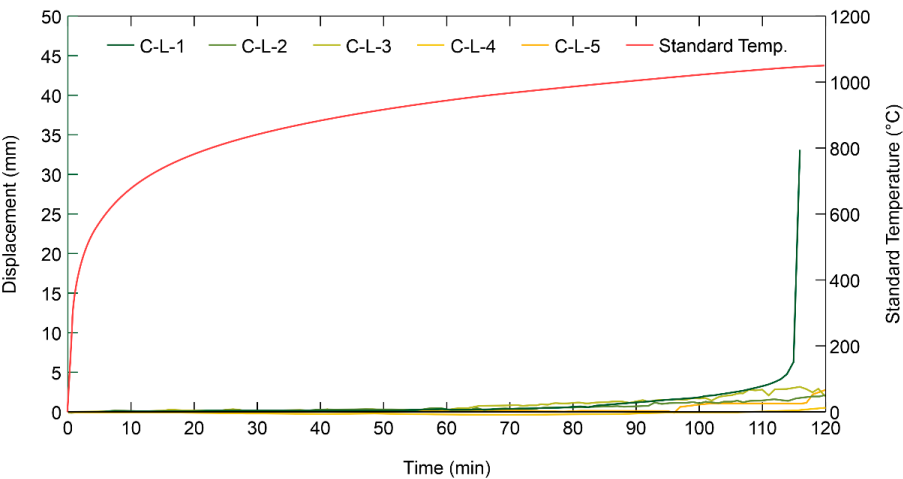
Figure 6. Behavior of samples with a time displacement.
