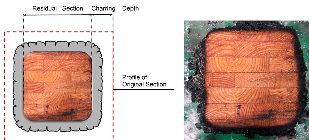
Figure 1. Charring layer of timber exposed to fire: (a) Residual cross-section of timber column exposed to fire, and (b) Cross-section of timber column after fire test.
