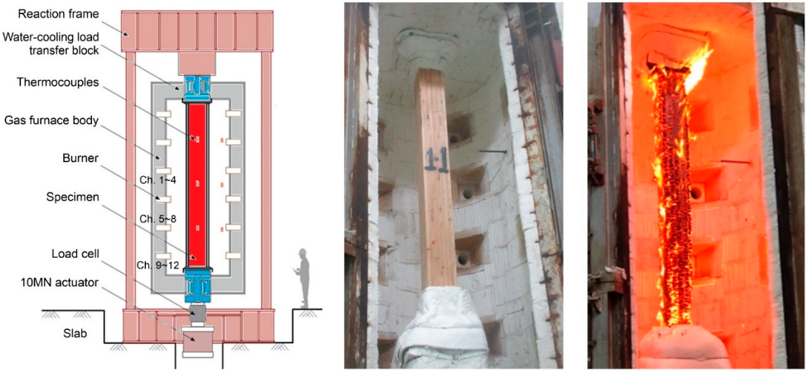
Figure 4. Design concepts for fire-resistant timber members: (a) column fire test in furnace, (b) sample before fire test, and (c) sample after fire test.
