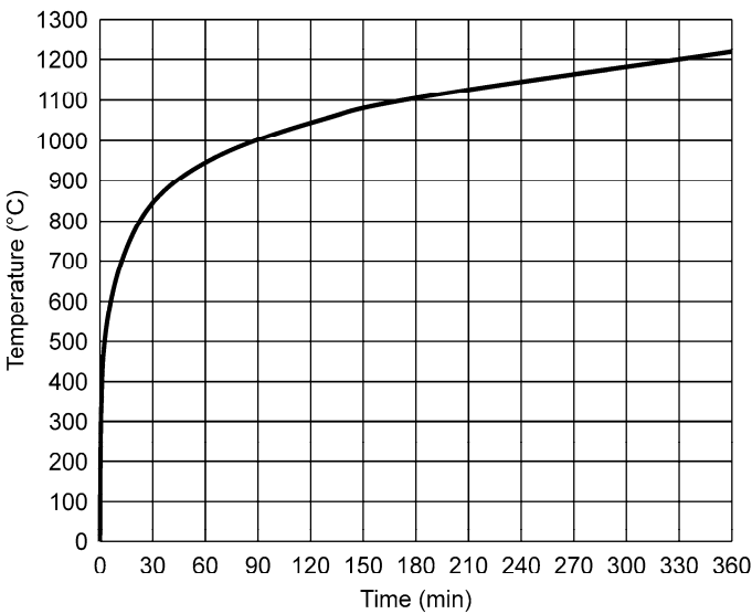
Figure 3. Standard time-temperature curve (ISO 834).
