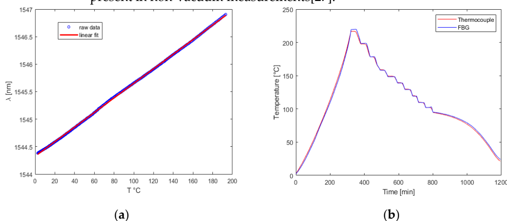
Figure 8 Test cycle 1: (a) Single FBG calibration curve; (b) Comparison between FBG and thermocouple.
