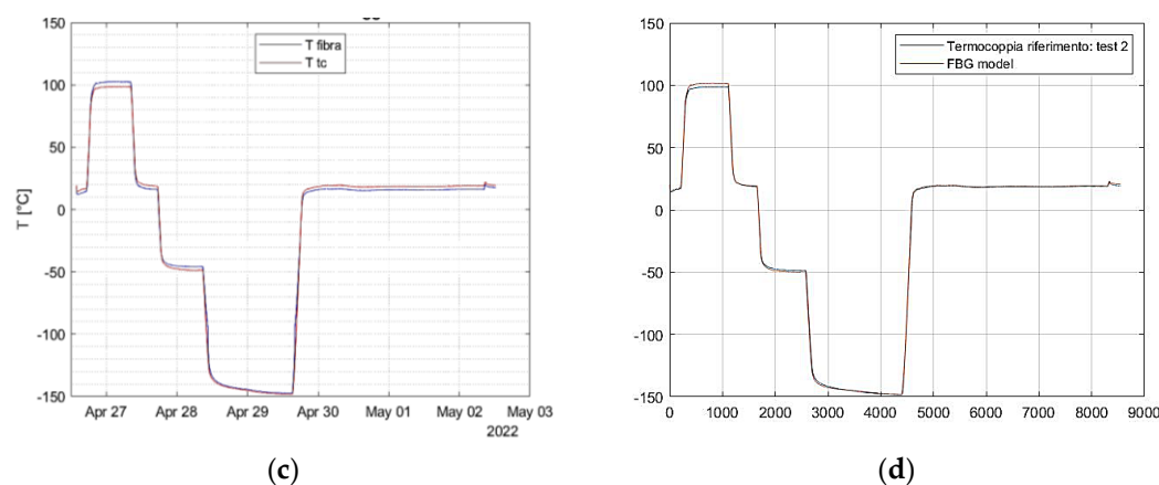
Figure 10 Test cycle 2: (a)Single FBG calibration curve; (b) Boxplot of calculated coefficients;(c) Linear interpolated data;(d) Fourier Interpolated Data.
