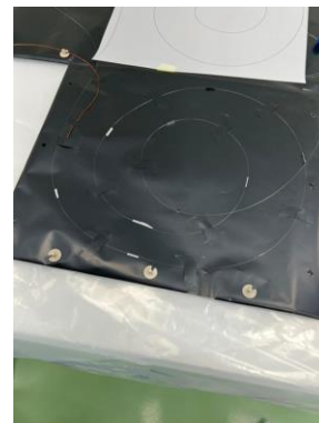
Figure 1 MLI Blankets with Integrated FBG Sensors
