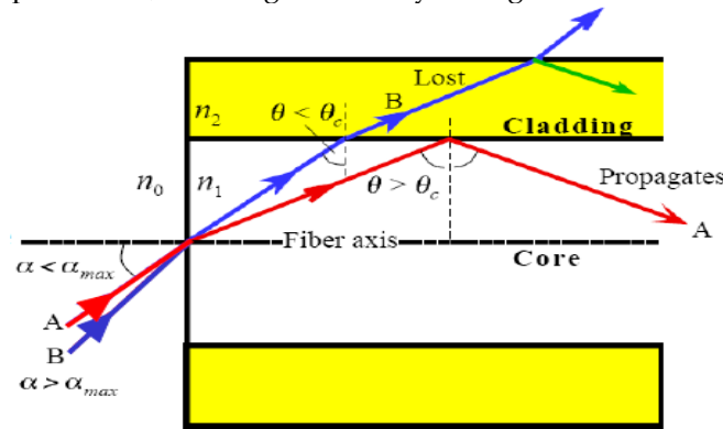
Figure 2 Scheme of optical fiber working principle [24]
