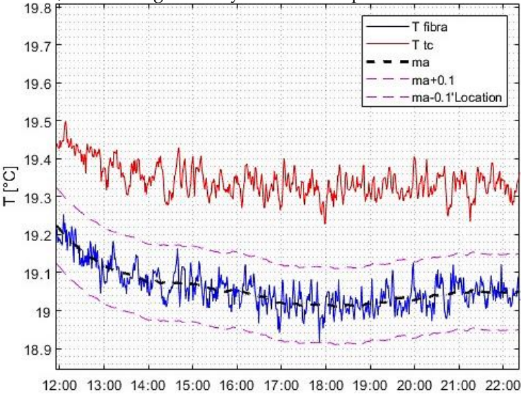
Figure 12 Detailed comparison between FBG and thermocouple performances and stability.
