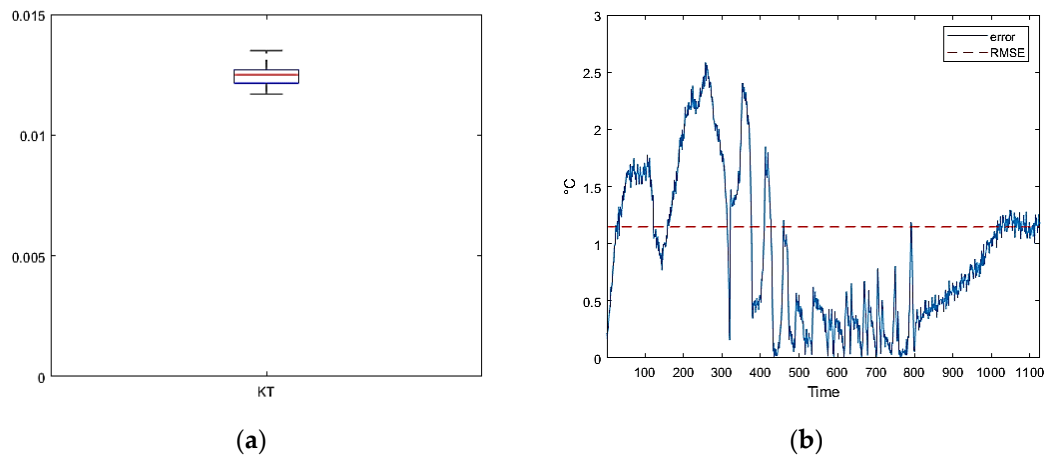
Figure 9 Test cycle 1: (a) Boxplot of experimental coefficient; (b) Absolute error trend.
