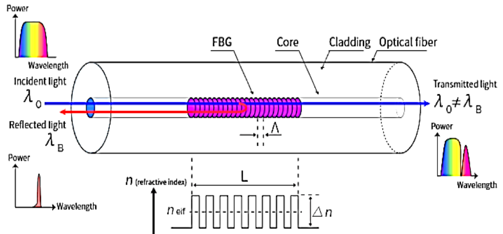
Figure 3 Scheme of FBG working principle [25]
