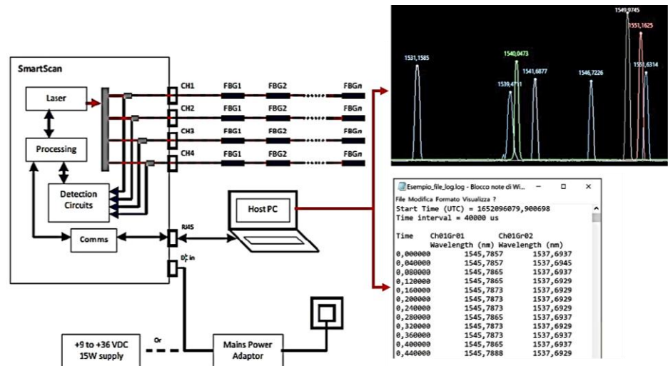
Figure 5 Scheme of data acquisition system.
