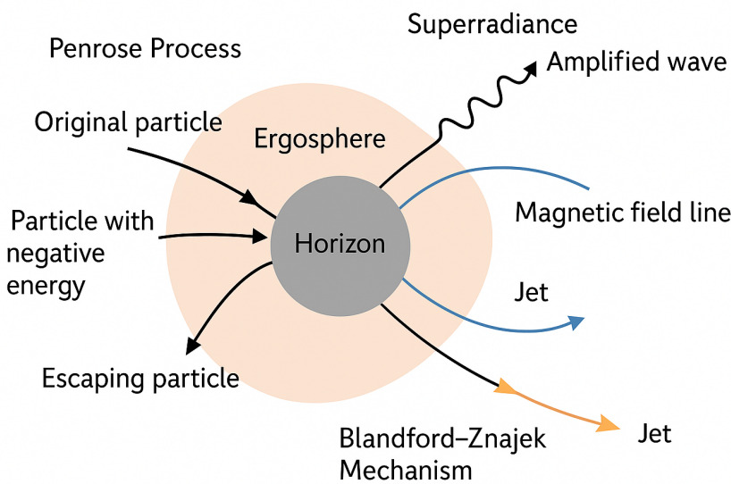
Figure 1. Penrose Process vs. Blandford-Znajek Mechanism.
