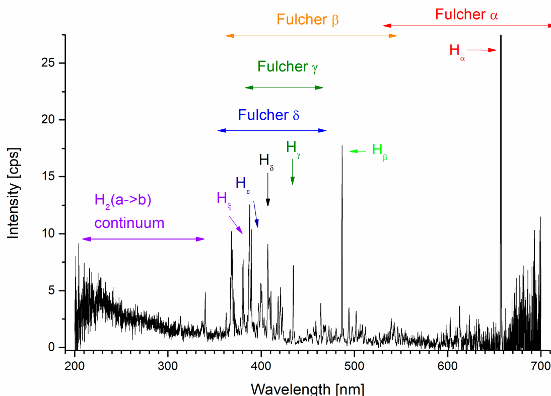
Figure 5. Electron induced fluorescence of the H 2 molecule—Balmer lines and Fulcher \alpha system. Measurements performed by Danko et al. [60].
