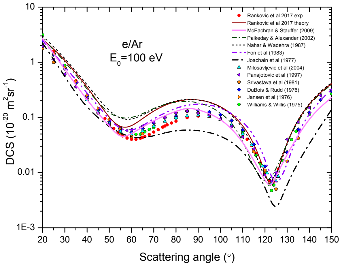
Figure 4. DCS for elastic electron scattering by argon atom at 100 eV impact energy. The data symbols used correspond to: (red circles) , Rankovic et al. [41] experiment; (dark red full line), Rankovic et al. [41] theory; (magenta solid line), McEachran and Stauffer [42]; (olive dash dot line), Paikeday and Alexander [43]; (dotted line), Nahar and Wadehra [44]; (violet dash dot dot line), Fon et al. [45]; (thin line), Staszewska et al. [46]; (cyan dash dot line), McCarthy et al. [47]; (dashed line), Joachain et al. [48]; (cyan up triangles), Milosavljević et al. [49]; (violet left triangle), Panajotović et al. [50]; (orange pentagons), Srivastava et al. [51]; (blue diamond), DuBois and Rudd [52]; (orange right triangles), Jansen et al. [53]; (asterisk), Vušković and Kurepa [54]; (green circles), Williams and Willis [55].
