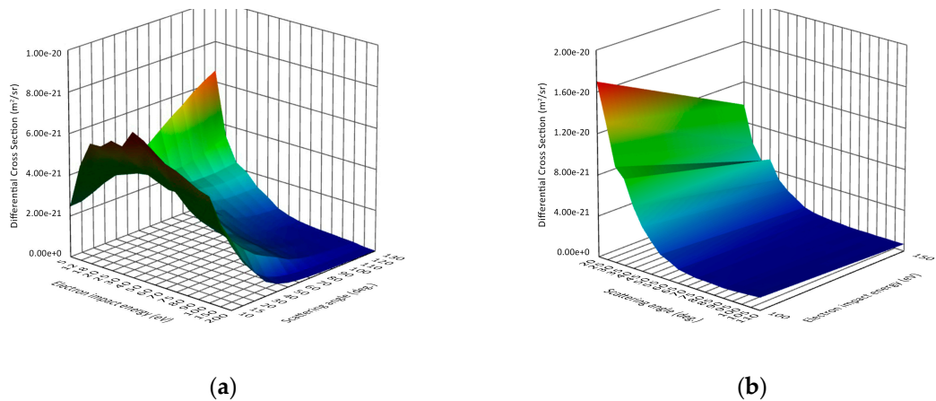
Figure 3. DCS surfaces as retrieved from RADAM database [23] for elastic electron scattering by: (a) He atom – data points are taken from ref. [24]; (b) Formamide molecule – data points are taken from ref. [25].
