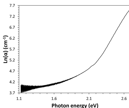
Figure 2. Plot of the absorption coefficient vs. photon energy for the calculation of the Urbach energy of Kapton.
