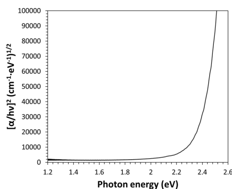
Figure 4. Cody plot for the Kapton-H type.
