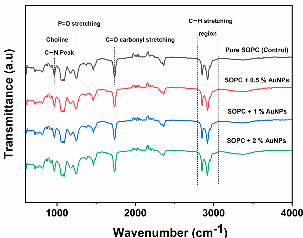
Figure 4. FTIR spectra of pure SOPC MLVs (control) and SOPC MLVs with 0.5, 1, and 2 w % of AuNPs.
