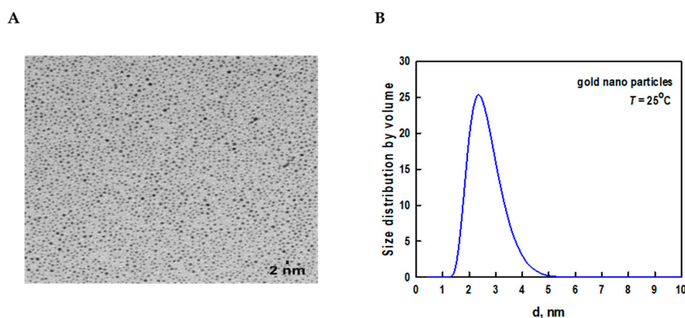
Figure 1. (A) TEM image of dodecanethiol-stabilized hydrophobic AuNPs. Scalebar corresponds to 2 nm. (B) Size distribution analysis of hydrophobic AuNPs by DLS.
