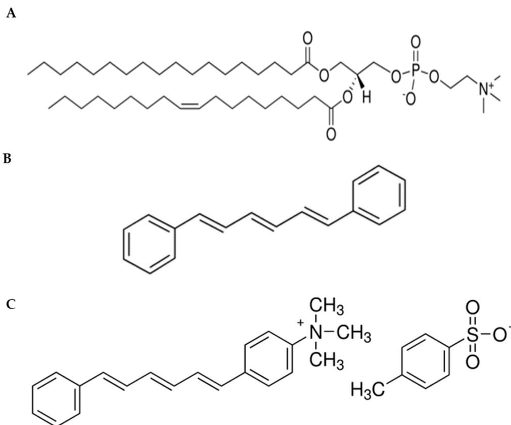
Figure 2. Chemical structure of (A) SOPC lipid, (B) 1, 6-diphenyl-1,3,5-hexatriene (DPH), and (C) 1-(4-trimethylammoniumphenyl)-6-phenyl-1,3,5-hexatriene (TMA-DPH) fluorescent probes.
