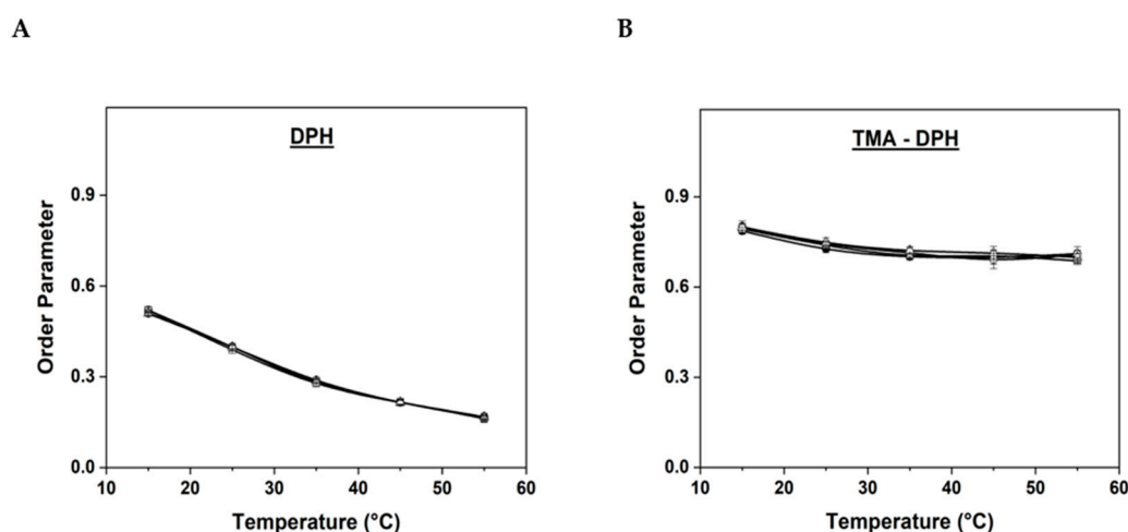
Figure 3. Lipid order parameter determined by (A) DPH and (B) TMA-DPH anisotropy measurements of SOPC MLVs with different concentrations of AuNPs. (● Pure SOPC MLVs taken as control; □ SOPC MLVs with 0.5 w % AuNPs; ○ SOPC MLVs with 1 w % AuNPs; △ SOPC MLVs with 2 w % AuNPs).
