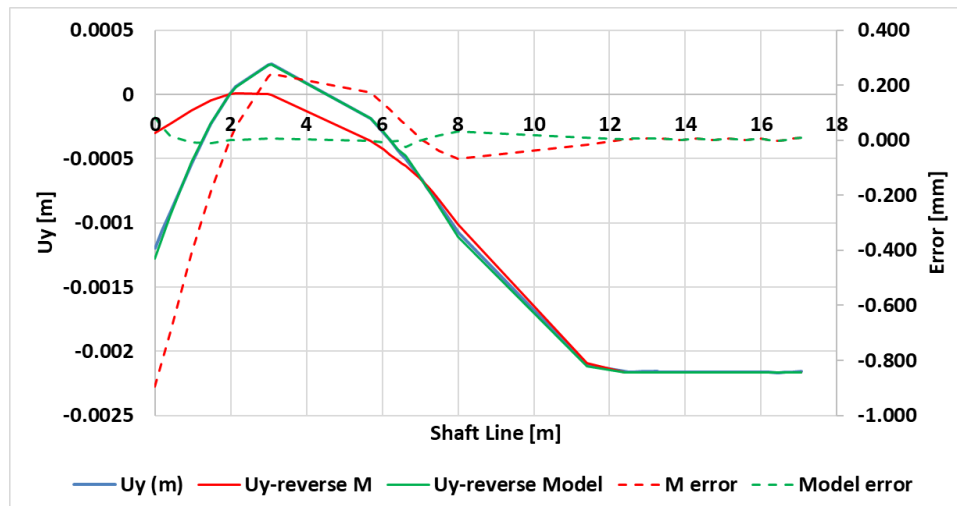
Figure 9. Scaled Model (M) and Equivalent Model (Model) error Comparison.
