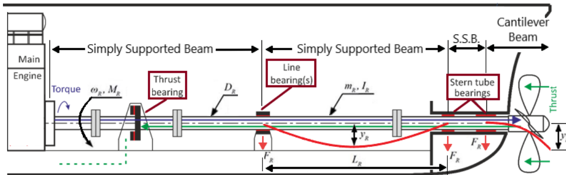
Figure 3. Key Scaling Parameters for Traditional Marine Shafting Systems.
