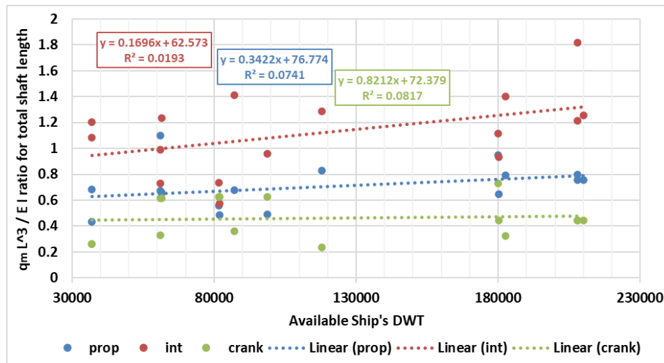
Figure 7. q_m L^3/EI ratio across the shaft-lines of ships with varying DWT.
