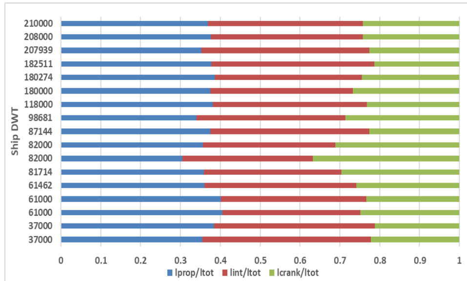
Figure 6. Various (Shaft Length / Total Shaft Length) Ratios for Bulk Carriers of different DWT.
