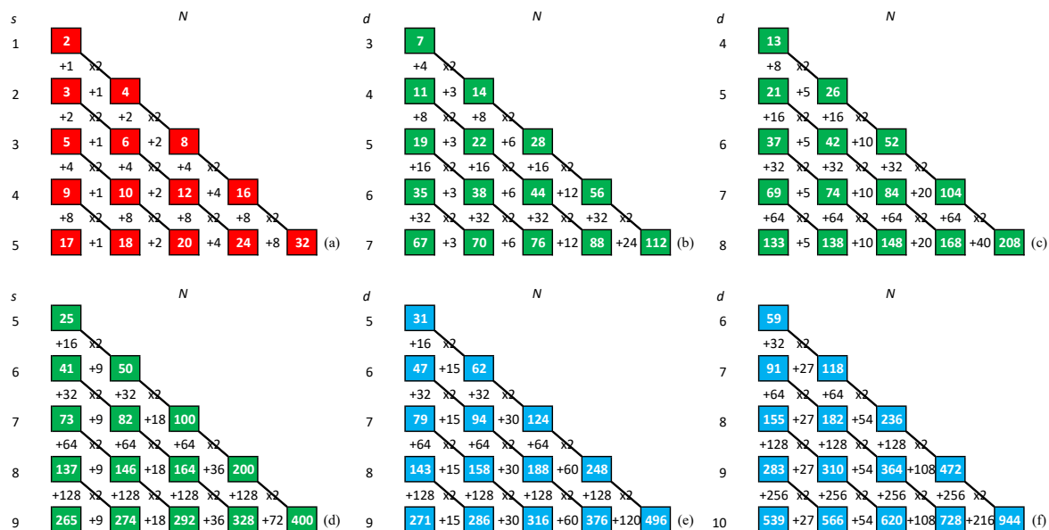
Figure 3. Lengths of all strings having the property of d_{\min}^{(\hat{N}_1)} = a_{\min}^{(\hat{N}_1)} = d_{\min}^{(\hat{N}_1)} = \hat{a}_{\min}^{(\hat{N}_1)} = s (a). Lengths \tilde{N}_3, \tilde{N}_5, \tilde{N}_9 of certain strings having the property of a_{\min}^{(\tilde{N}_*)} = d_{\min}^{(\tilde{N}_*)} + 1 (b-d). Lengths \tilde{N}_{15}, \tilde{N}_{27} of certain strings having the property of a_{\min}^{(\tilde{N}_*)} = d_{\min}^{(\tilde{N}_*)} + 2 (e,f)
