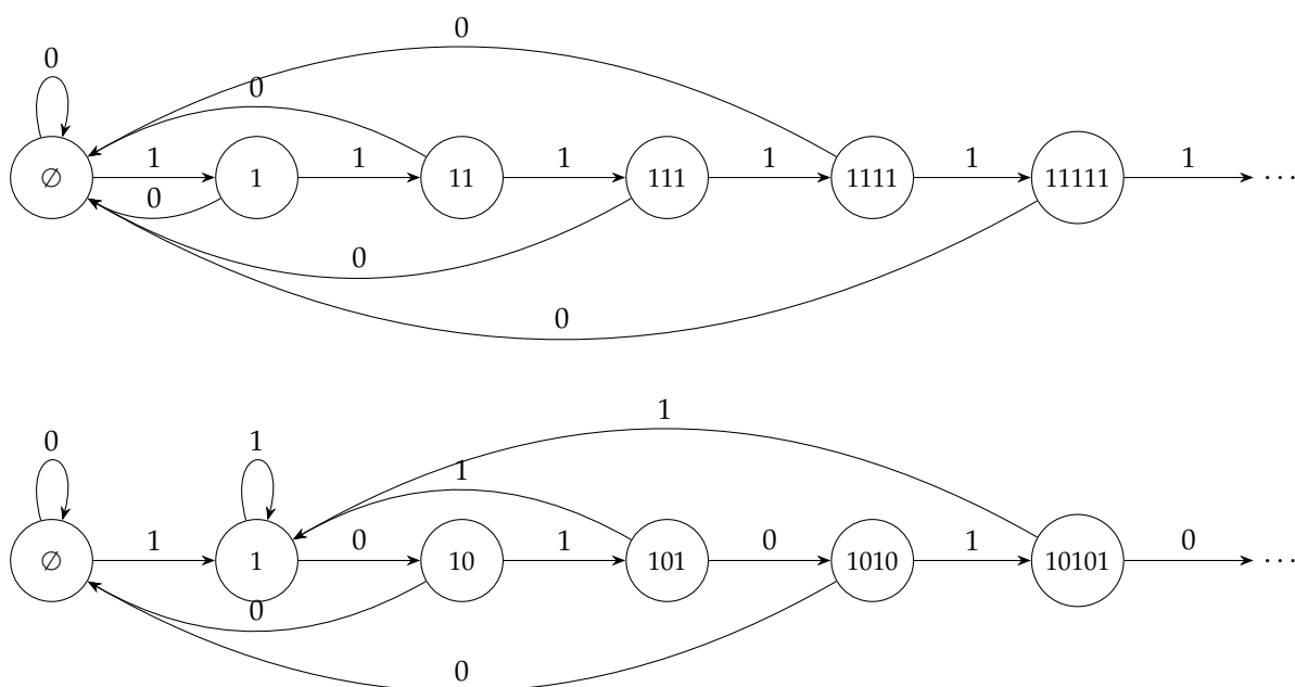
Figure 8. Markov chains illustrating different expected waiting times for strings [111\dots] and [1010\dots] .
