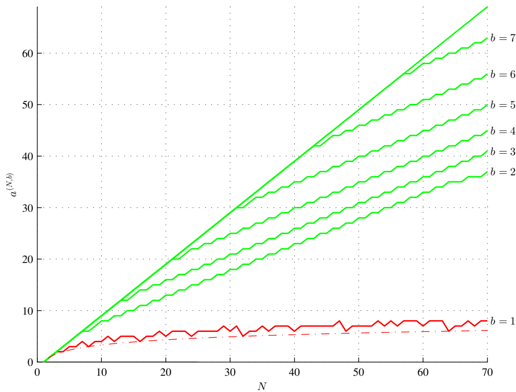
Figure 7. The minimum assembly index (OEIS A003313, red; \log_2(N) , red, dash-dot), and the maximum assembly index (green) for 1 \leq b \leq 7 and 0 < N \leq 70 showing the 2 nd threshold of quadruplet saturation 4b^4 for b = 2 at N = 64 .
