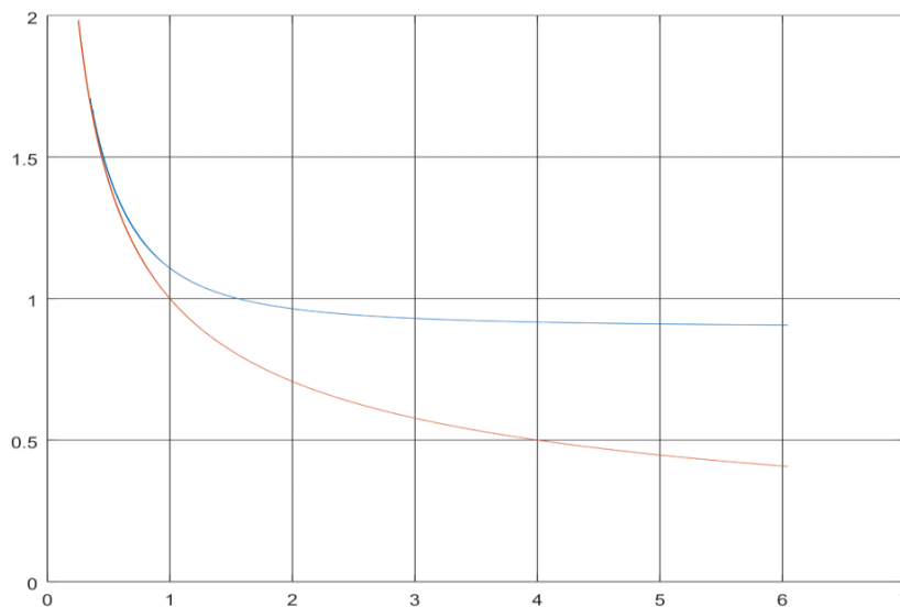
Figure 2. The rotation curve v(r) \equiv \omega(r)r|_{\lambda=1} obtained from (58) by setting \lambda = 1 (blue). The Newtonian curve for the same parameters (red).
