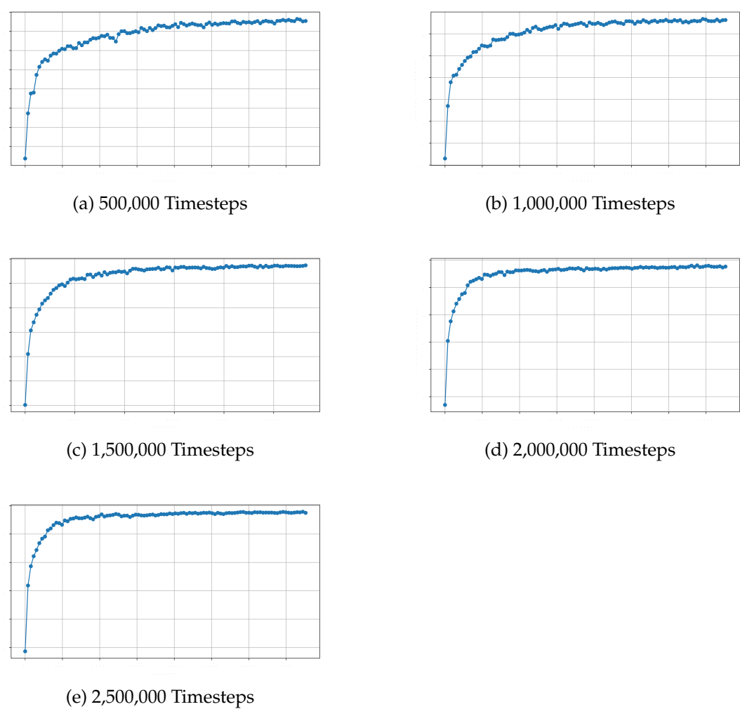
Figure 2. Normalized rewards per episode for the PPO agent at different training milestones (500K to 2.5M timesteps). The overall upward trend indicates effective policy learning and performance optimization over time.
