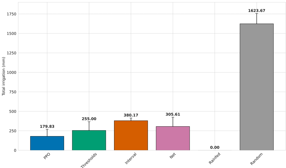
Figure 4. Total irrigation applied (mm) under different strategies. PPO and SMT demonstrate efficient water use, while random irrigation applies excessive amounts. Rainfed conditions rely solely on natural precipitation.
