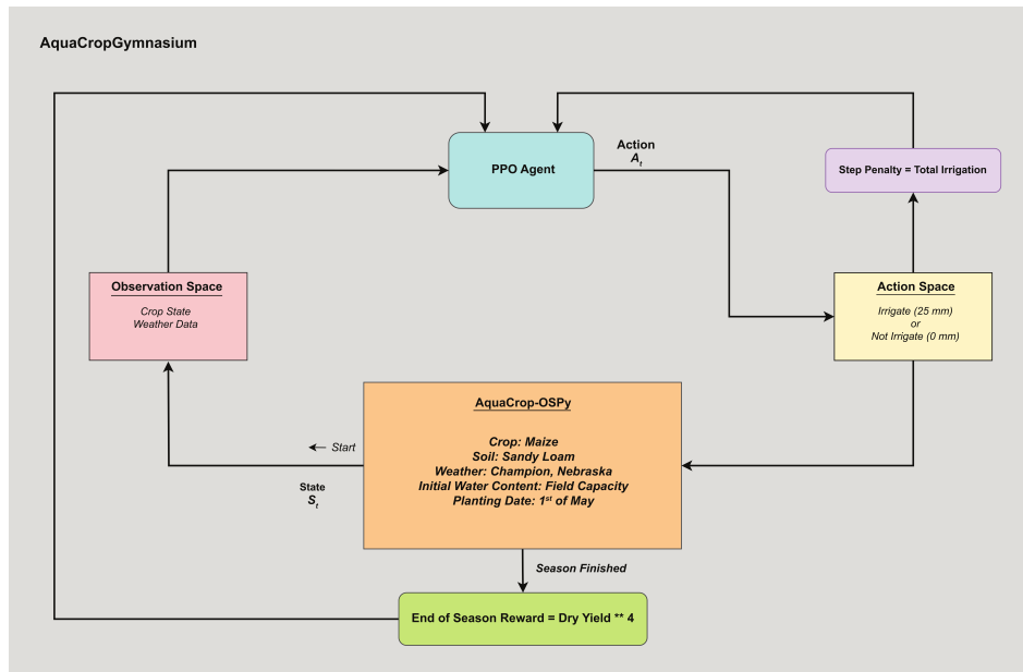
Figure 1. The interaction between the PPO agent and the AquaCrop-OSPy simulation within the AquaCropGymnasium framework.
