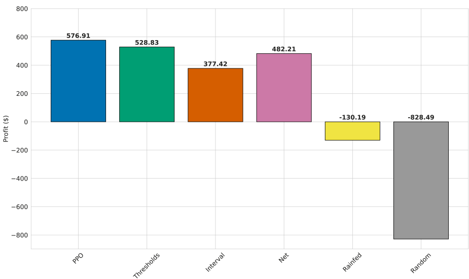
Figure 6. Profit per hectare ($/ha) under different irrigation strategies. PPO achieves the highest profitability, surpassing the optimized SMT strategy by approximately 9%. Random and rainfed approaches yield negative profits due to inefficient water use or reduced yields.
