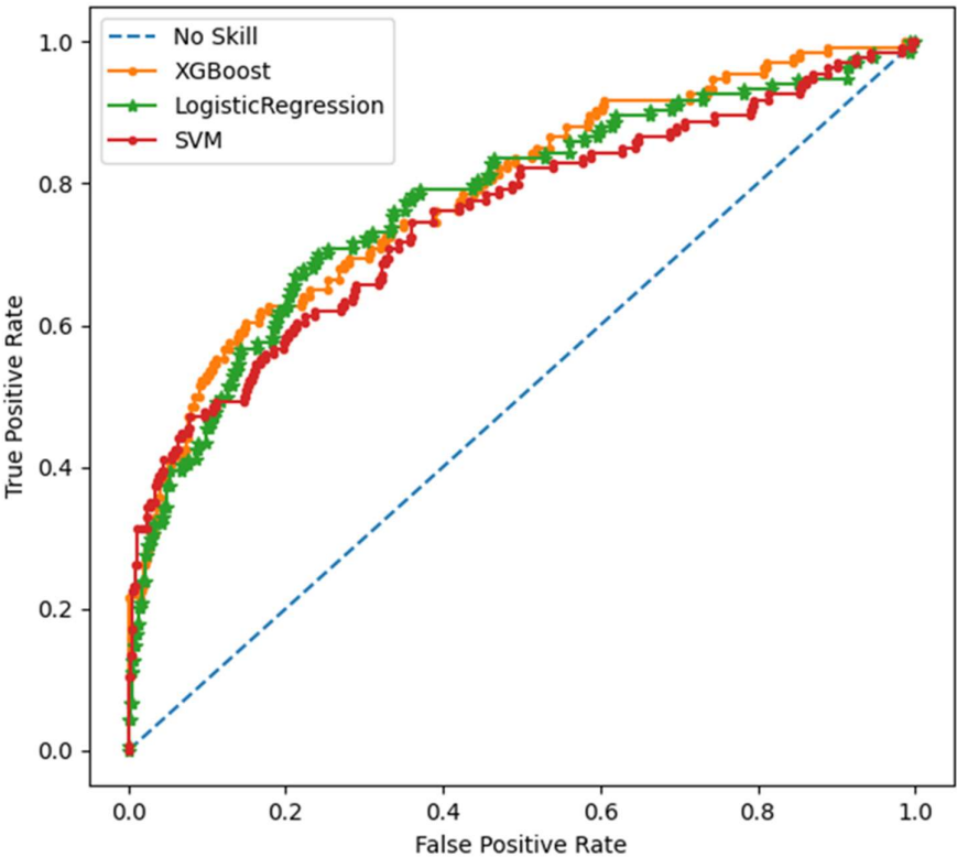
Figure 1. ROC-AUC curve for XGBoost, Logistic Regression, and SVM models.
