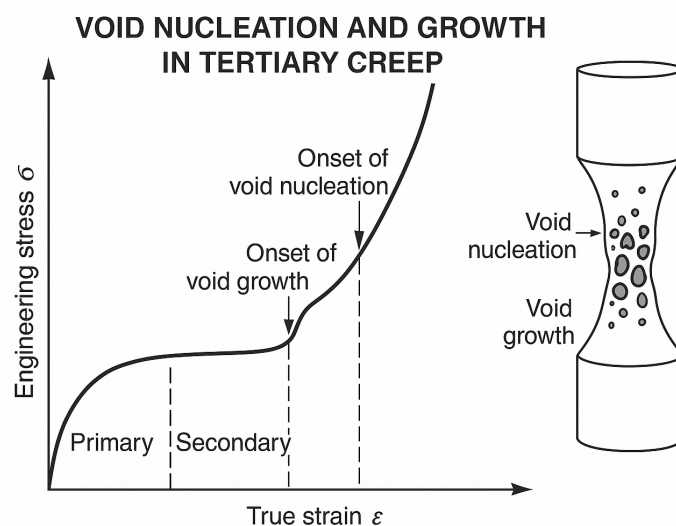
Figure 31. Void Nucleation and Growth in Tertiary Creep
