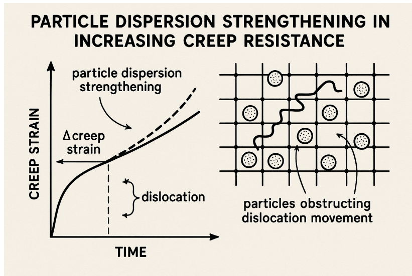
Figure 52. Particle Dispersion Strengthening in increasing Creep Resistance
