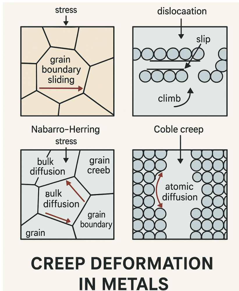
Figure 40. Creep Deformation in Metals
