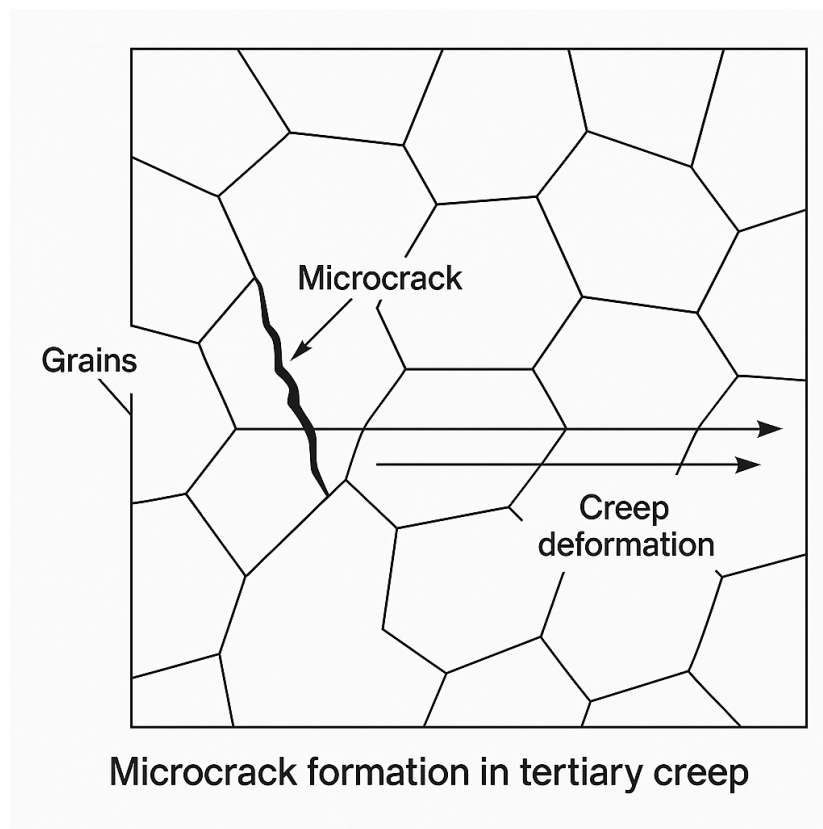
Figure 32. Microcrack Formation in Tertiary Creep
