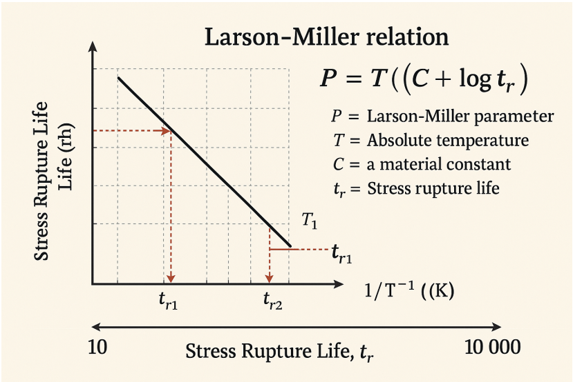
Figure 45. Larson Miller Relation
