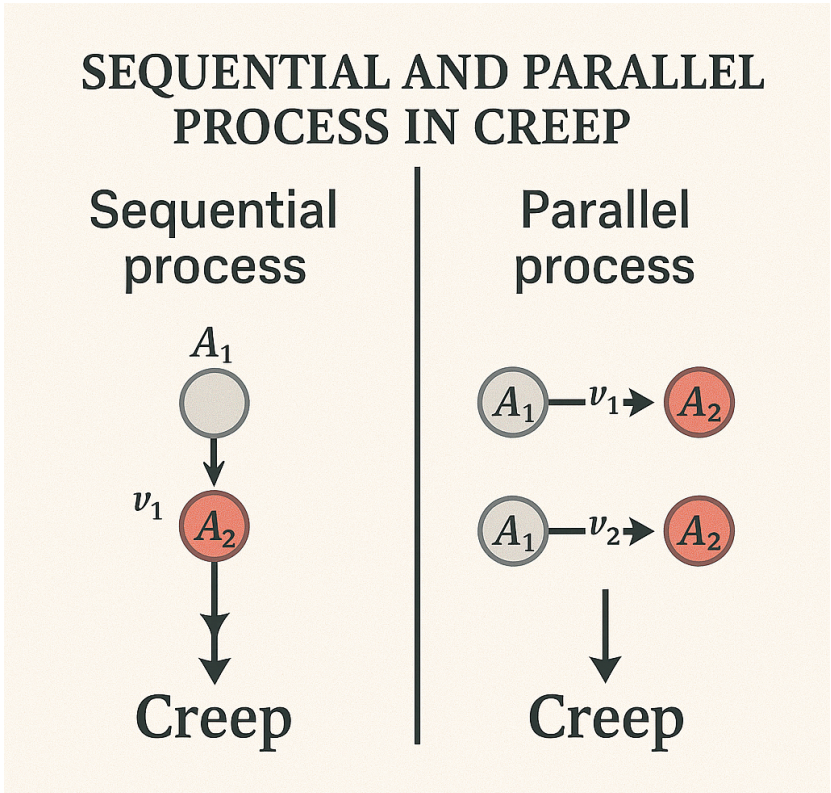
Figure 22. Sequential and Parallel Process in Creep
