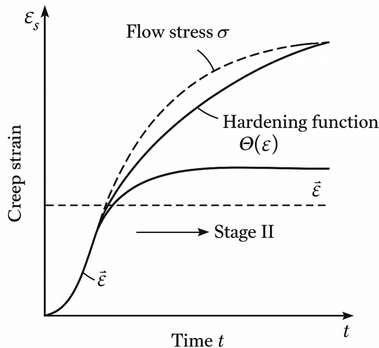
Figure 27. Work Hardening in Secondary Creep
