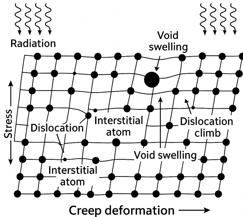
Figure 49. Effect of Irradiation in Creep Deformation
