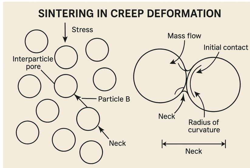
Figure 39. Sintering in Creep Deformation
