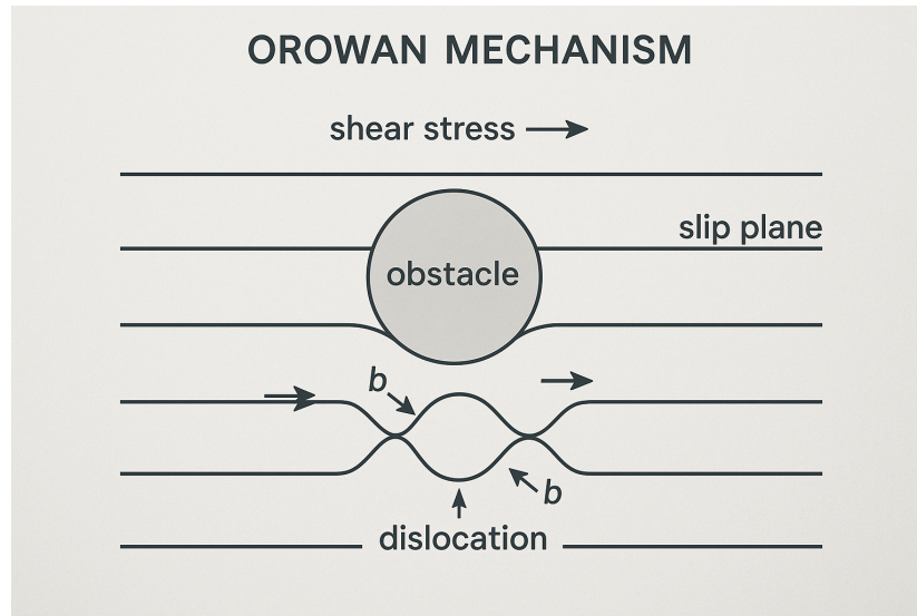
Figure 36. Orowan Mechanism
