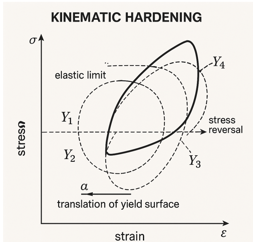
Figure 38. Kinematic Hardening Model
