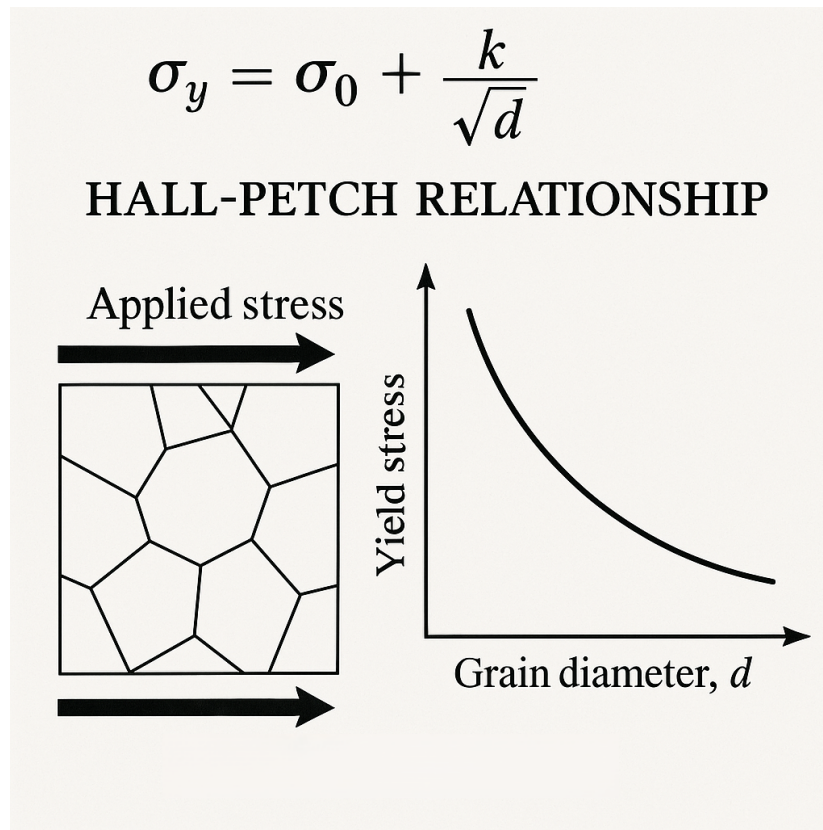
Figure 14. Hall-Petch Relationship
