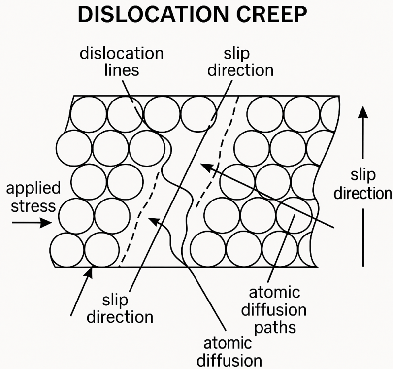
Figure 8. Dislocation Creep
