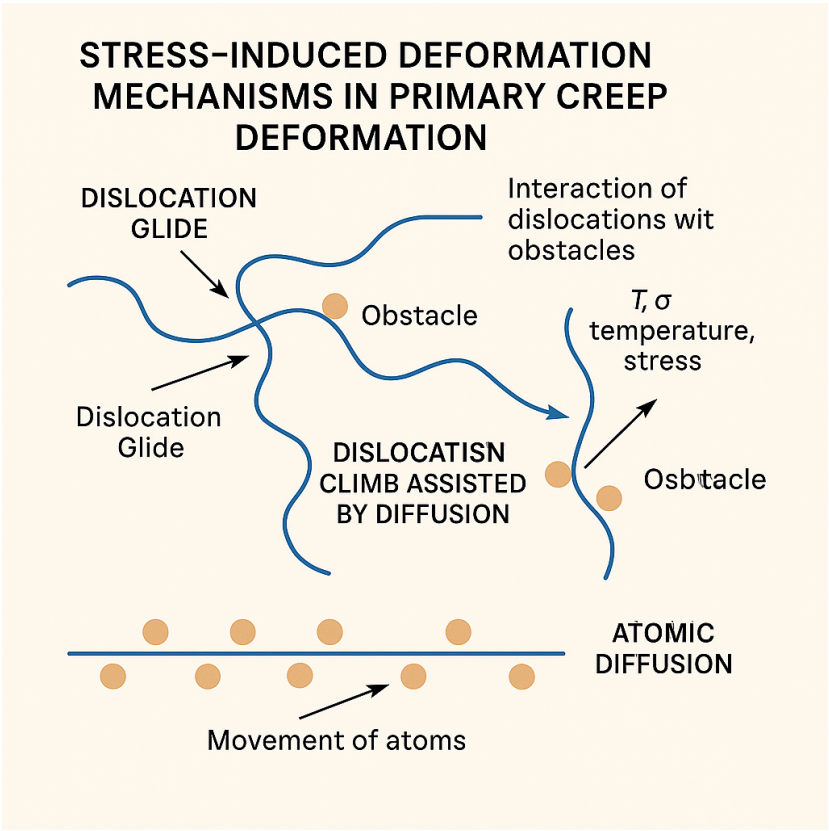
Figure 24. Stress-induced Deformation in Primary Creep
