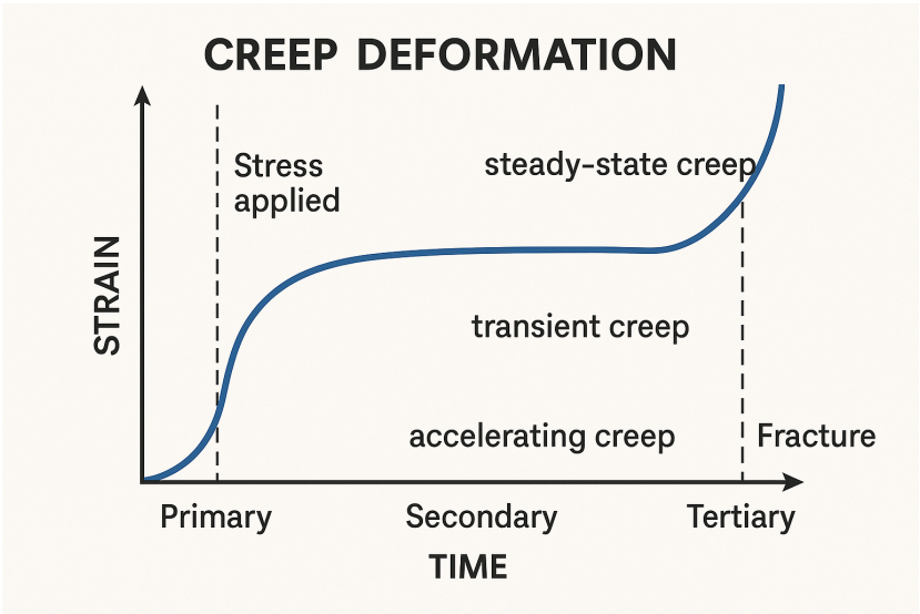
Figure 23. 3 Stages of Creep
