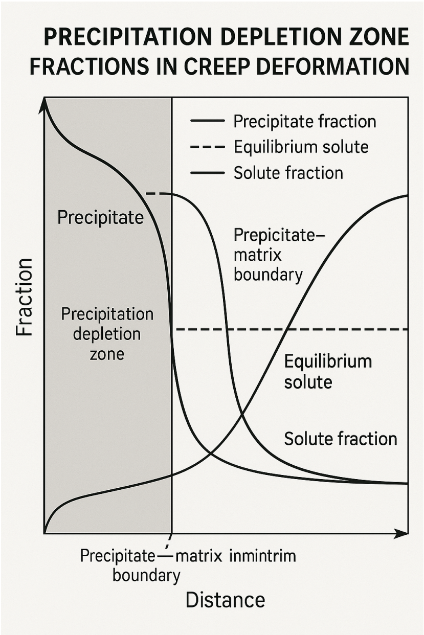
Figure 15. Precipitation Depletion Zone
