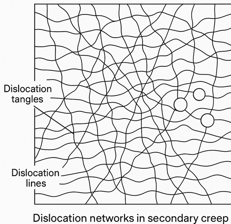
Figure 29. Dislocation Networks in Secondary Creep
