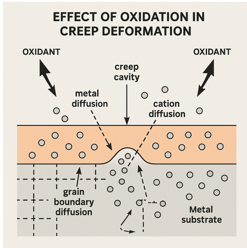
Figure 48. Effect of Oxidation in Creep Deformation
