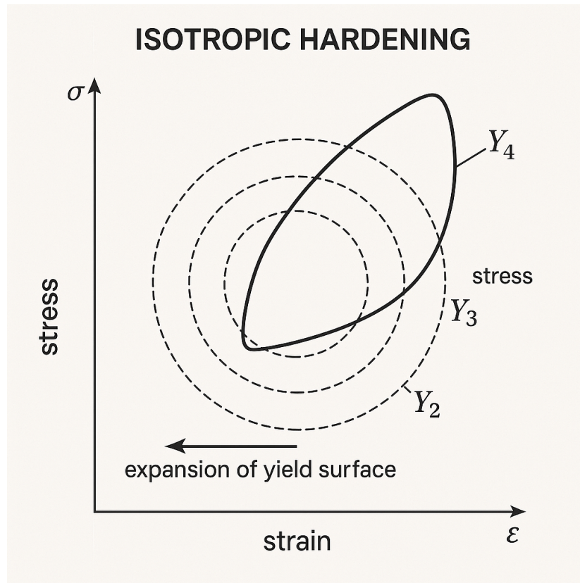
Figure 37. Isotropic Hardening Model
