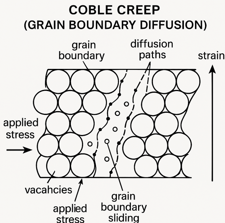
Figure 7. Coble Creep (Grain Boundary Diffusion)
