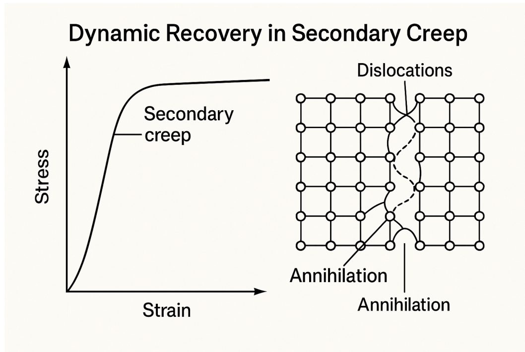
Figure 28. Dynamic Recovery in Secondary Creep
