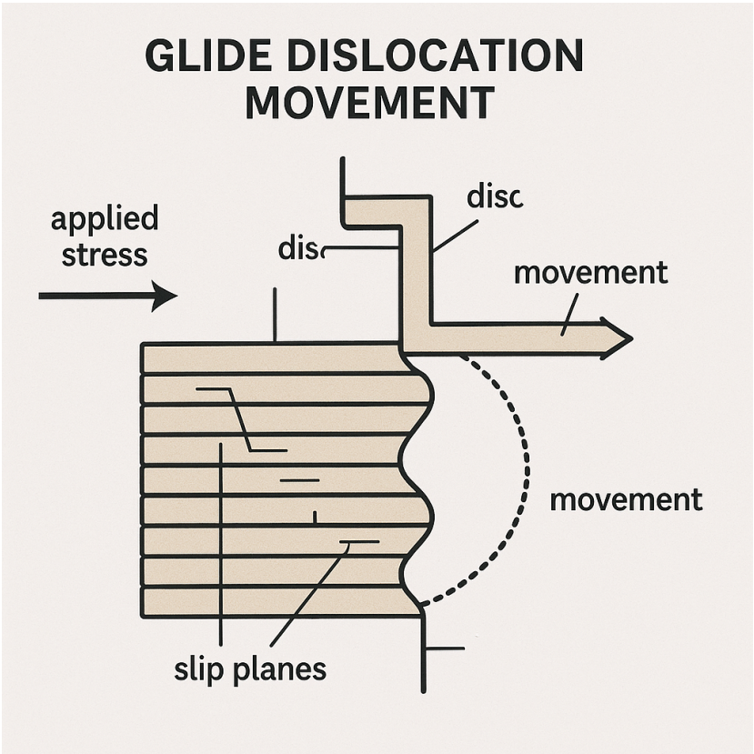
Figure 10. Glide Dislocation Movement
