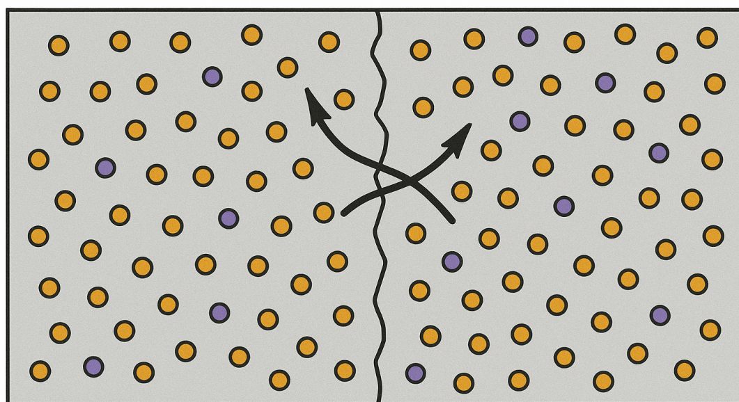
Figure 4. Vacancy diffusion at Grain Boundaries in creep
