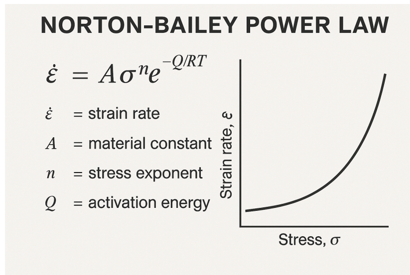
Figure 35. Norton-Bailey Law
