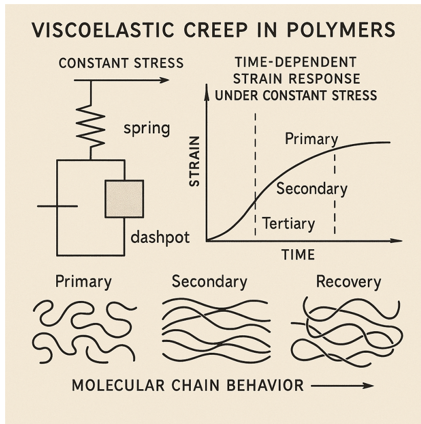
Figure 41. Viscoelastic Creep in Polymers
