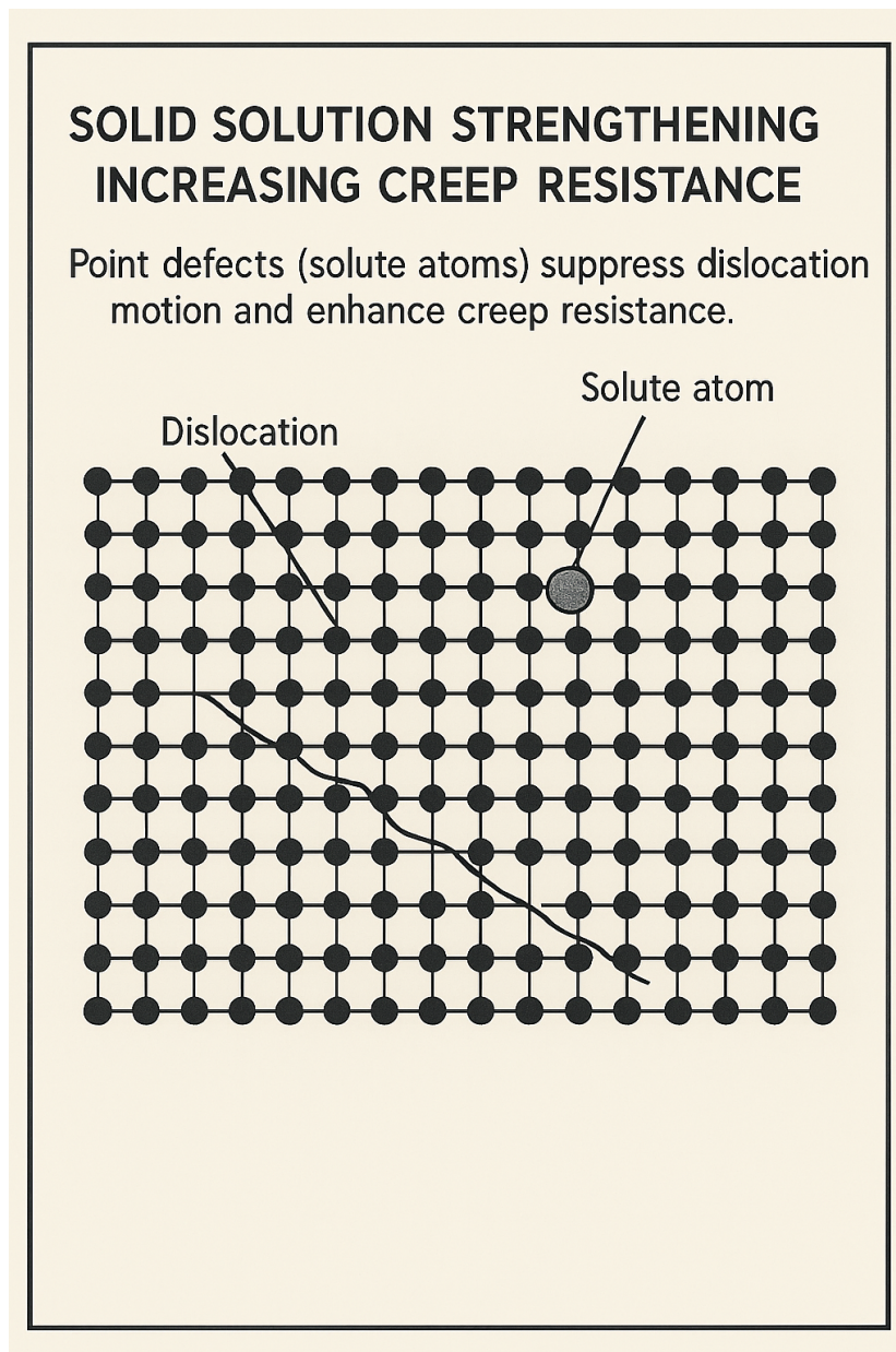
Figure 50. Solid solution strengthening in Creep Resistance
