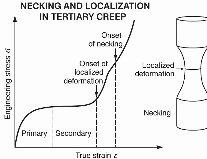
Figure 34. Necking and Localization in Tertiary Creep
