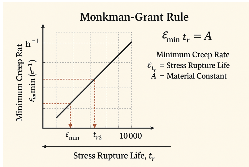
Figure 46. Monkman Grant Rule
