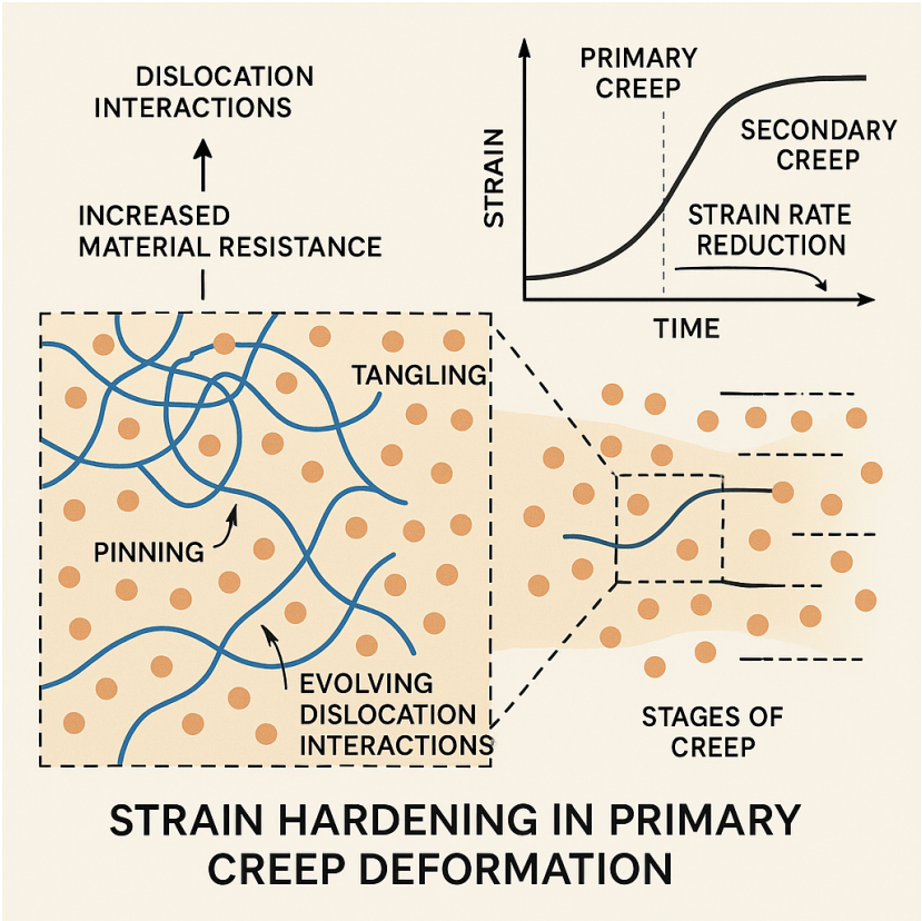
Figure 25. Strain Hardening in Primary Creep
