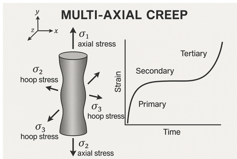
Figure 47. Multi Axial Creep
