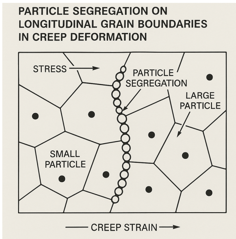
Figure 16. Particle Segregation on Longitudinal Grain Boundaries
