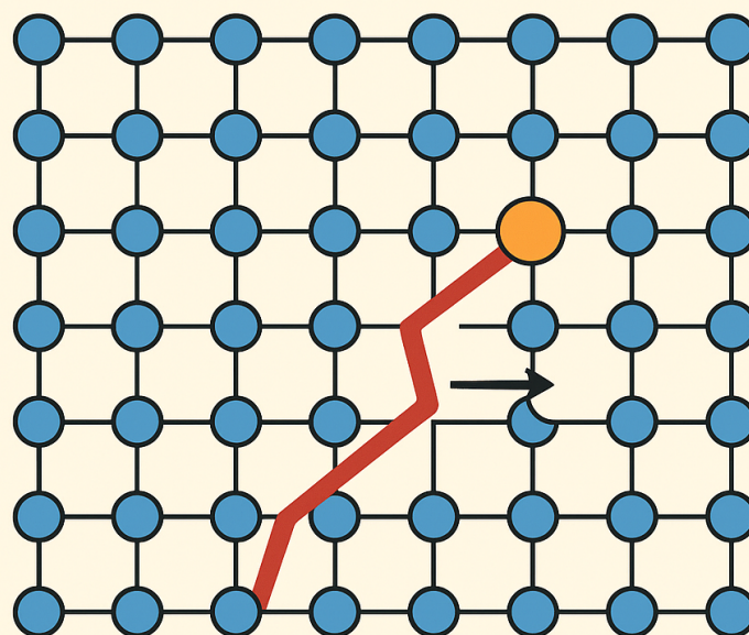
Figure 2. Dislocation-assisted diffusion
