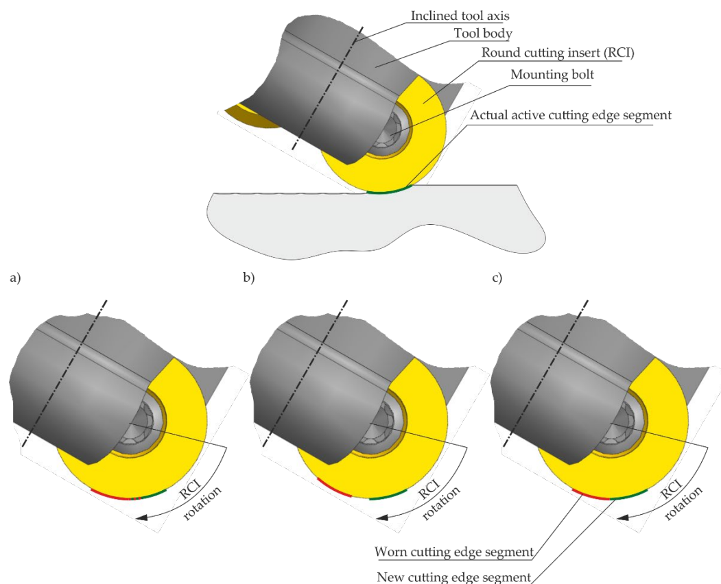
Figure 2. Possible cases of the round cutting insert rotation: (a) overlapping of a new segment with a worn segment – wrong; (b) too large a gap between segments – wrong; (c) segments adjacent to each other – correct.
