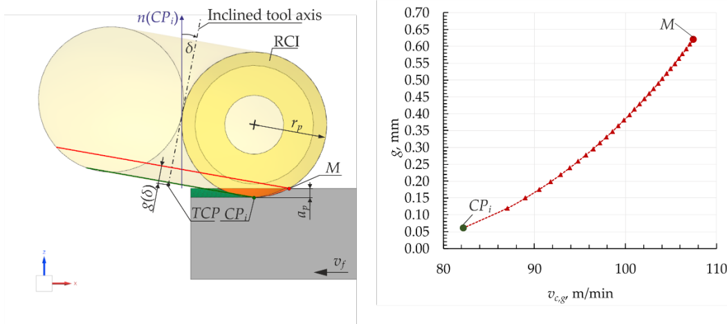
Figure 7. Cutting speed variation along the tool axis for torus milling cutter. (Tool diameter: 16 mm, round cutting insert radius: 4 mm, spindle speed: 2786 rpm, inclination angle: 10^\circ ).
