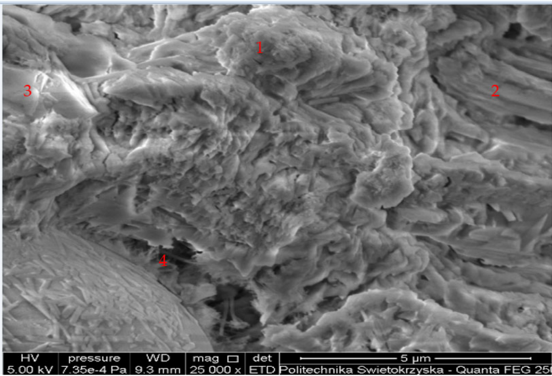
Figure 9. Microstructure area of mortar SW with analysed points.
