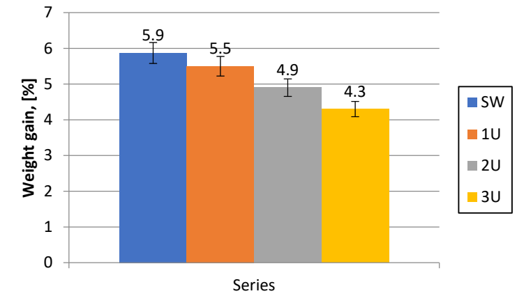
Figure 6. Weight gain in the mortar absorbency test, [%].
