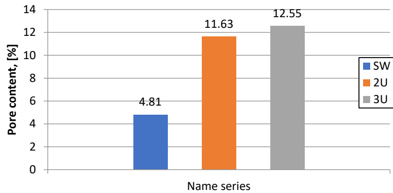
Figure 7. Percentage of pores in the mortar cross-sections tested.
