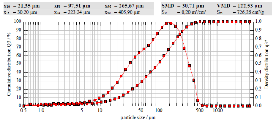
Figure 2. Grain size of the recycled product.
