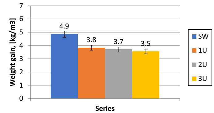
Figure 5. Weight gain in the capillary rise test of mortars, [kg/m 2 ].
