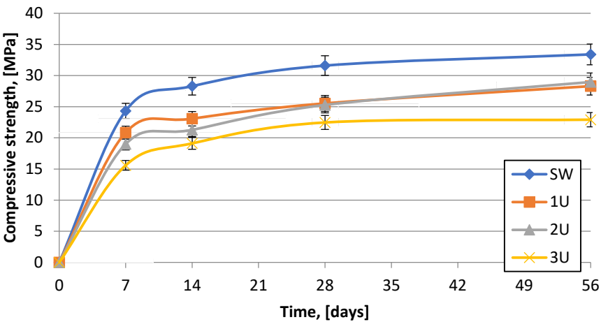
Figure 3. Average increase in compressive strength of the tested series.
