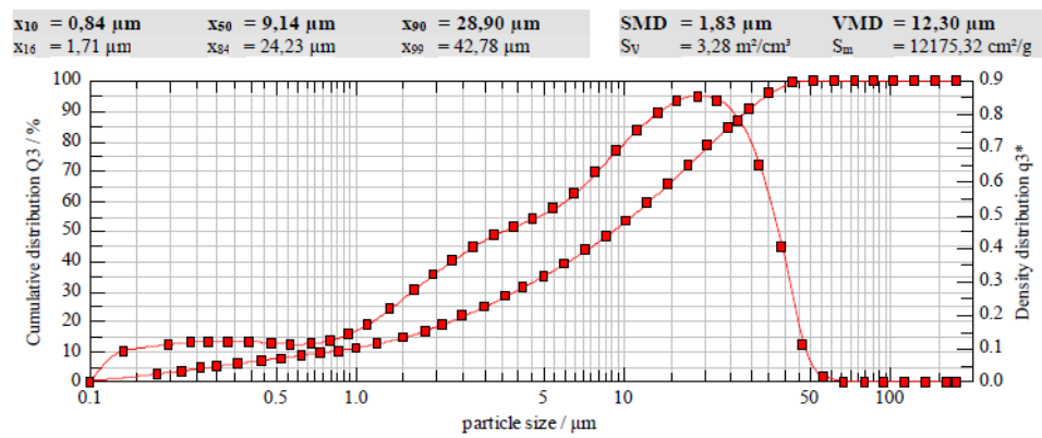
Figure 1. Grain size of CEM I 42.5R cement.
