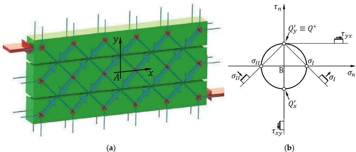
Figure 25. Straps activated by a seismic load: (a) In the plane of the wall; (b) As explained by the stress analysis performed in the Mohr plane for the infinitesimal neighborhood of point A .
