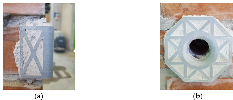
Figure 11. The 3D printed elements applied with mortar on the specimens: (a) Rounded angles; (b) Funnel plates.
