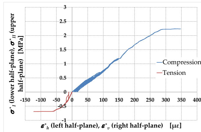
Figure 28. Uniaxial stress/strain relationships obtained for Specimen M1-90.
