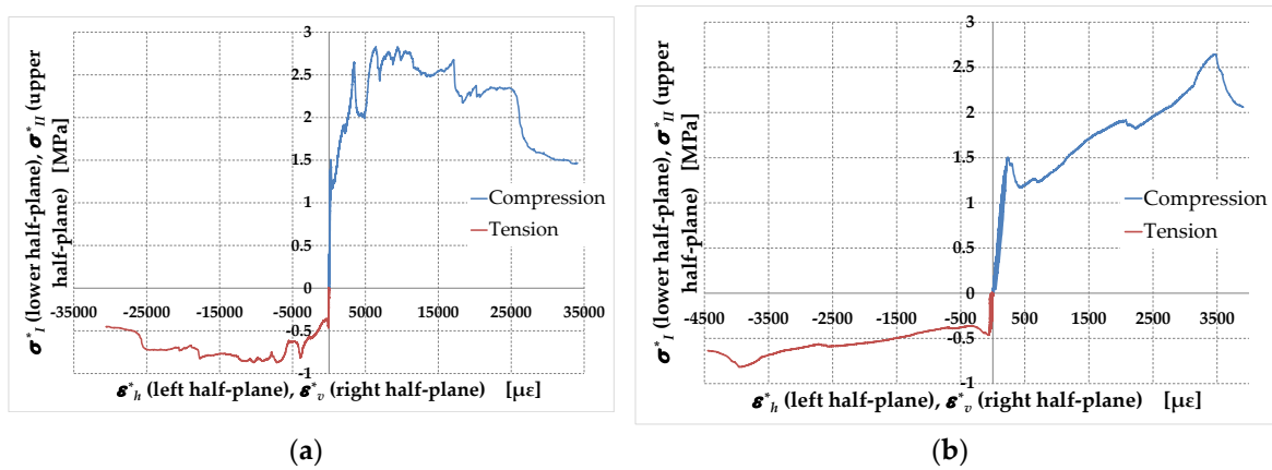
Figure 30. Uniaxial stress/strain relationships of Specimen M2-45: (a) Until the end of the loading test; (b) Truncated, to highlight the difference in slope at the origin in the two quadrants.
