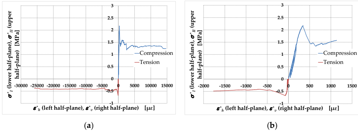
Figure 29. Uniaxial stress/strain relationships of Specimen M1-45: (a) Until the end of the loading test; (b) Truncated, to highlight the difference in slope at the origin in the two quadrants.
