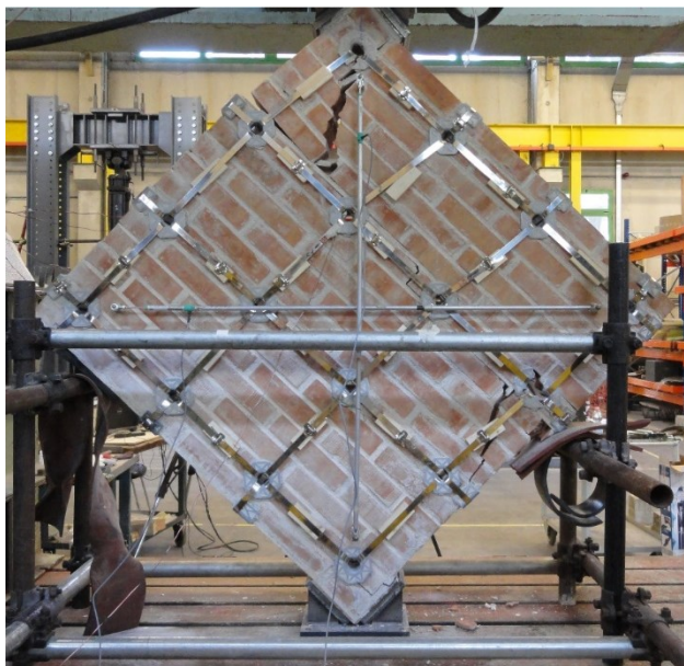
Figure 18. Failure mode of Specimen M1-90.
