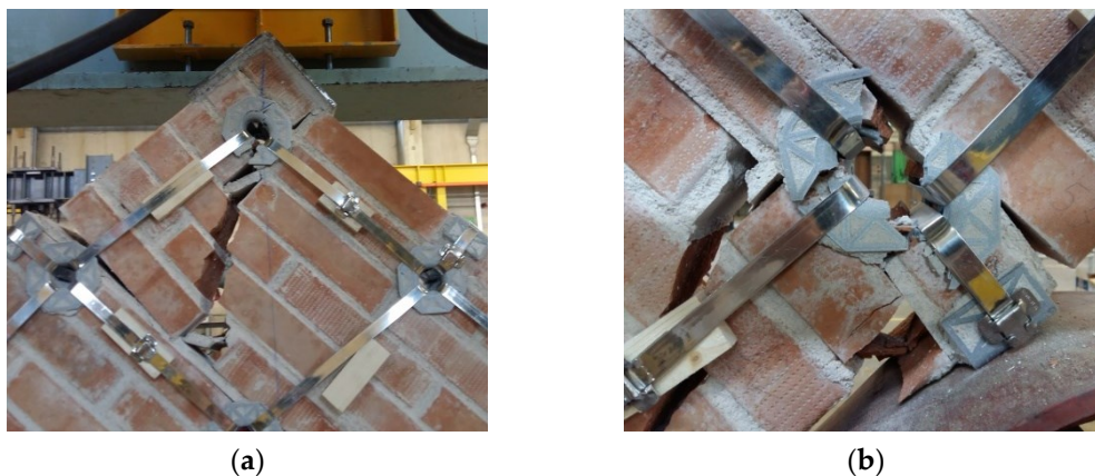
Figure 19. Details of the broken funnel plates: (a) Funnel plate in the upper left corner of the mechanism; (b) Funnel plate in the lower right corner of the mechanism.
