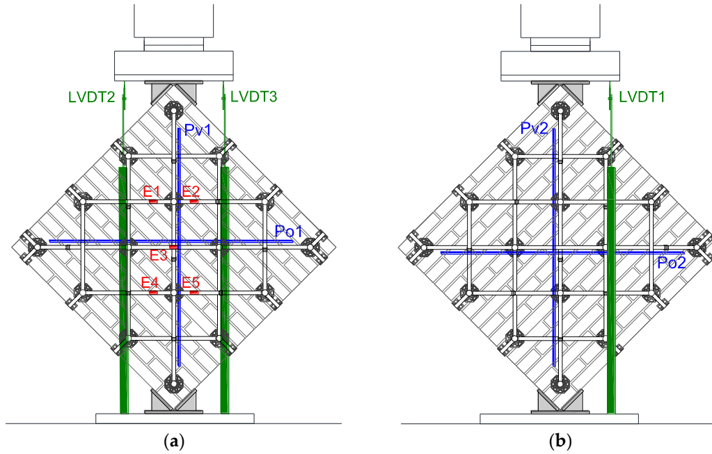
Figure 15. Instrumentation of Specimen M1-45: (a) Front view; (b) Back view.
