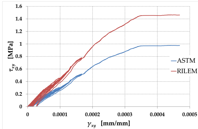
Figure 22. Shear stress/shear strain curves for specimen M1-90, according to ASTM and RILEM interpretations of the diagonal compression test.
