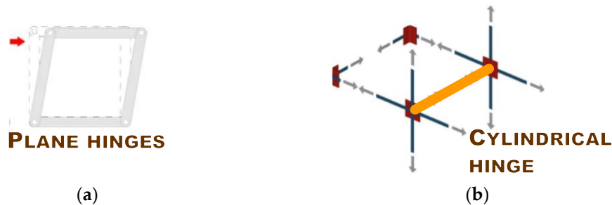
Figure 2. Lability of the CAM® System with a rectangular arrangement: (a) In the wall plane; (b) In the wall thickness.
