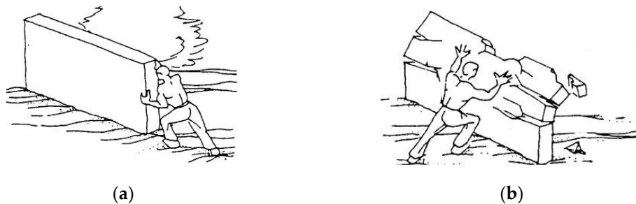
Figure 1. How a seismic event loads a wall: (a) In the plane of the wall (shear loading in the midplane); (b) Along the direction perpendicular to the plane of the wall (out-of-plane loading).
