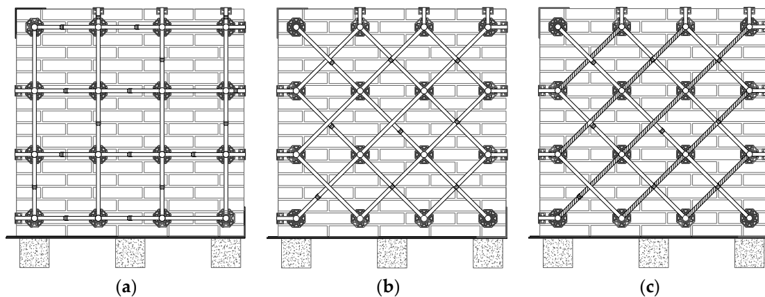
Figure 5. The three specimens of the experimental program: (a) Specimen M1-90; (b) Specimen M1-45 and (c) Specimen M2-45.
