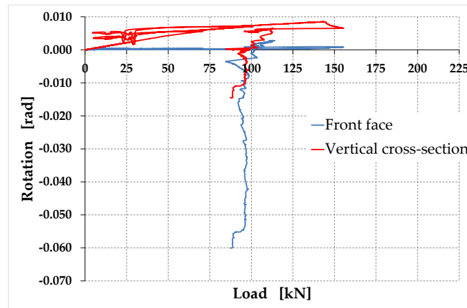
Figure 16. Rotations undergone by Specimen M1-45: positive values indicate anti-clockwise rotations on the front face and on the vertical cross-section, seen from the left side.
