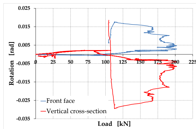
Figure 17. Rotations undergone by Specimen M2-45: positive values indicate anti-clockwise rotations on the front face and on the vertical cross-section, seen from the left side.
