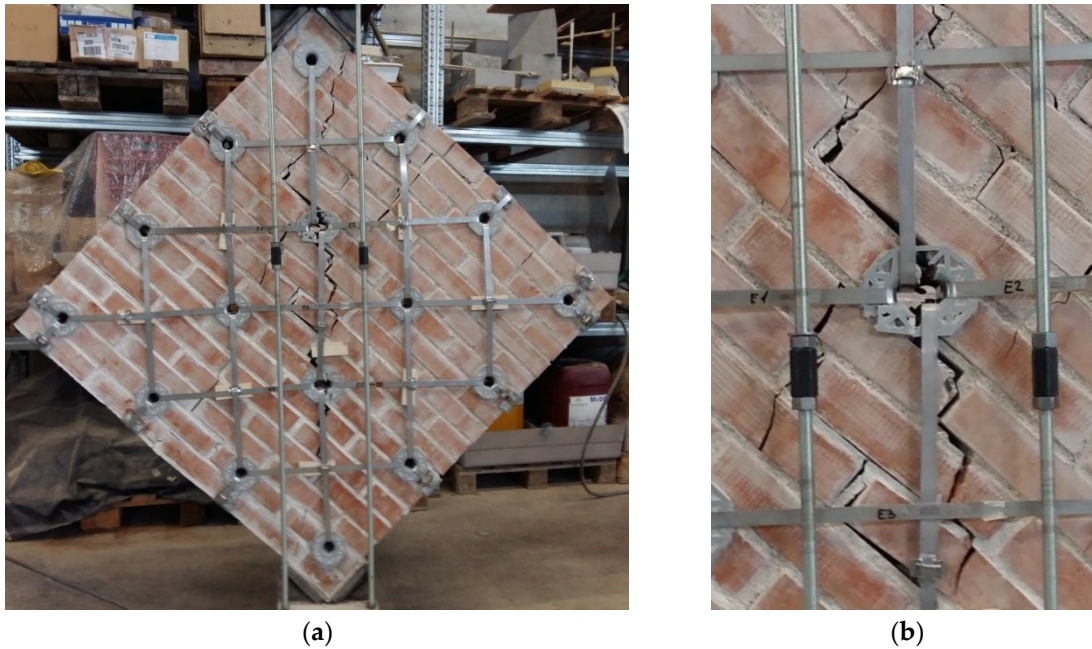
Figure 20. Failure mode of Specimen M1-45: (a) Appearance of the specimen after its removal from the testing machine; (b) Detail of the crack along the compressed diagonal.
