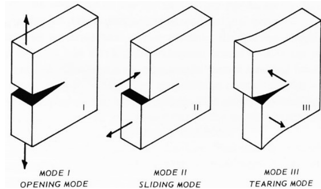
Figure 31. The three modes of crack propagation in fracture mechanics [73].
