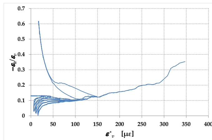
Figure 32. Apparent Poisson's ratio versus strain \varepsilon_v^* ; specimen M1-90.
