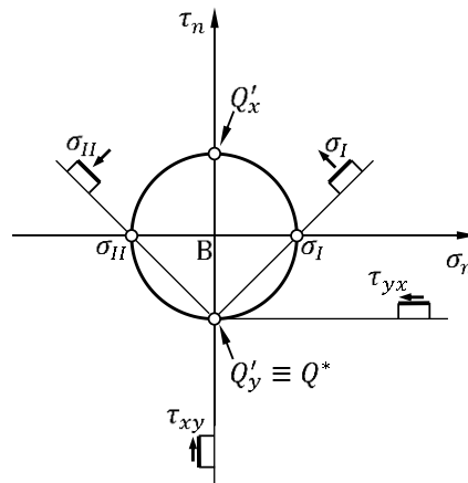
Figure 26. Stress analysis performed in the Mohr plane for the infinitesimal neighborhood of point A when the direction of the seismic load reverses.
