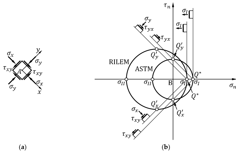
Figure A4. The Pole Method for the identification of the stress components in the infinitesimal neighborhood of point A : (a) Reference frame of Figure A1 for the association between planes with unit normal vector \mathbf{n} and points Q'_n of the Mohr plane; (b) Application of the method in the ASTM and RILEM interpretations of the diagonal compression test.
