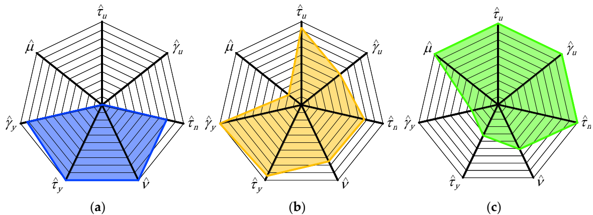
Figure 35. Radar diagrams of: (a) specimen M1-90; (b) specimen M1-45 and (c) specimen M2-45.
