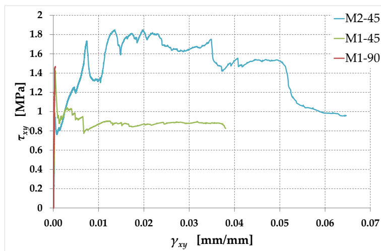
Figure 23. Shear stress/shear strain curves for the tested specimens.
