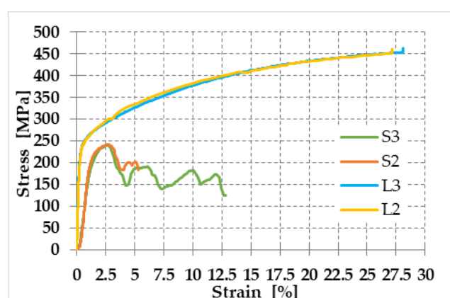
Figure 9. Stress/strain diagrams of the four specimens for the mechanical characterization of the straps.
