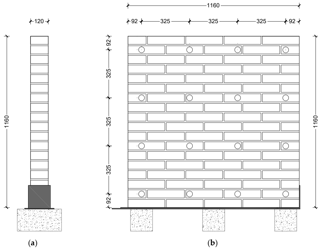
Figure 4. Geometric characteristics of the single-headed masonry specimens (all dimensions in mm): (a) Side view; (b) Front view.
