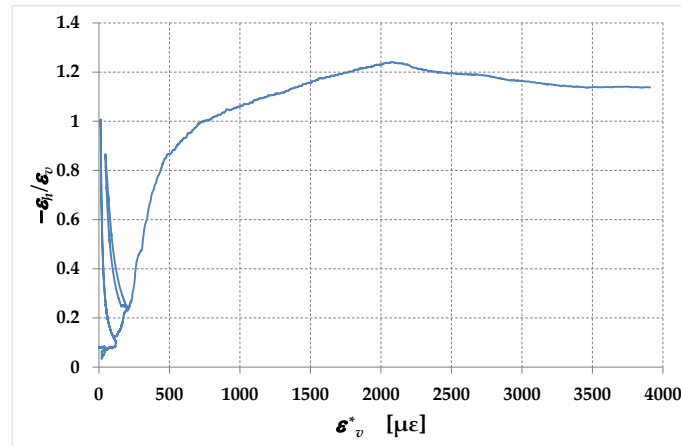
Figure 34. Apparent Poisson's ratio versus strain \varepsilon_v^* : specimen M2-45.
