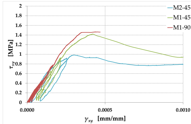
Figure 24. Detail of Figure 23 for shear strain values between 0 and 0.001.
