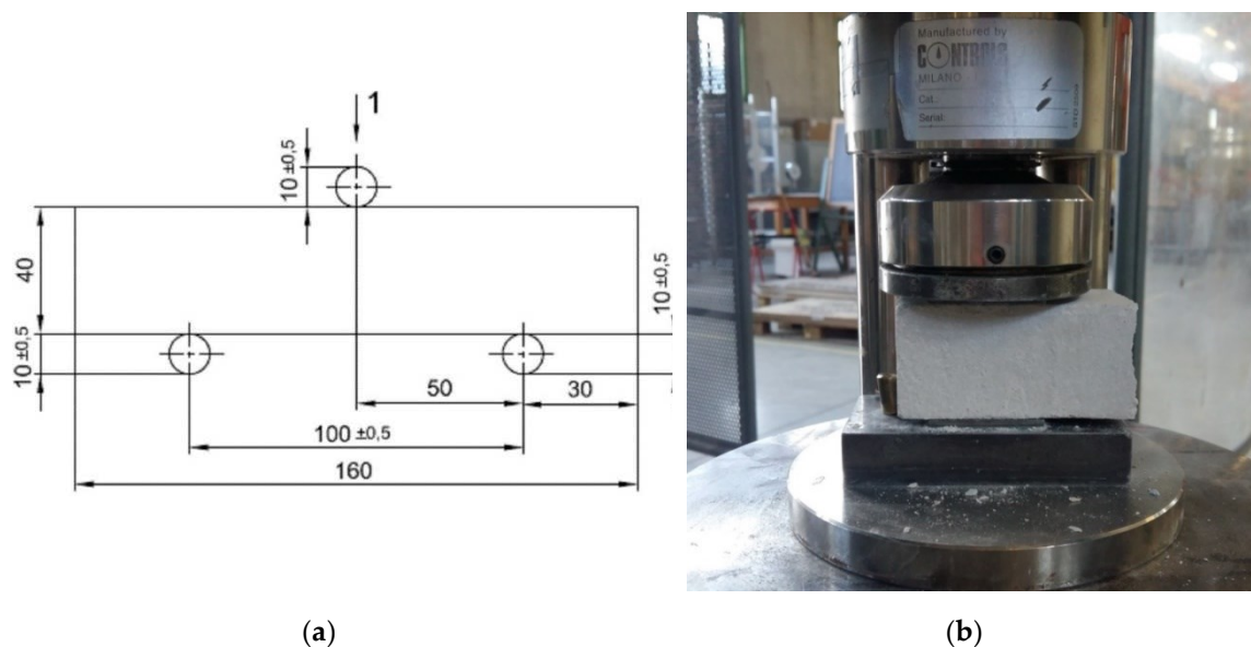
Figure 7. Mechanical characterization of the mortar according to the UNI EN 1015-11:2019 standard: (a) Set-up of the three-point bending flexural test (dimensions in mm); (b) Uniaxial compression test on one of the two half-prisms originating from the flexural test.
