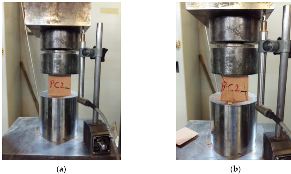
Figure 6. Appearance of the specimen PC2: (a) Before the compression test and (b) After the compression test.
