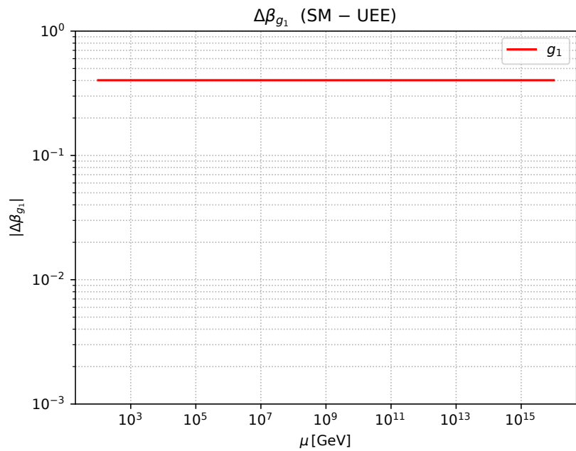
Figure A2. Plot of \Delta\beta_{g_1} only.
