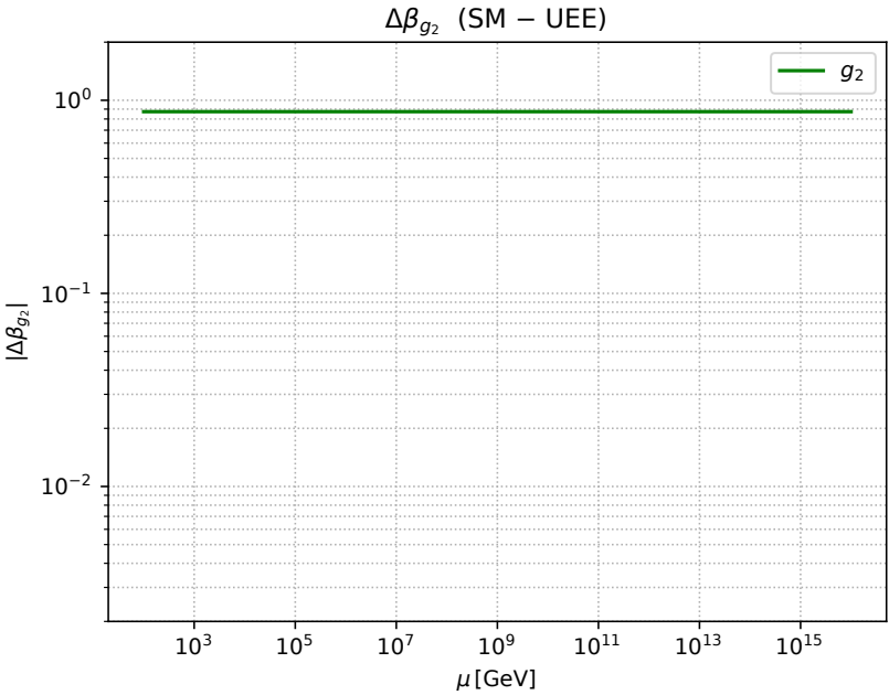
Figure A3. Plot of \Delta\beta_{g_2} only.
