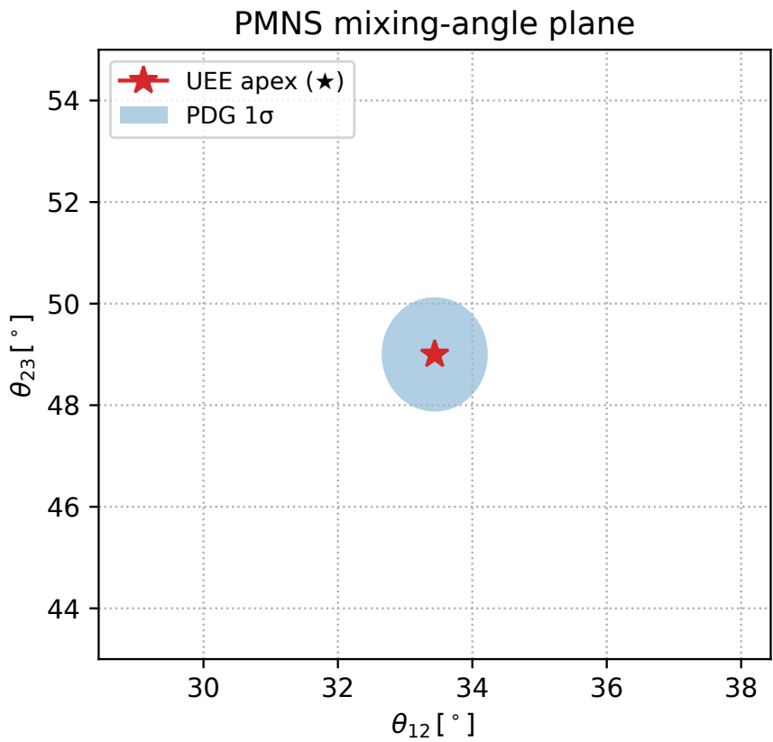
Figure A8. PMNS mixing-angle plane. ★ = UEE prediction, blue ellipse = PDG 2024 1σ.
