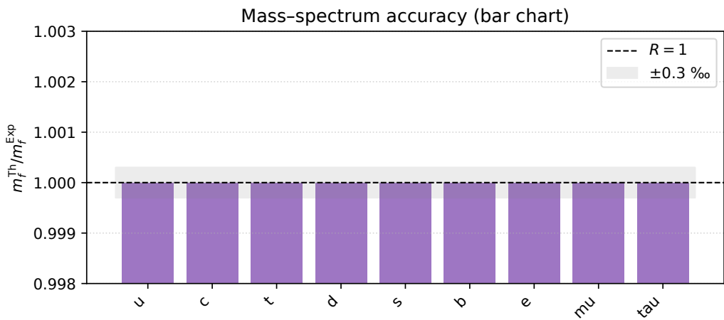
Figure A13. Mass-ratio bar chart: grey band = \pm 0.3 \text{ ‰} , dashed line = exact match.
