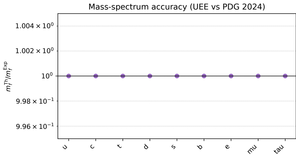
Figure A6. Mass ratios m_f^{\text{Th}}/m_f^{\text{Exp}} (logarithmic).
