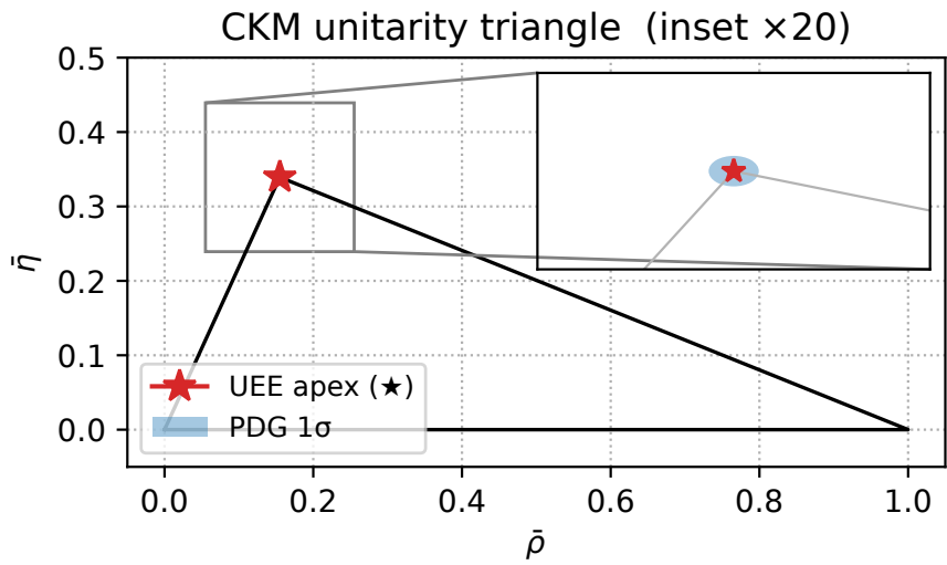
Figure A7. CKM unitarity triangle. ★ = UEE predicted vertex, blue ellipse = PDG 2024 1σ.
