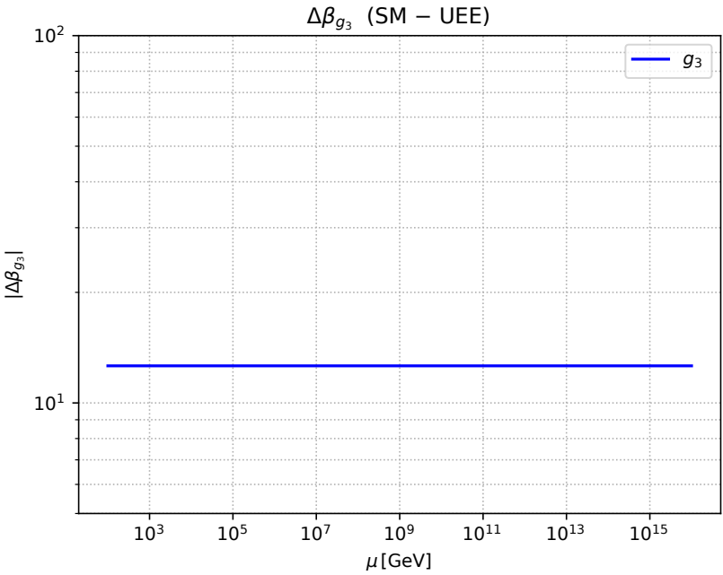
Figure A4. Plot of \Delta\beta_{g_3} only.
