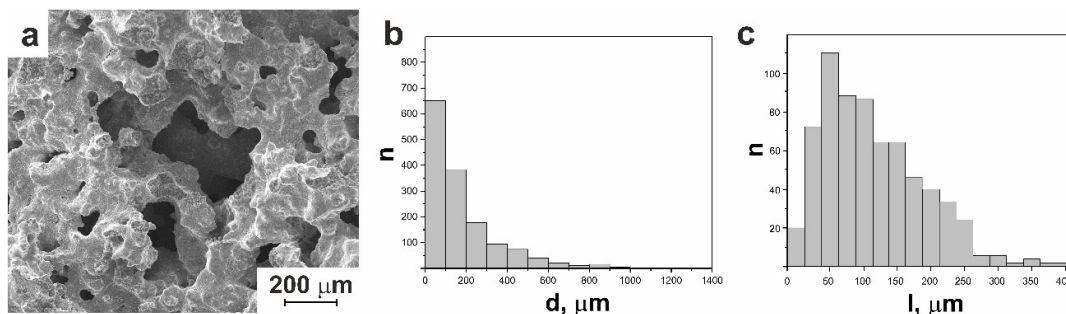
Figure 2. (a) SEM image (SE mode) showing surface morphology of porous SHS-prepared TiNi alloy. (b,c) Histograms of pore size (b) and of inter pore bridge size (c) distribution in the porous TiNi alloy.
