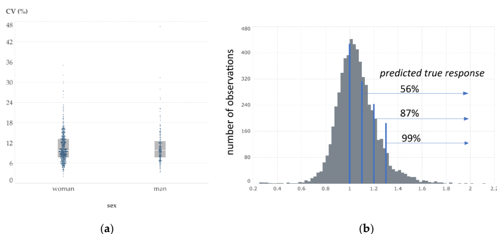
Figure 1. Variance of signals and distribution of SI values. The distribution of CV% values is shown for women and men (a). Assuming a normal distribution for random signals and 10% CV, the percentage of truly increased events can be calculated (b).
