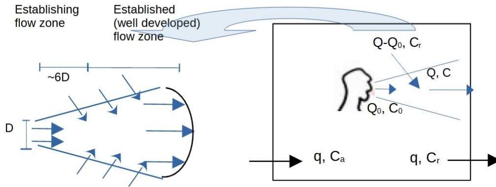
Figure 5. Near-field exhalation cone showing air entrainment.
