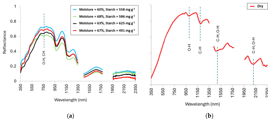
Figure 2. Reflectance spectra of (a) wet saffron corms with different moisture and starch content (each line = one corm; spectrum averaged over [3] scans) shown as examples with their corresponding reference water (%) and starch (mg g -1 , dry weight) and (b) dried (average of 12 samples), powdered saffron corms over 350–2350 nm showing a steep rise to ~1000 nm, a downturn at 1100–1250 nm, a broad hill near 1600 nm, and structured bands at 2000–2100 and 2150–2300 nm (instrumental gaps at ~1350–1450 and 1750–1900 nm).
