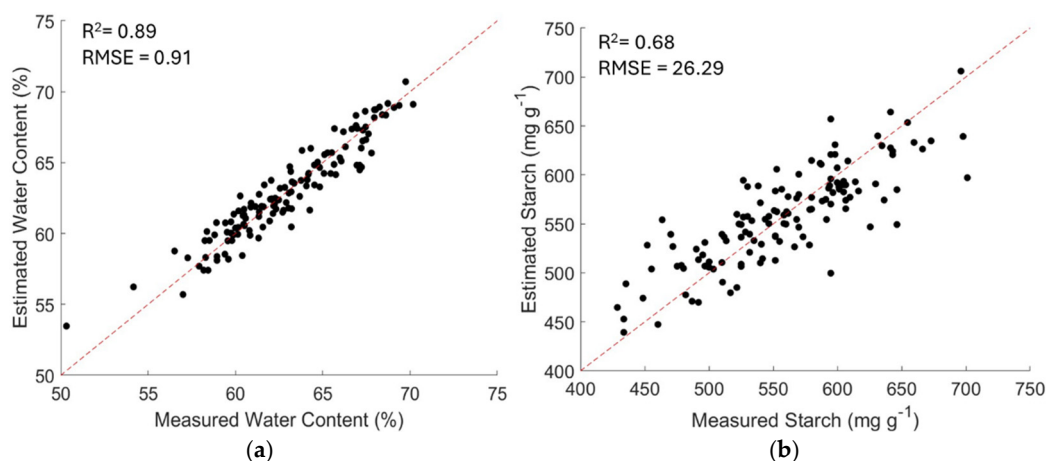
Figure 5. Plots for VIS-NIR predictions in fresh saffron corms ( n = 130 ). (a) moisture content (%)—measured vs. predicted ( R^2 = 0.89 , RMSE = 0.91\% ). (b) starch ( \text{mg g}^{-1} , dry basis)—measured vs. predicted ( R^2 = 0.68 , RMSE = 26.29 \text{ mg g}^{-1} ).
