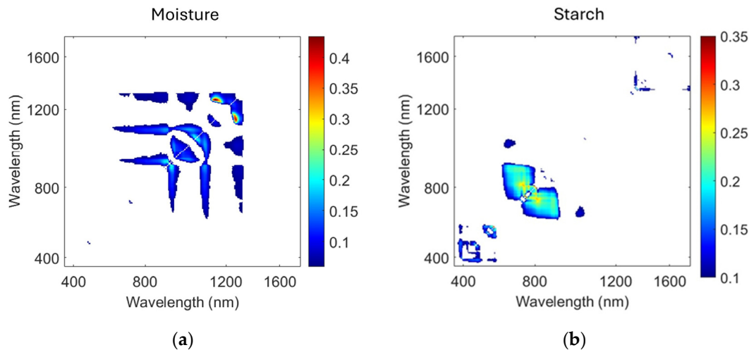
Figure 4. Two-dimensional R^2 heat maps of RI narrowband spectral indices (based on wavelength-pair combinations) for estimating (a) water content and (b) starch content from reflectance spectra (400–1750 nm).
