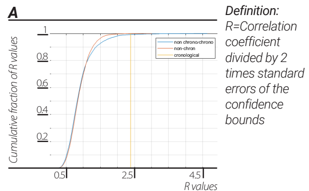
Figure 8: reconstruction of space-time intervals
