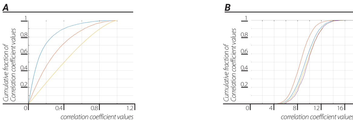
Figure 7: CDF of correlation coefficients in the diffraction experiment between temporally ordered 2-adic representation of edges of dendrograms of different sizes N=5...980 (A, blue trace). CDF of correlation coefficients in the diffraction experiment between non-temporally ordered 2-adic representation of edges of dendrograms of different sizes N=5...980 (A, orange trace). CDF of correlation coefficients between randomly constructed, 2-adic representation of edges of dendrograms of different sizes N=5...980 (A, yellow trace). Coarse graining the universal dendrogram for each N=5...980 frames show differences in p-adic representation between consecutive chronological dendrograms coarse grained edges (B, blue trace) non chronological dendrograms coarse grained edges (B, orange trace) randomization of chronological sequence of dendrogram edges before coarse graining (B, yellow trace), random binary data (B, purple trace).
