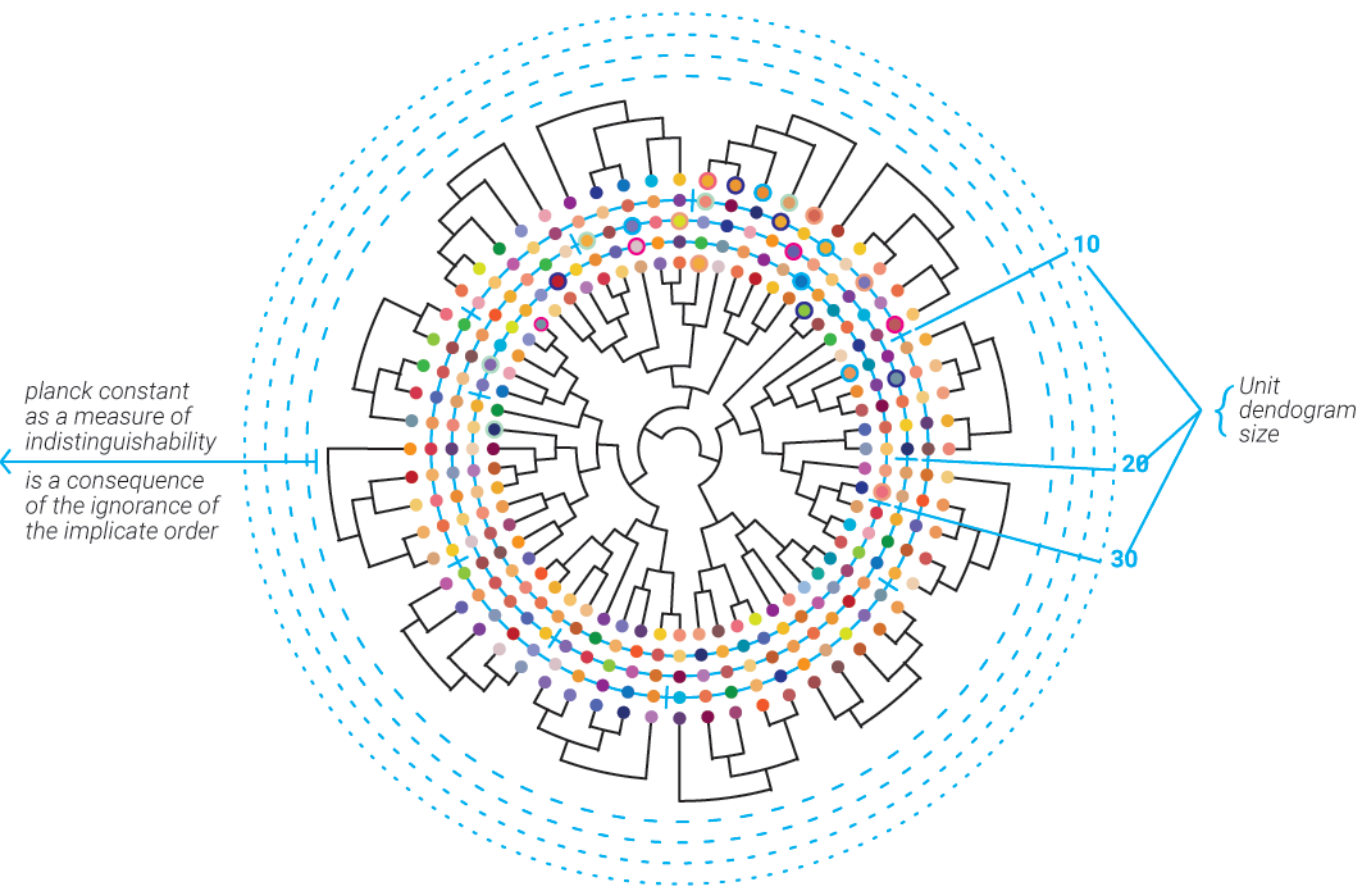
Fig. 3: Abstract description of the implicate and extrinsic order along side the emergence of Planck's constant as a measure of indistinguishability. The "Universal" dendrogram is shown at the center of the circle with its color spheres edges describing each edge 2-adic expansion values of edge route. The outer spheres circles describe the 2-adic values of each edge in the "unit" temporal dendrogram with decreasing edge numbers N = 20, 10, 5 . Each unit dendrogram 2-adic values were best-matched to its corresponding edges in the smaller (higher edge number) circle compared to its non-corresponding edges (see for example 5 spheres with rings in each circle). Planck's constant is the measure of indistinguishability, which is a consequence of the ignorance of each dendrogram edge from the infinite sub dendrograms that continue from it (outer dotted circles).
