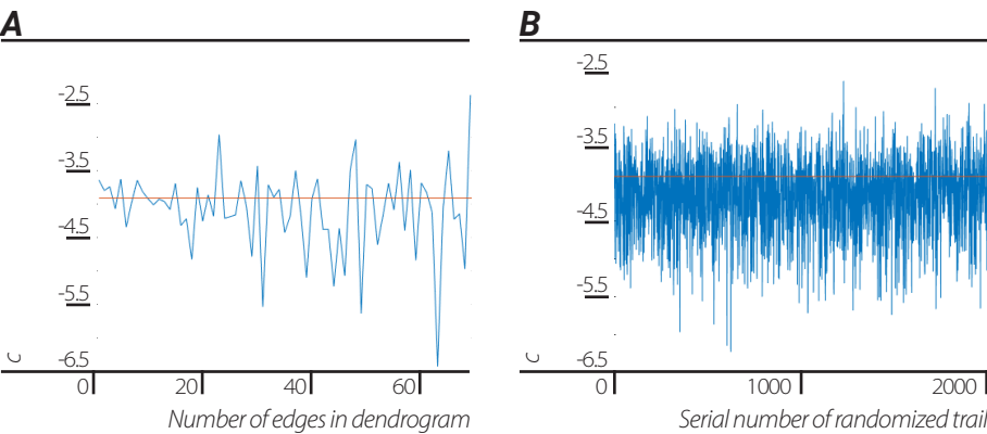
figure 4: emergence of planck constant and speed of light
