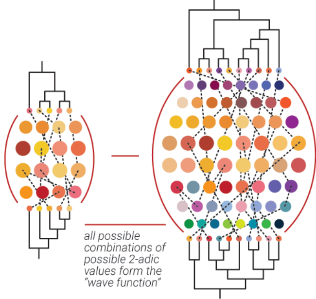
Figure 6: measurement of the wave function according to maximal variety principal
