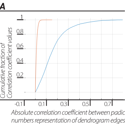
Fig. 5: Cumulative distribution function (cdf) of correlation between the same events represented as 2-adic values in dendrograms of different sizes N = 5 \dots 3920 (blue line) and cdf of the absolute correlation between different events represented as 2-adic values in dendrograms of different sizes N = 5 \dots 3920 (orange line)
