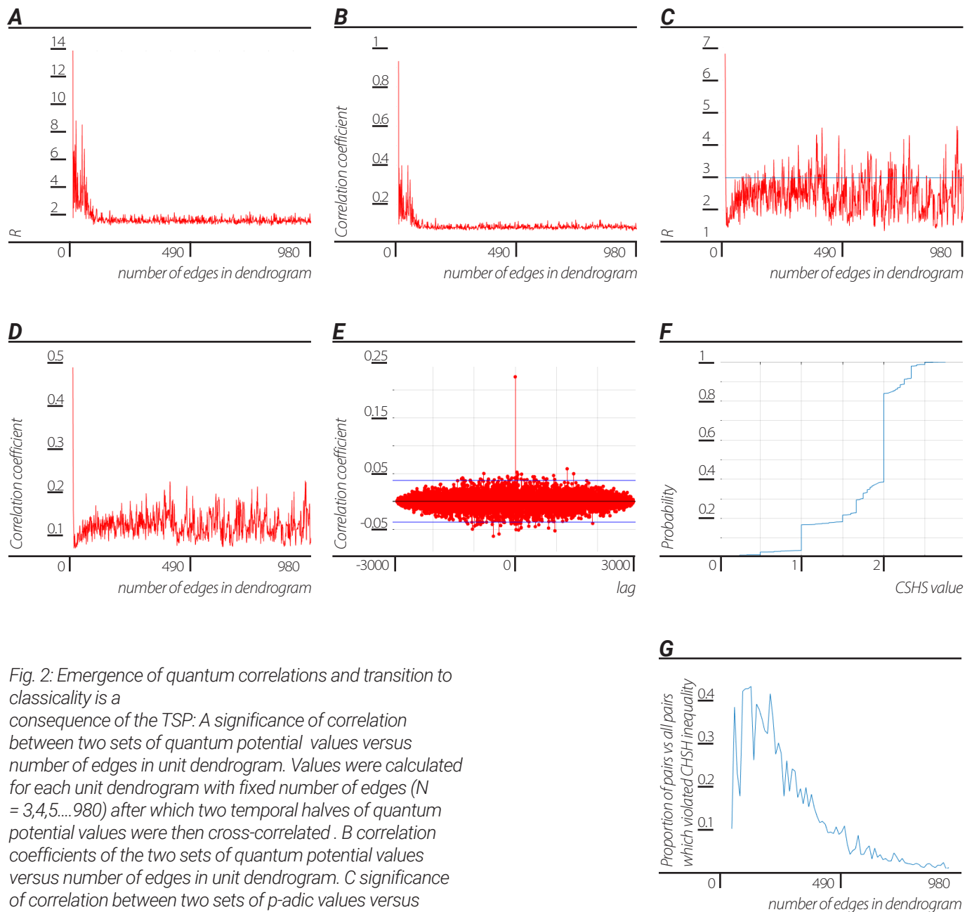
figure 2: quantum correlations from classical data and the transition from quantum to classicality
