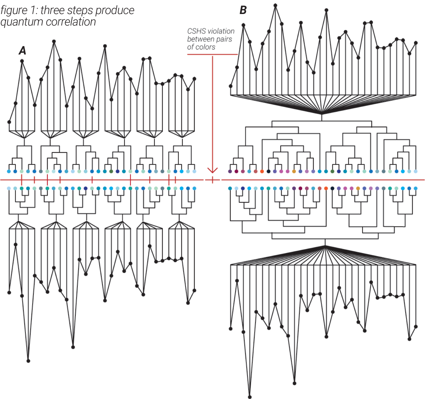
Fig. 1: The emergence of quantum correlations. Illustration of the three steps process (TSP) leading to quantum correlations. Two sets of raw data (black dots) are clustered into two dendrograms each containing 30 edges (B). The same data were clustered into two sets of six dendrograms each with five edges (A). Colored spheres represent the 2-adic values of an edge route in the dendrogram. When examining the correlation between the two sets of 2-adic values on the right, it can be seen that the correlations did not violate the Clauser–Horne–Shimony–Holt (CHSH) inequality. The same raw data, divided into groups of five datapoints and then clustered into a five-edge dendrogram produced pairs of 2-adic values that violate CHSH inequality.
