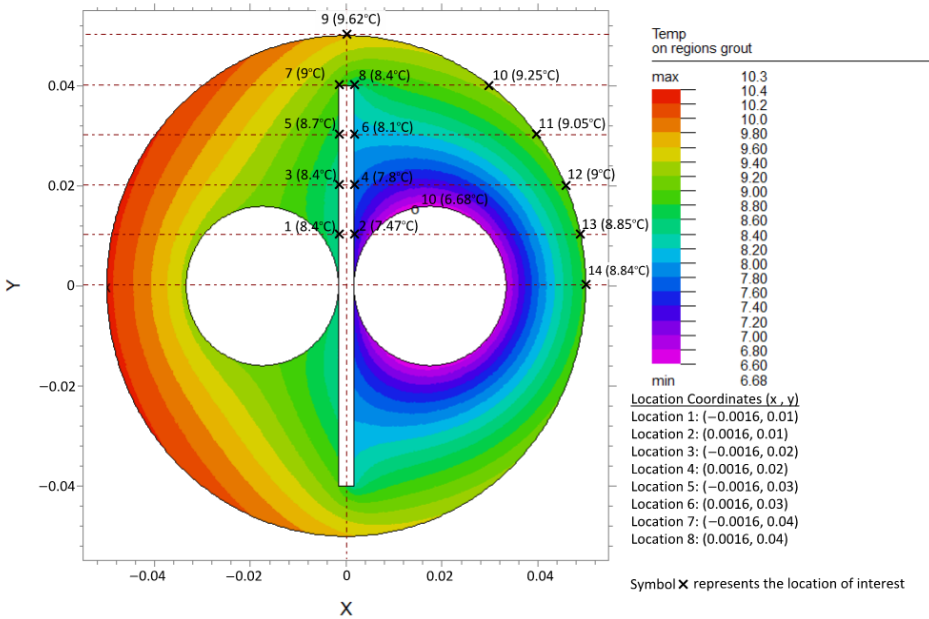
Figure 16. Temperature distribution in grout region for U-tube BHX with barrier arrangement FSB-3PLMT, k_s : 1 W/m·K, k_g : 0.585 W/m·K, and S : 35 mm.
