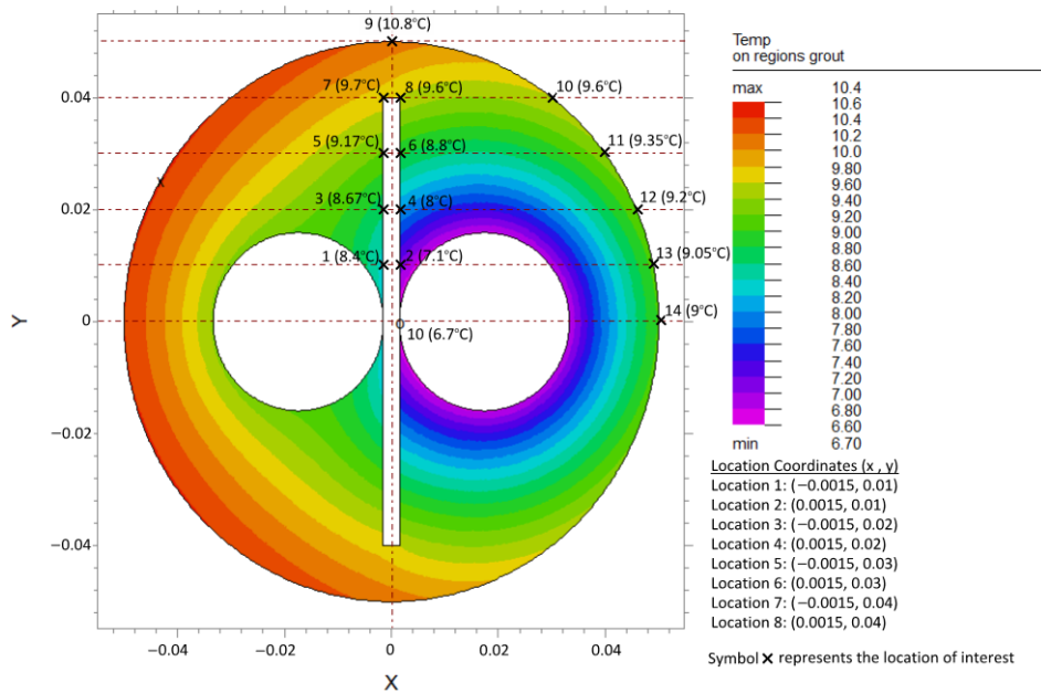
Figure 15. Temperature distribution in grout region for U-tube BHX with barrier arrangement FSB-3PL1, k_s : 1 W/m·K, k_g : 0.585 W/m·K, and S: 34.8 mm.
