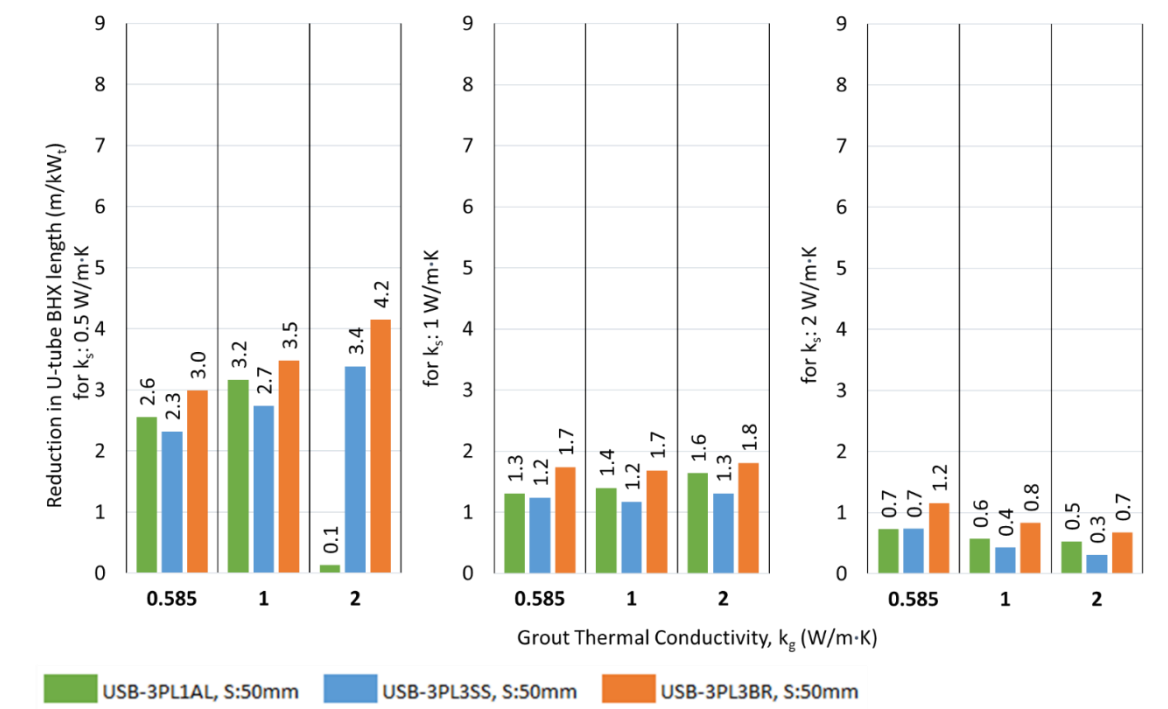
Figure 24. Reduction in the BHX length for various U-barriers; k_s : 2 W/m·K.
