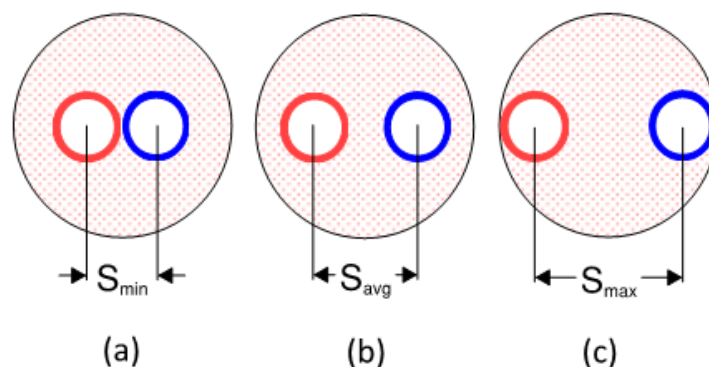
Figure 4. Various shank spacings of U-tube BHX model.
