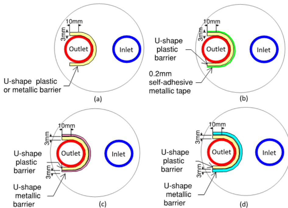
Figure 9. Schematic of U-shape barrier arrangements for U-tube BHX (a) Single 3 mm U-shape plastic or metallic barrier (b) 3 mm U-shape plastic barrier with 0.2 mm metallic tape (c) Double U-shape barrier of 3 mm plastic and 1 mm metal (d) Double U-shape barrier of 3 mm plastic and 3 mm metal.
