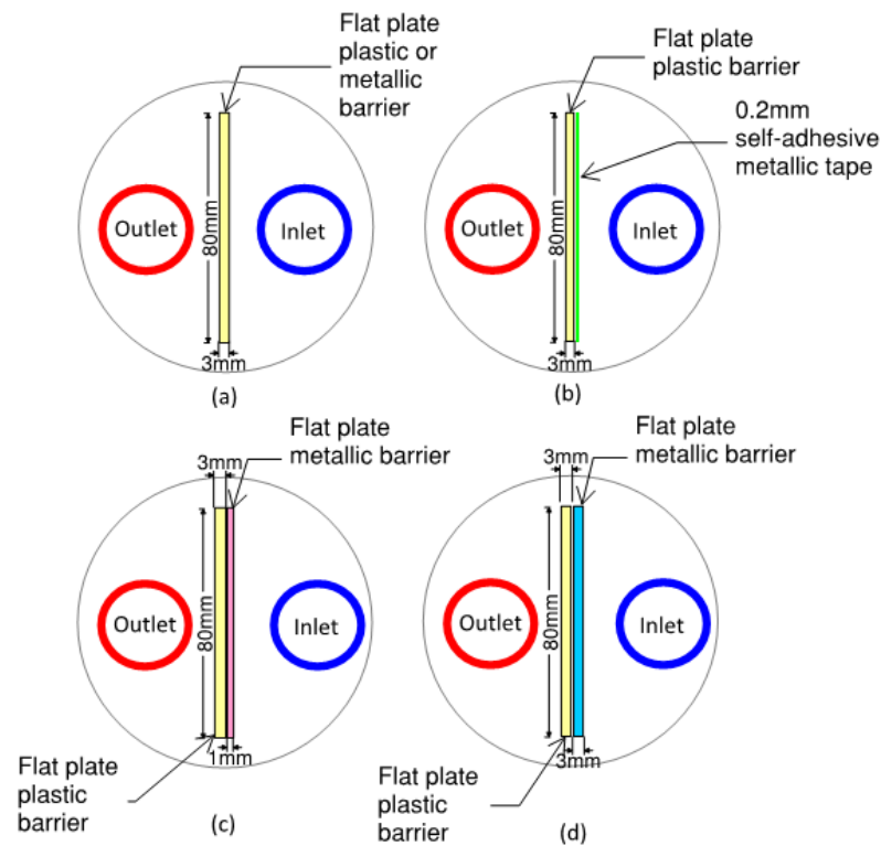
Figure 8. Schematic of flat plate shape barrier arrangements for U-tube BHX (a) Single 3 mm flat plate plastic or metallic barrier (b) 3 mm flat plate plastic barrier with 0.2 mm metallic tape (c) Double flat plate barrier of 3 mm plastic and 1 mm metal (d) Double flat plate barrier of 3 mm plastic and 3 mm metal.
