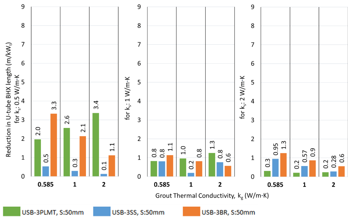
Figure 22. Reduction in the BHX length for various single U-barriers; k_s : 2 W/m-K.
