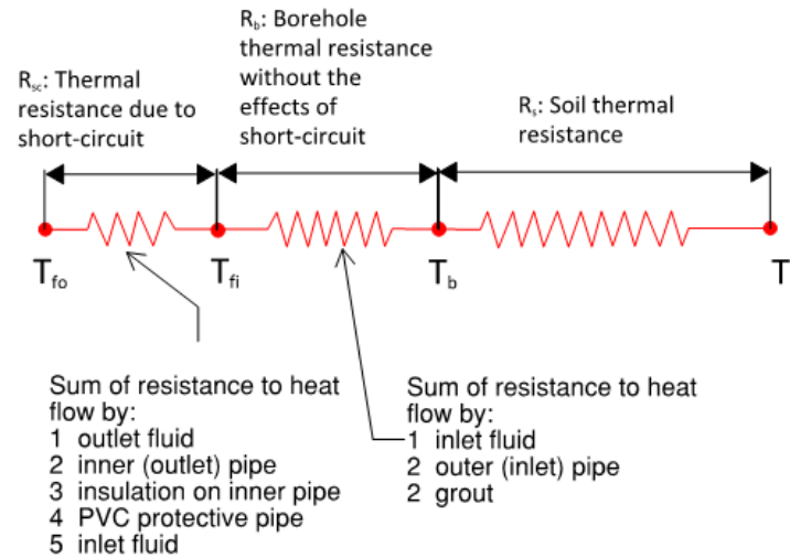
Figure 7. Thermal resistance network for coaxial pipes BHX.
