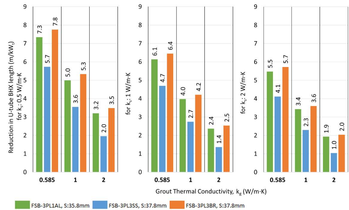
Figure 19. Reduction in U-tube BHX length at S_{min} , for double flat plate barriers at various conditions of grout and soil thermal conductivity.
