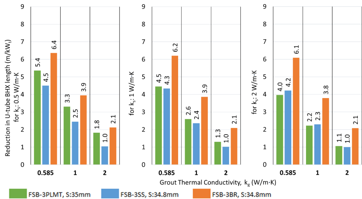
Figure 17. Reduction in U-tube BHX length at S_{min} for flat plate barriers at various conditions of grout and soil thermal conductivity.
