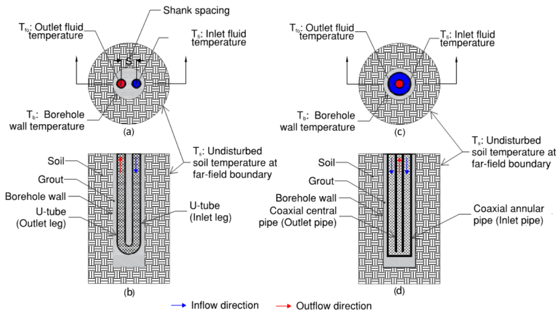
Figure 1. Schematic diagram showing BHX; (a,b) plan and section for U-tube arrangement; (c,d) plan and section for coaxial pipe arrangement with inflow through annular pipe.
