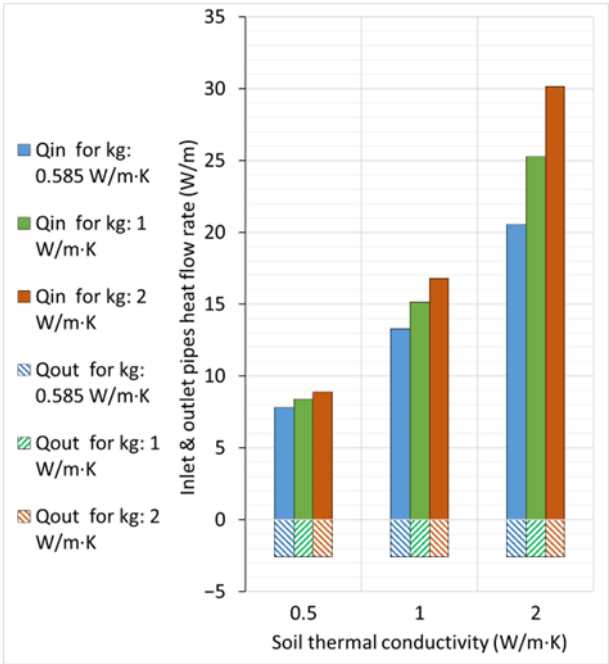
Figure 12. Heat transfer rate from the inlet and outlet pipes for insulated coaxial pipes (inflow through outer pipe).
