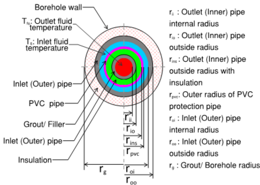
Figure 6. Insulated coaxial pipes model geometry.
