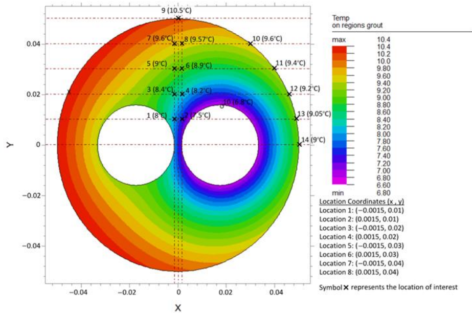
Figure 14. Temperature distribution in grout region for conventional U-tube BHX, k_s : 1 W/m·K, k_g : 0.585 W/m·K, and S: 34.8 mm.
