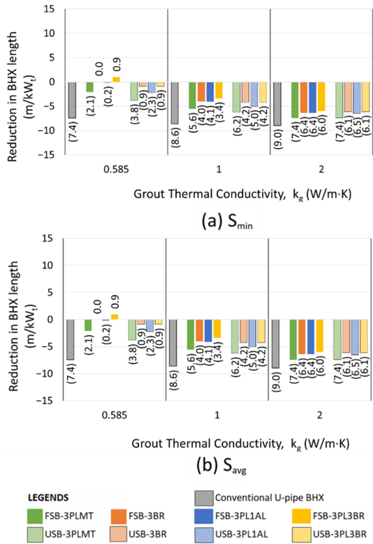
Figure 27. Reduction in length for various arrangements of U-tube BHX compared to coaxial pipes; ks: 2 W/m·K, (a) S_{min} , (b) S_{avg} .
