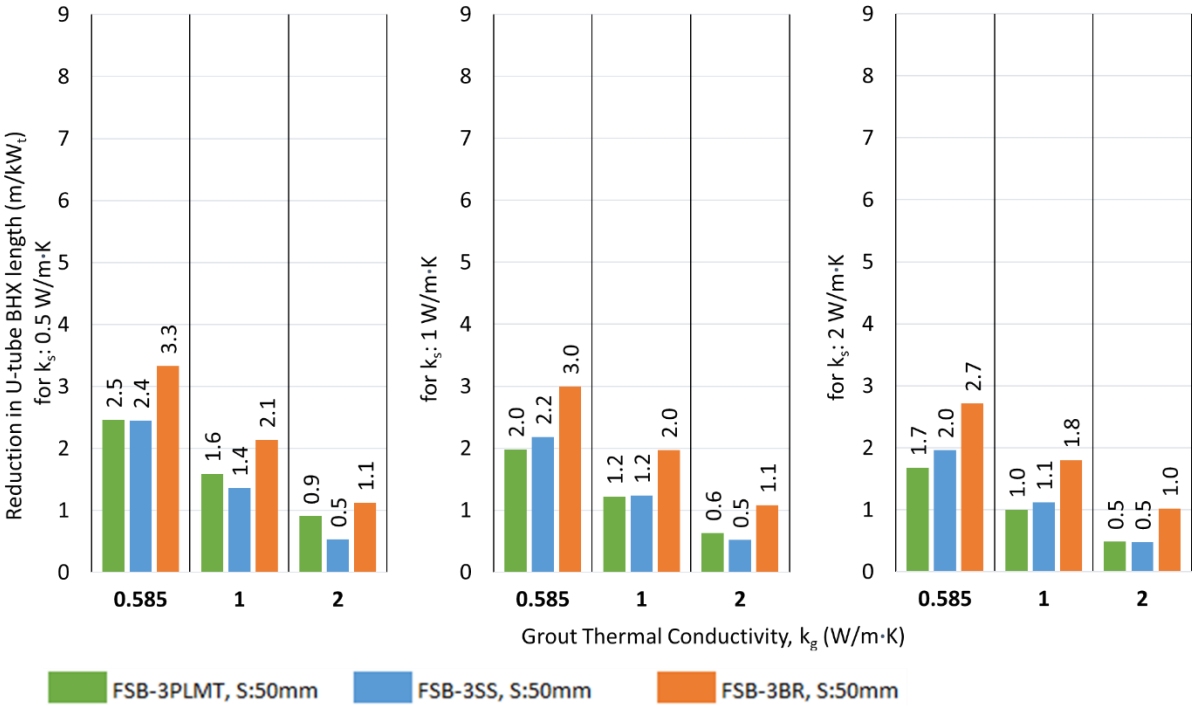
Figure 18. Reduction in U-tube BHX length at S_{avg} for flat plate barriers at various conditions of grout and soil thermal conductivity.
