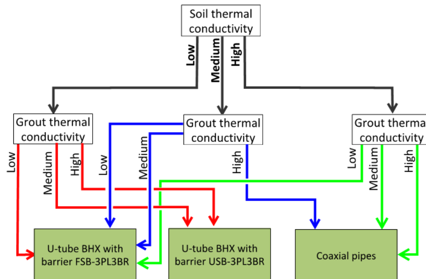
Figure 28. Decision tree for the type of BHX with the minimum length.
