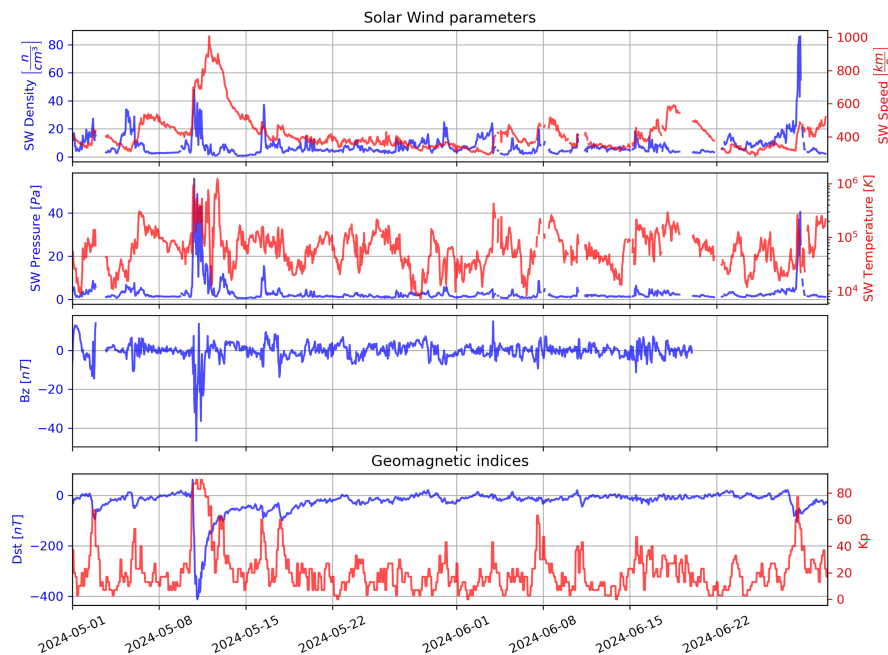
Figure 1. Parameters of the solar wind at 1 AU and geomagnetic indices from omni from May 1 st to June 30 th 2024. Top panel: solar wind density (blue) and solar wind speed (red). Second panel: solar wind pressure (blue) and solar wind temperature (red). Third panel: Southward component of the interplanetary magnetic field B_z . Bottom panel: Dst index (blue) and Kp index multiplied by 10 (red).
