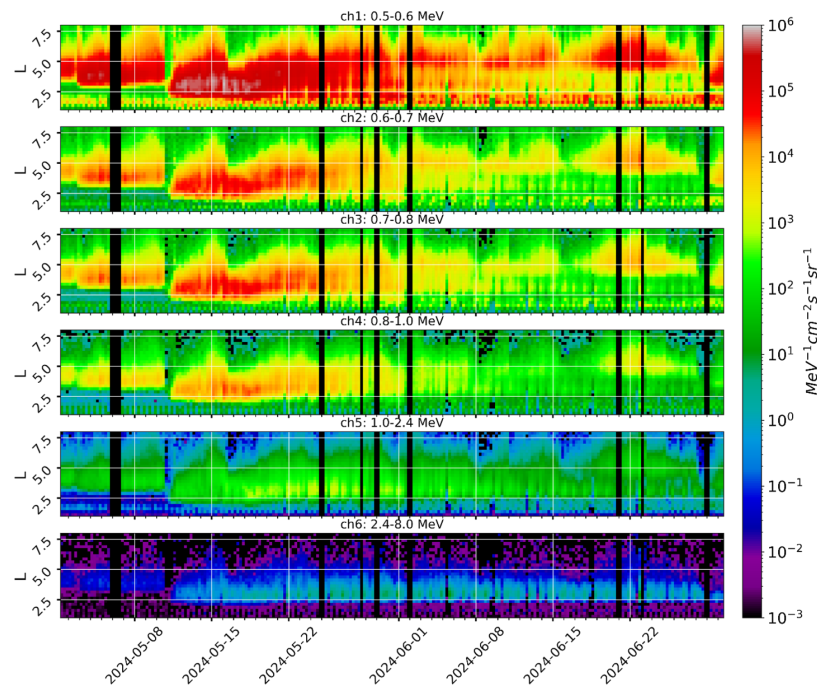
Figure 7. Electron differential fluxes observed from 1 May to 30 June 2024 as a function of the McIlwain parameter L (vertical axis) and time (horizontal axis) in the 6 EPT electron energy channels. Fluxes are averaged in bins which are 6 hours long in time and 0.25 in L . From top to bottom, the energy of the channels increases and they all share the same color bar.
