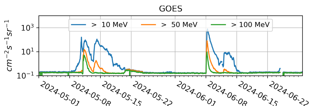
Figure 2. GOES observations of proton fluxes with energy > 10 MeV (blue), > 50 MeV (orange) and > 100 MeV (green) at the geostationary orbit from 1 May 2024 to 30 June 2024.
