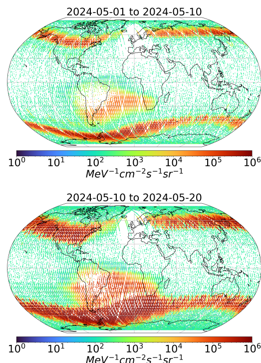
Figure 11. Map of electron flux in Channel 1 (500-600 keV) observed from 1 to 10 May 2024 (before the storm, top panel) and from 11 to 20 May 2024 (after the storm, bottom panel). One can see the South Atlantic Anomaly (high fluxes) and its counterpart in the Northern hemisphere (lower fluxes), as well as the penetration of the outer belt at high latitudes.
