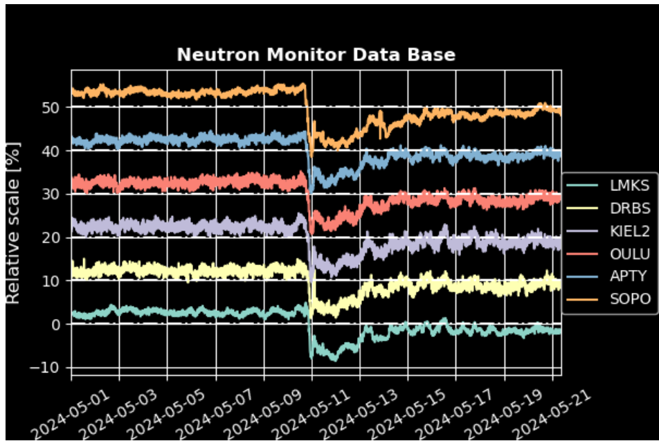
Figure 6. Observations of neutron monitors at different stations specified in Table 1, located at all latitudes like Dourbes (Belgium, 50° lat) and SOPO (South Pole latitude 90°). The perturbation during the night of 10 to 11 May 2024 is well visible. The neutrons decrease during the storm (Forbush decrease) is immediately followed by a Ground Level Enhancement.
