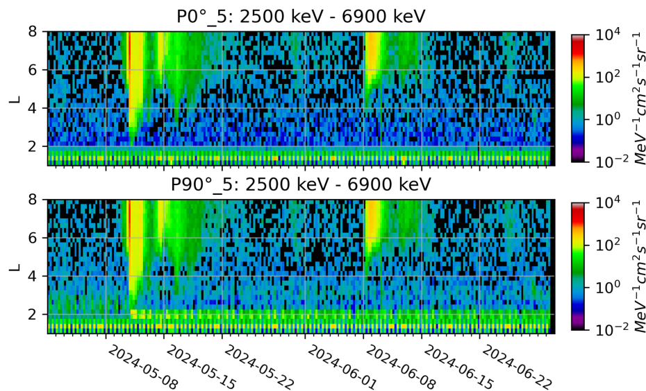
Figure 4. Proton differential fluxes observed by MEPED from 1 May to 30 June 2024 as a function of the McIlwain parameter L (vertical axis) and time (horizontal axis) in 5 th proton energy channel of MEPED. Fluxes are averaged in bins which are 6 hours long in time and 0.25 in L . Top panel: 0° telescope, bottom panel: 90° telescope.
