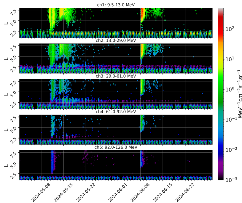
Figure 3. Proton differential fluxes observed by PROBA-V/EPT from 1 May to 30 June 2024 as a function of the McIlwain parameter L (vertical axis) and time (horizontal axis) in the first 5 EPT proton energy channels. Fluxes are averaged in bins which are 6 hours long in time and 0.25 in L. From top to bottom, the energy of each channel increases and they all share the same colorbar.
