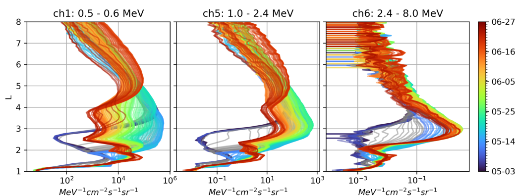
Figure 9. EPT smoothed electron differential fluxes as a function of L and time (color bar) in 3 different energy channels from 3 May to 27 June 2024. Grayed profiles correspond to the period between 8 and 10 May where the smoothed fluxes significantly deviate from the 6 hour averaged fluxes.
