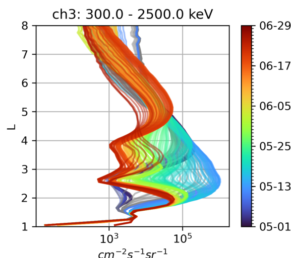
Figure 10. Same as Figure 10 for MEPED 90° telescope for > 300 keV integral electron flux.
