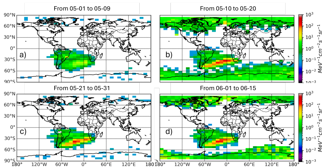
Figure 5. Proton fluxes observed in the first EPT proton channel averaged in longitude and latitude bins during four different periods covering most of the period considered in previous figures. The averaging bins here have a width of 10^\circ in longitude and 5^\circ in latitude. Each panel corresponds to a different period: a) quiet conditions from May 1 st to May 9 th , b) storm time and beginning of the recovery from May 10 th to May 20 th , c) recovery period from May 21 st to May 31 st , d) second proton injection from June 1 th to June 15 th .
