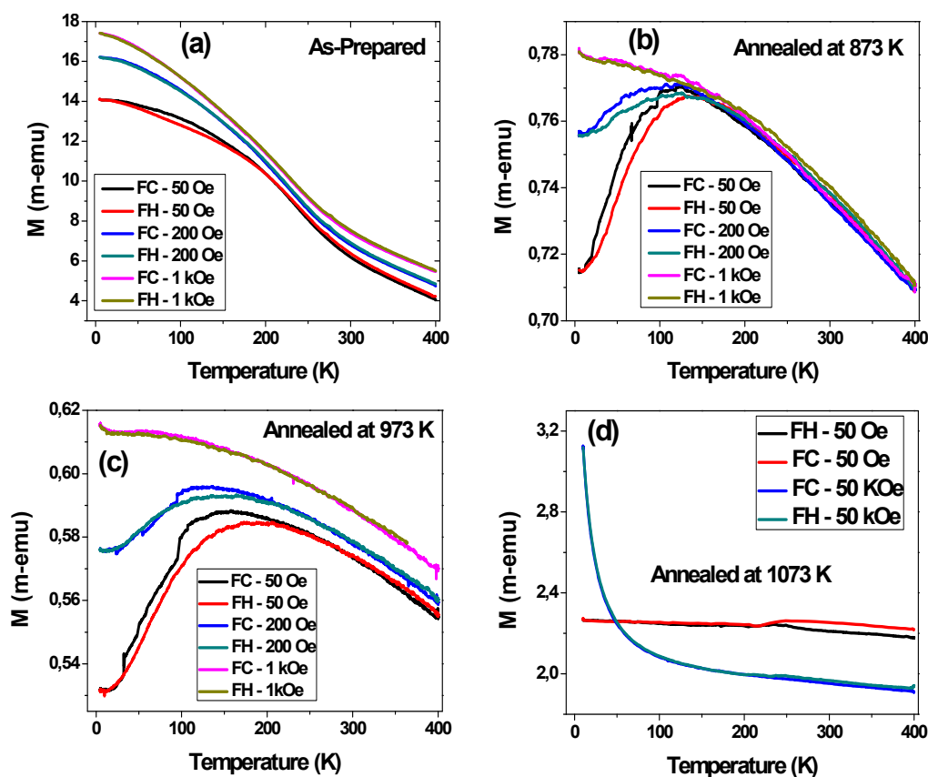
Figure 10. Temperature-dependent magnetization curves for \text{Co}_2\text{FeSi} microwires measured under different applied magnetic fields for (a) as-prepared, (b) annealed at 873 K, (c) annealed at 973 K, and (d) annealed at 1073 K.
