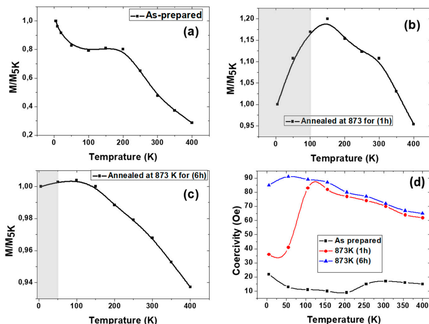
Figure 6. Temperature dependence of the remanence (a) for as prepared, (b) for annealed at 873 (1 h) and (c) for annealed at 873 K for 6 h and the coercivity (d) of \text{Co}_2\text{FeSi} microwire wire investigated samples, respectively (lines for eye guide).
