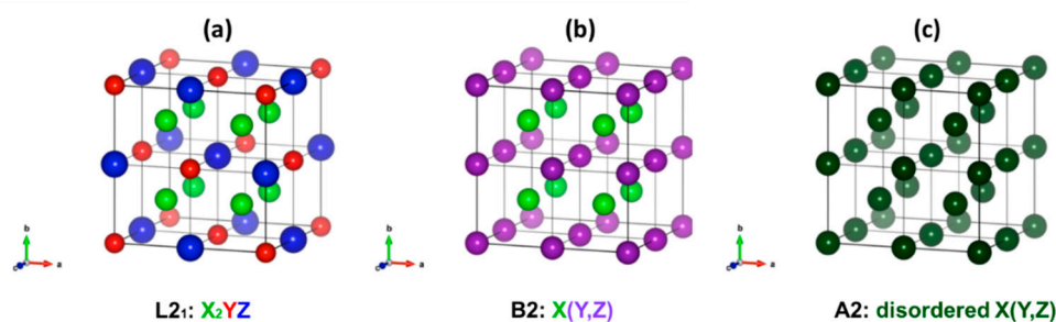
Figure 1. Crystal structures of (a) L2_1 phase and typical disordered phases in Heusler alloys: (b) B2 and (c) A2. B2 phase is disordered between Y and Z but ordered between X and (Y, Z). A2 phase is a completely disordered (random) structure (bcc structure). Unit cells of B2 and A2 are shown by thicker lines in (b) and (c). Figures were reformed from [57].
