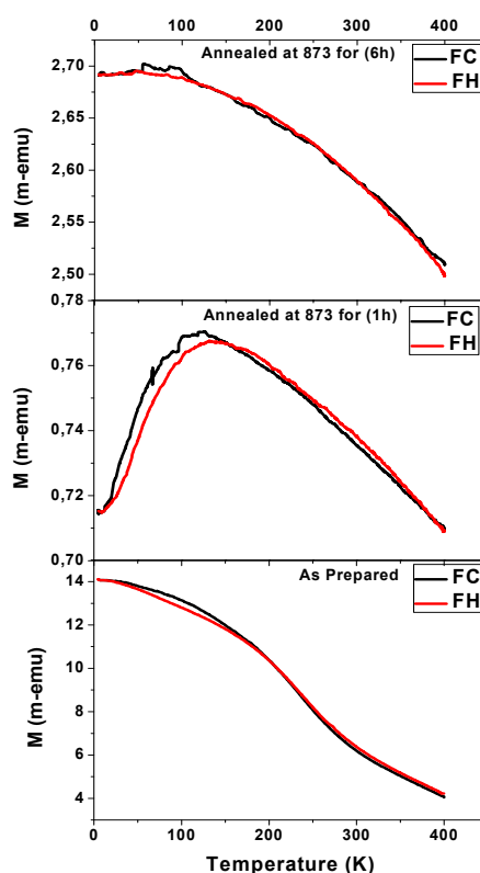
Figure 8. Temperature dependence of magnetization measured for \text{Co}_2\text{FeSi} glass-coated microwires (a) as prepared, (b) annealed at 873 K for 1 h and (c) annealed at 873K for 6 h with applied external magnetic field 50 Oe.
