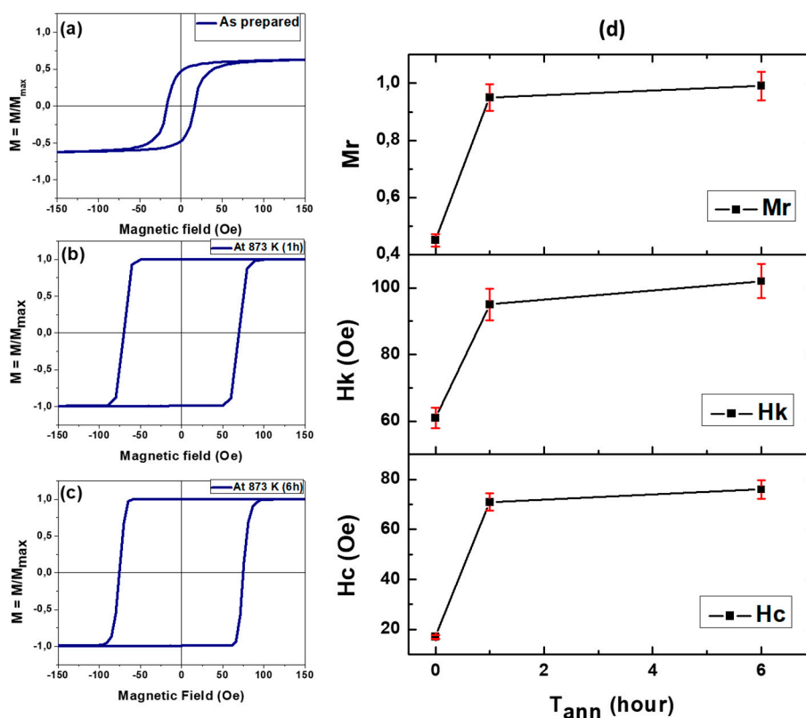
Figure 5. Hysteresis loops of \text{Co}_2\text{FeSi} G-CMMWs: (a) as prepared, (b) annealed at 873 K for 1 hour, and (c) annealed at 873 K for 6 hours. All loops were measured at room temperature. (d) The dependence of coercivity, anisotropy field, and remanence on annealing time for \text{Co}_2\text{FeSi} G-CMMWs is shown (lines are for eye guide).
