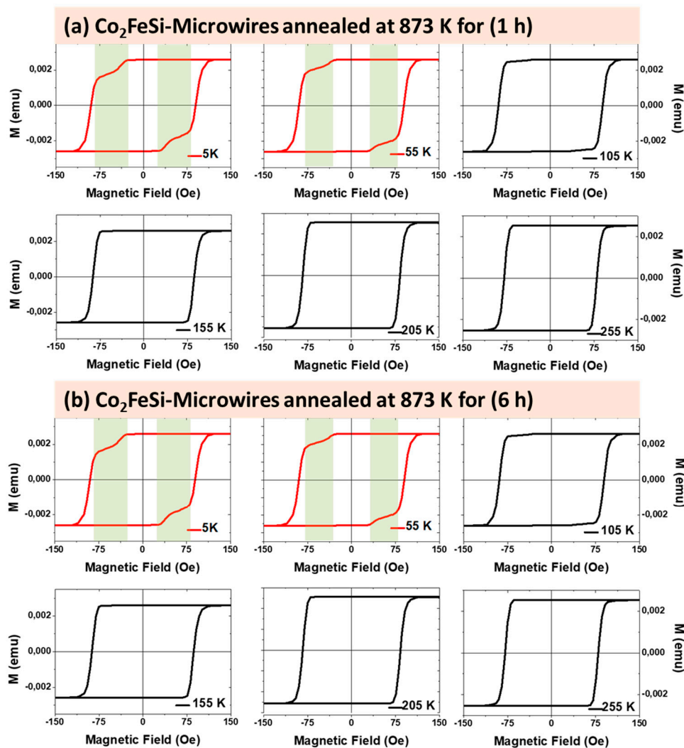
Figure 7. Hysteresis loops measured in a magnetic field applied parallel to the axis of the microwires over the temperature range 5 to 255 K for annealed Co_2FeSi microwires at 873 K for 1 hour (a) and 6 hours (b).
