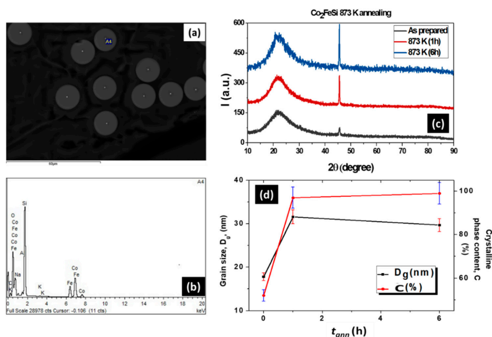
Figure 3. (a) SEM image showing the cross-section of as-prepared \text{Co}_2\text{FeSi} glass-coated microwires. (b) EDX spectrum from a selected point, confirming the presence of Co, Fe, and Si in the alloy. (c) X-ray diffraction (XRD)
