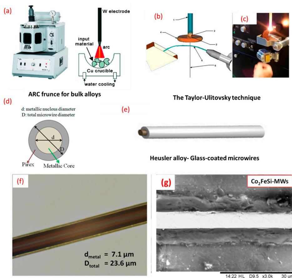
Figure 2. Image of the experimental steps facility for fabrication of thin Heusler based-glass-coated microwires. (a) indicates arc melting furnace (b) and (c) Taylor-Ulitovski method for production of glass-coated microwires, (d) and (e) illustrate the Heusler-based glass-coated microwires sketch. (f) Optical microscope and (g) SEM images of Heusler-type Co_2FeSi glass-coated microwires .
