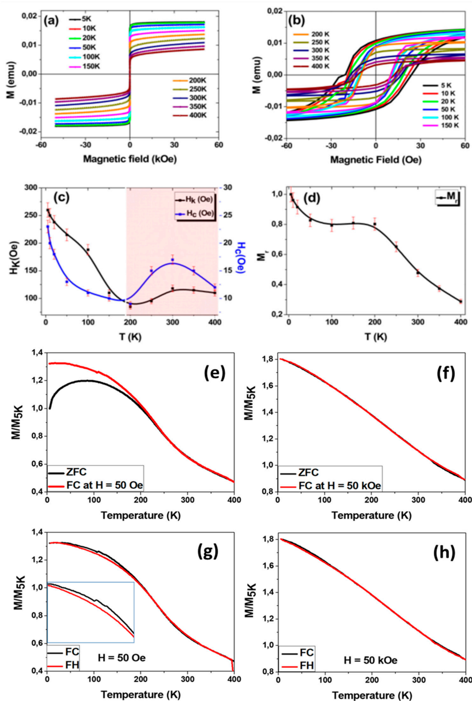
Figure 4. (a) Hysteresis loops of as-prepared Co_2FeSi glass-coated microwires, measured with a magnetic field applied parallel to the wire axis in the temperature range of 5–400 K, with field values between \pm 50 kOe. (b) Hysteresis loops at a lower magnetic field scale. (c) Temperature dependence of coercivity and anisotropy field. (d) Normalized remanence as a function of temperature (lines serve as a visual guide). (e,f) Zero field cooling (ZFC), field cooling (FC) of Co_2FeSi microwires at temperature range 400 K to 5 K with different applied magnetic field low field 50 Oe and high magnetic field 50 kOe, respectively. (g,h) FC from 400 K to 5 K and field heating (FH) from 5 K to 400 K of Co_2FeSi microwires with different applied magnetic field low field 50 Oe and high magnetic field 50 kOe, respectively.
