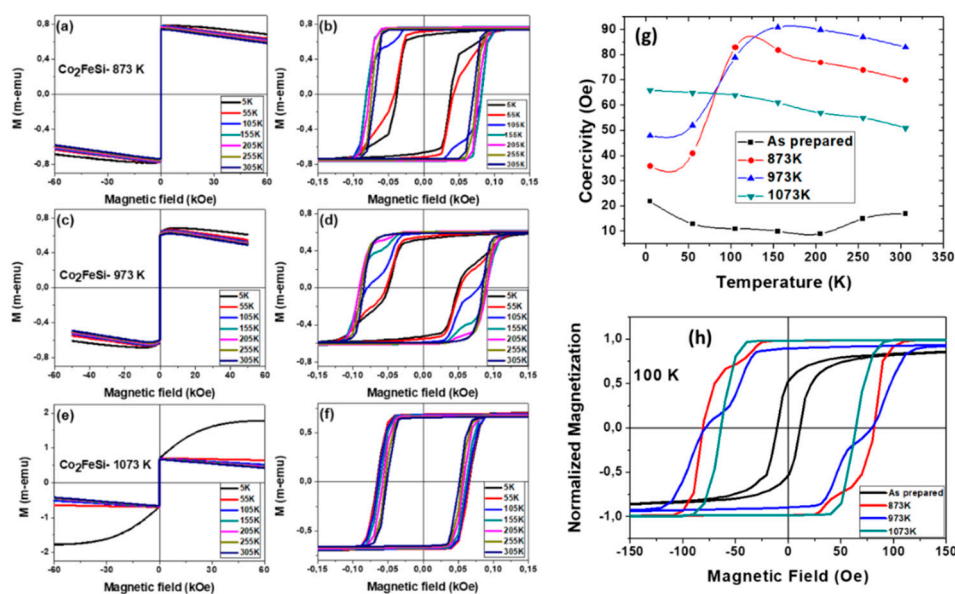
Figure 9. Hysteresis loops of Co_2FeSi microwires annealed at different temperatures for one hour, measured with the magnetic field applied parallel to the microwire axis over a temperature range of 5 to 305 K: (a, b) 873 K, (c, d) 973 K, and (e, f) 1073 K. (g) Temperature-dependent coercivity ( H_c ) for as-prepared and annealed samples at various temperatures (lines serve as a visual guide). (h) Hysteresis loops recorded at 100 K for as-prepared and annealed Co_2FeSi microwires at 873 K, 973 K, and 1073 K, with the magnetic field applied along the microwire axis.
