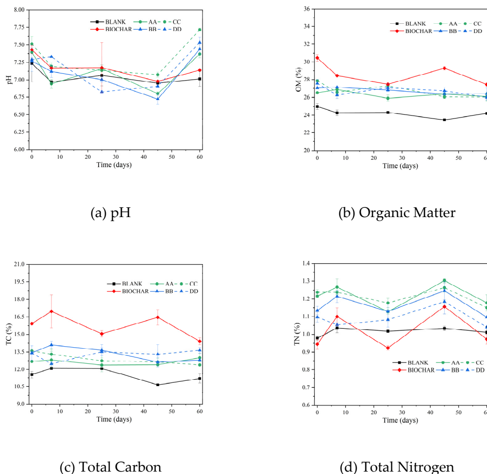
Figure 2. Dynamic changes in soil samples' physicochemical properties: (a) pH, (b) organic matter, (c) total carbon (TC) and (d) total nitrogen (TN).
