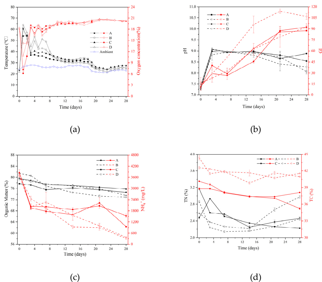
Figure 1. Dynamical changes in (a) temperature and oxygen concentration, (b) pH and germination index (GI), (c) organic matter and ammonia (NH 4 + ), (d) total nitrogen (TN) and total carbon (TC) in the physicochemical properties of compost samples.
