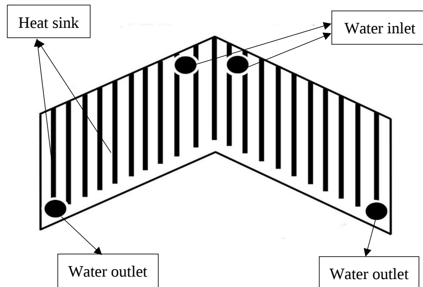
Figure 13. Cooling tank of the Thermoelectric Generator.
