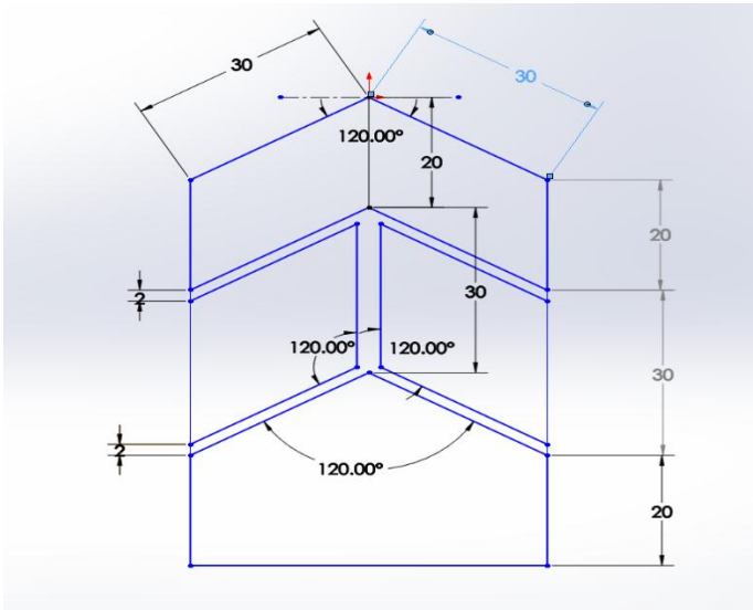
Figure 15. Front View of the system before Extrusion (SOLIDWORKS).
