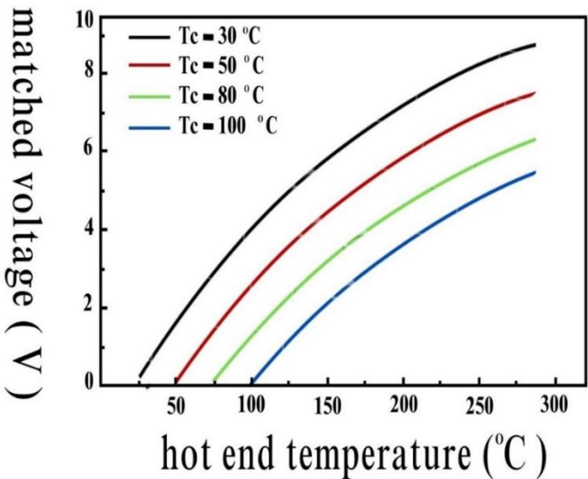
Figure 3. Matched voltage versus Hot end temperature.
