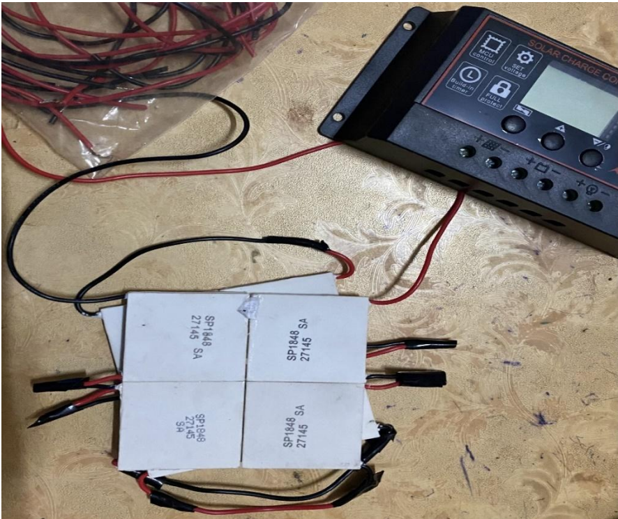
Figure 12. Series connection of Thermoelectric generators along with a charge controller.
