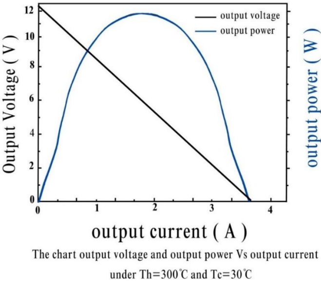
Figure 11. Chart for output voltage and output power versus output current.
