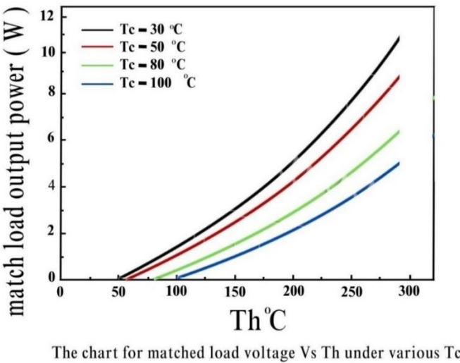
Figure 10. Chart for matched load voltage versus Th under various Tc.
