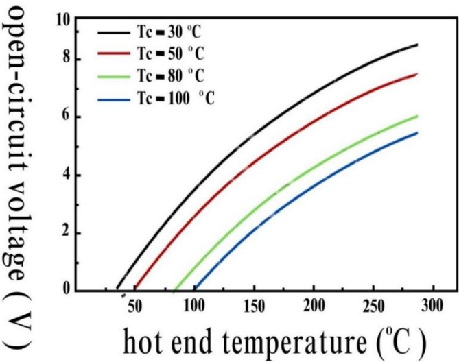
Figure 2. Thevenin voltage (open-circuit) versus Hot end temperature.
