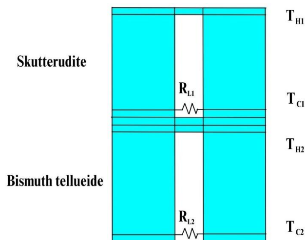
Figure 1. Model of The Two Stage Thermoelectric Generator.
