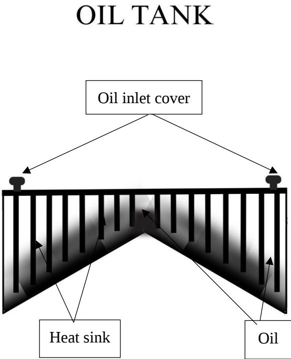
Figure 14. Heating oil tank of the Thermoelectric Generator.
