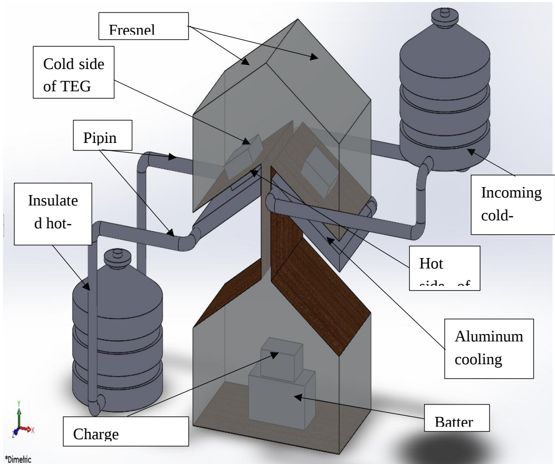
Figure 16. 3D view of the system after Extrusion (SOLIDWORKS).
