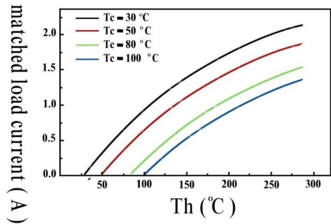
The chart for matched load current Vs Th under various Tc
