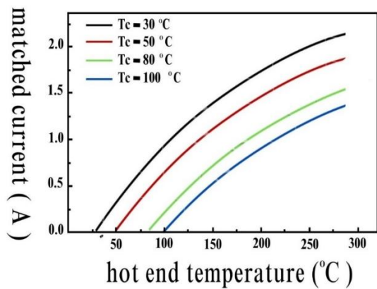
Figure 5. Matched current versus Hot end temperature.
