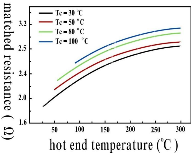
Figure 4. Matched resistance versus Hot end temperature.
