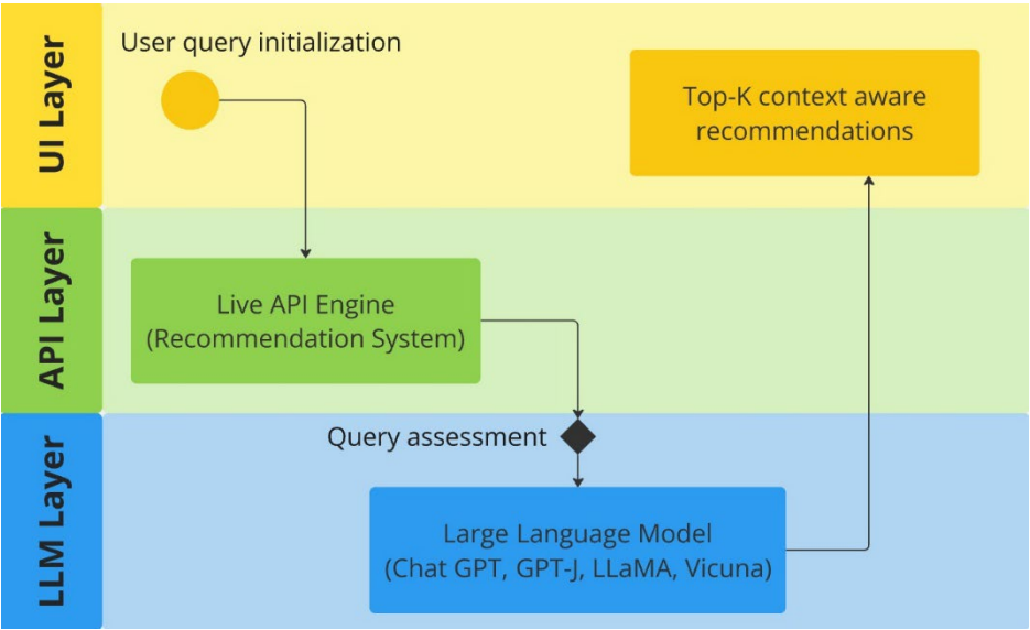
Figure 1. Framework for LLMs Enabled Recommendation Systems.
