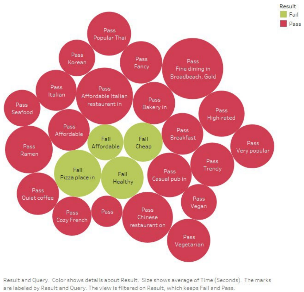
Figure 8. Pass Fail Status of Complex Queries.
