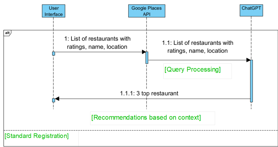
Figure 3. System Sequence Diagram of GPT Restaurant Recommender.
