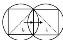
Figure 1. A quantum image of space is a spin foam. When a spin direction is prescribed, a description of cubes is preferred.
