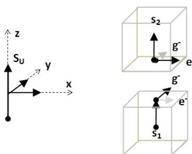
Figure 2. Right; semi spinors s_1 over M face and s_2 over E face. Electric charge over x axis and magnetic charge over y axis.
