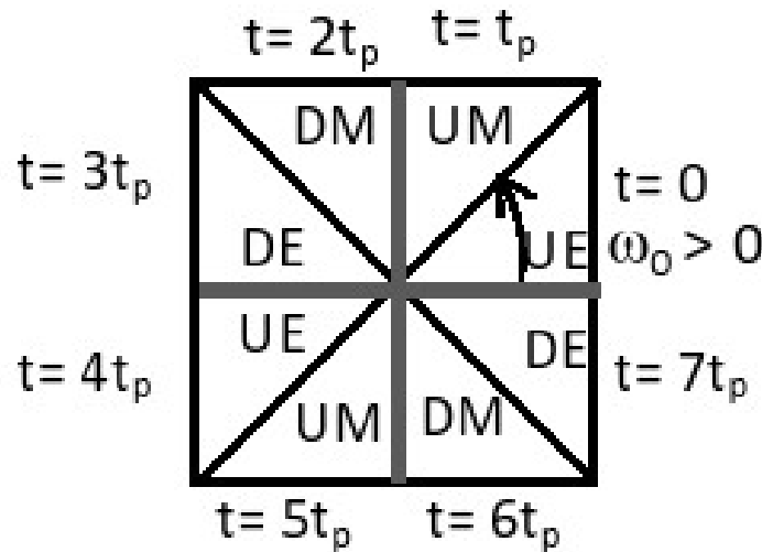
Figure 4. Because the factor \frac{\pi}{8} in \varphi_m , the state s_0(m) in eq. (9) at time t = m.t_p , is in the middle of the interval (t - \frac{t_p}{2}, t + \frac{t_p}{2}) .
