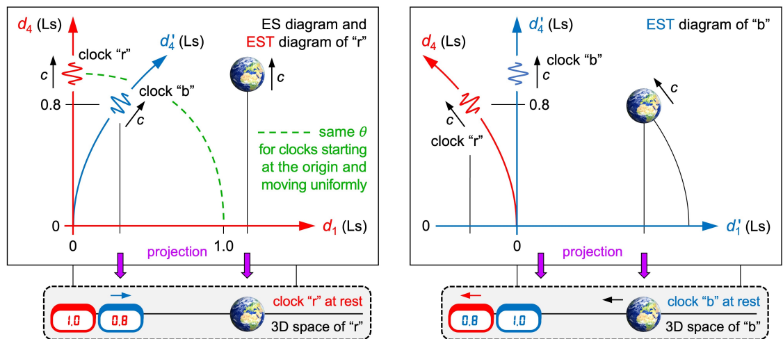
Fig. 3 ES diagram and EST diagrams of two clocks. "b" accelerates toward Earth. Left: ES diagram and likewise EST diagram of "r". The d'_4 axis is drawn curved because it indicates the current 4D motion of "b". Right: EST diagram of "b". This is not (!) an ES diagram because "b" accelerates with respect to absolute ES. EST is relative (two diagrams). ES is absolute (one diagram for all)
