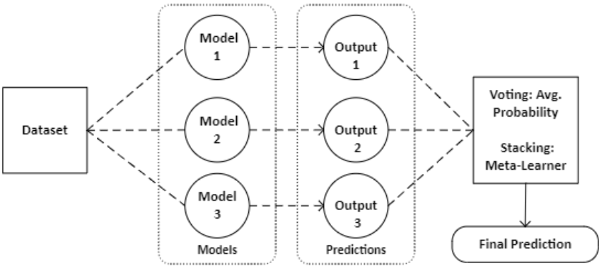
Figure 3. Ensemble Methods.
