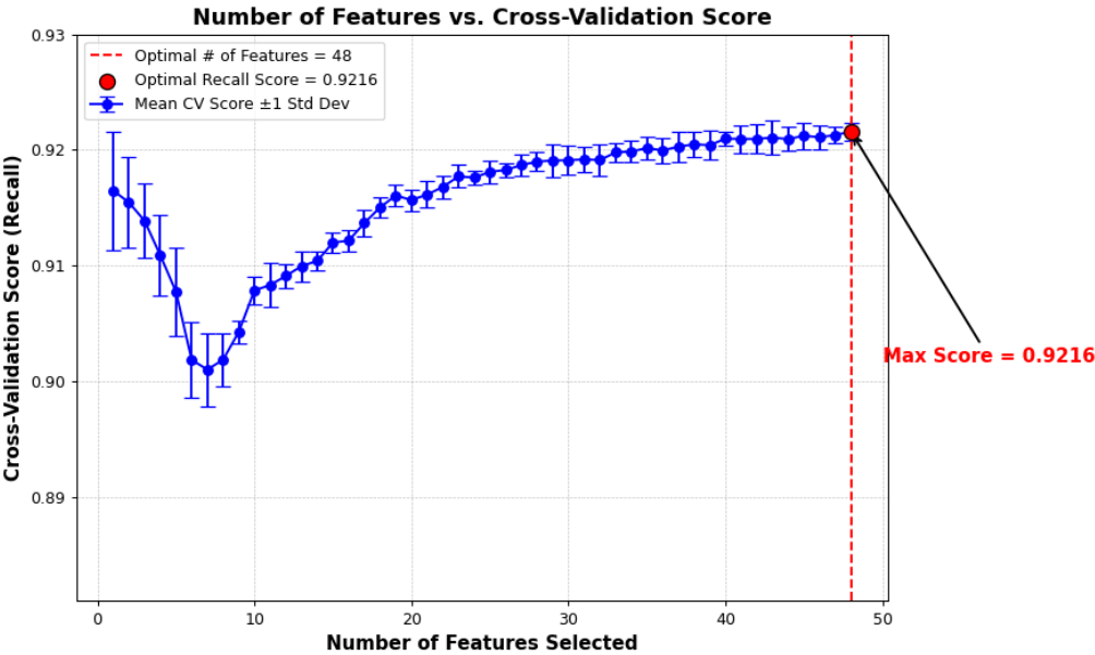
Figure 4. Features Selected.
