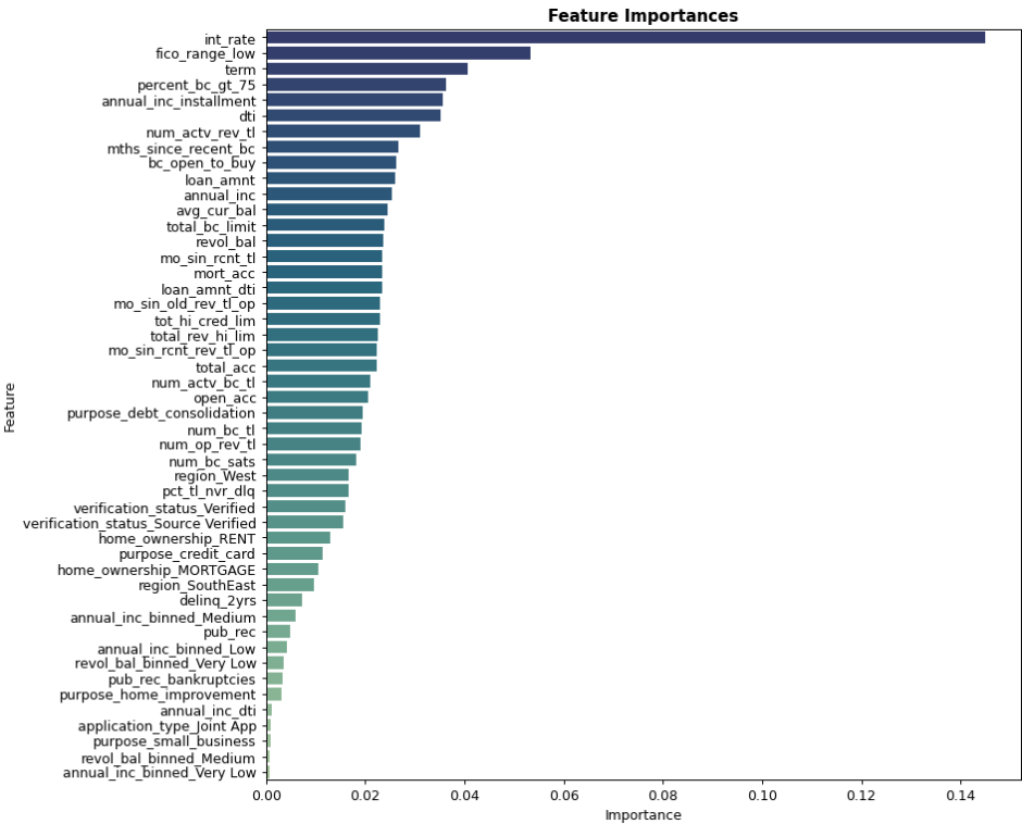
Figure 5. Feature Importance.
