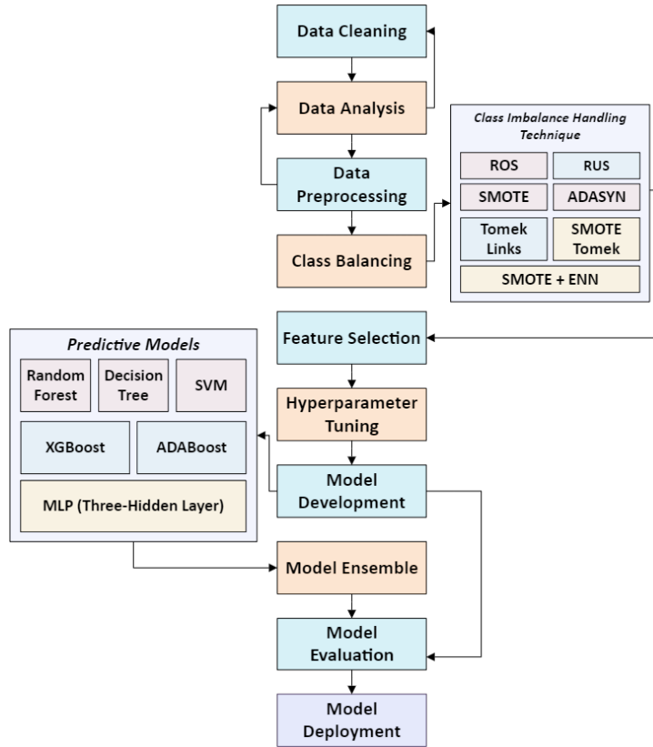
Figure 1. Research Framework.
