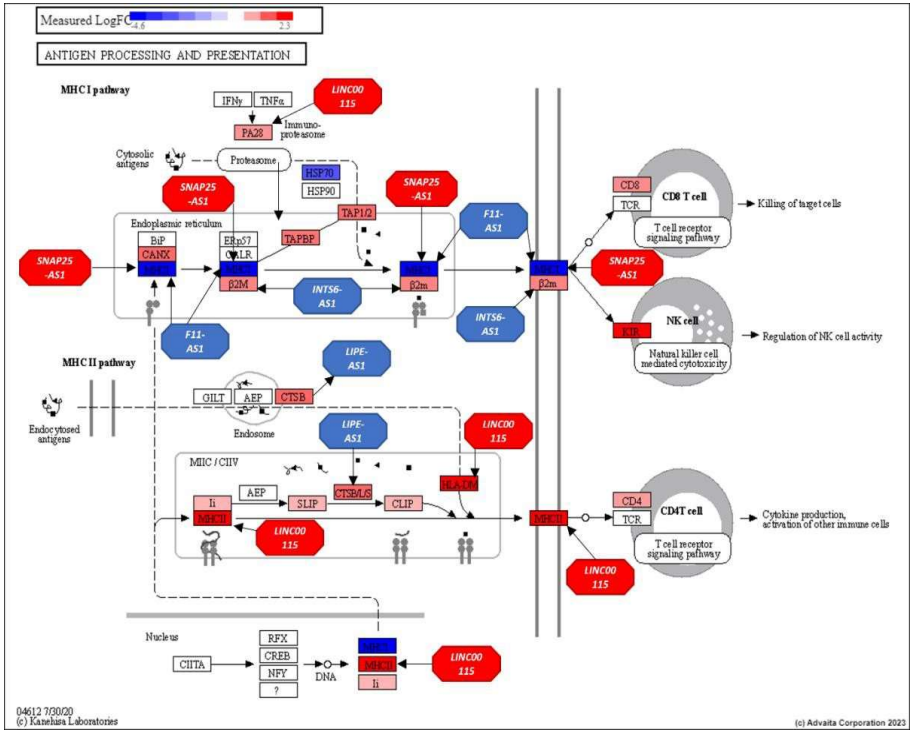
Figure 10. Antigen processing and presentation pathway (KEGG: 04612) displaying gene regulation on AF vs EU prostate differential expression analysis and the influence of lncRNAs identified using structural equivalence analyses. RED: upregulated, BLUE: downregulated.
