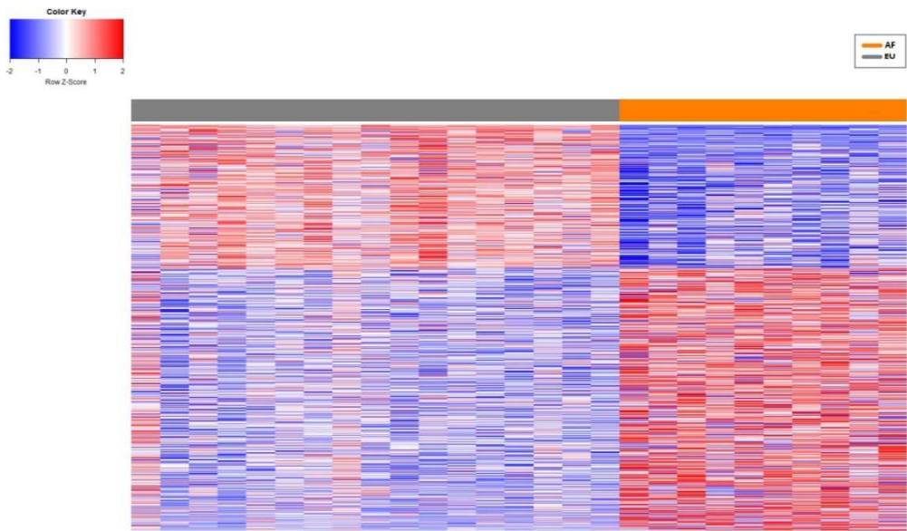
Figure 3. Differential Expression of lncRNAs between patients of African (AF) and European descent (EU). 1,283 lncRNAs significantly DE between AF and EU patients. Red and blue boxes indicate relative over- and under expression with respect to a reference which is calculated as the mid-point between the AF and EU groups. Only lncRNA transcripts found significant at the level q \leq 0.1 and a fold change \geq 1.5 in the comparison, are shown.
