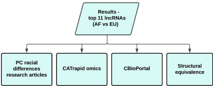
Figure 2. Workflow outlining downstream analyses of the top 11 ranking lncRNAs.
