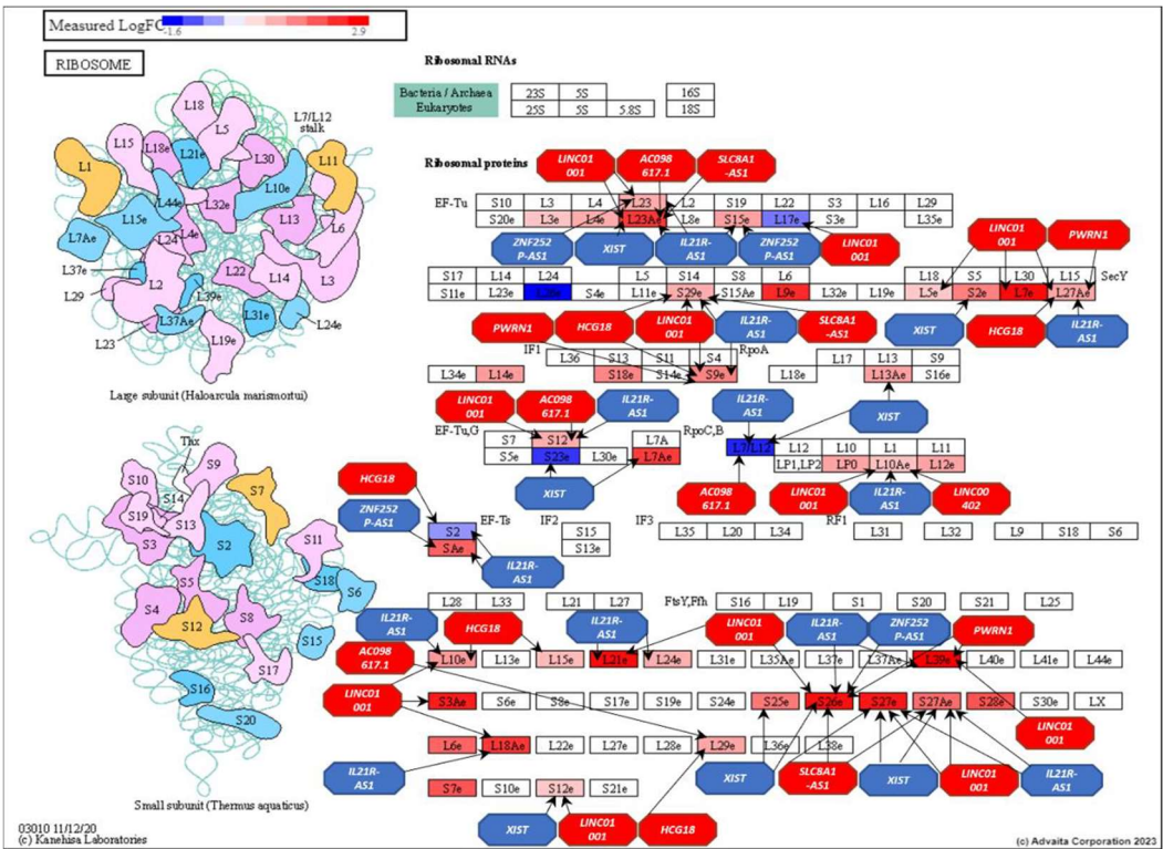
Figure 8. Ribosome pathway (KEGG: 03010) displaying DE gene expression between AF vs EU prostate differential expression analysis and the influence of the top ranking lncRNAs on their regulation. RED: upregulated, BLUE: downregulated.
