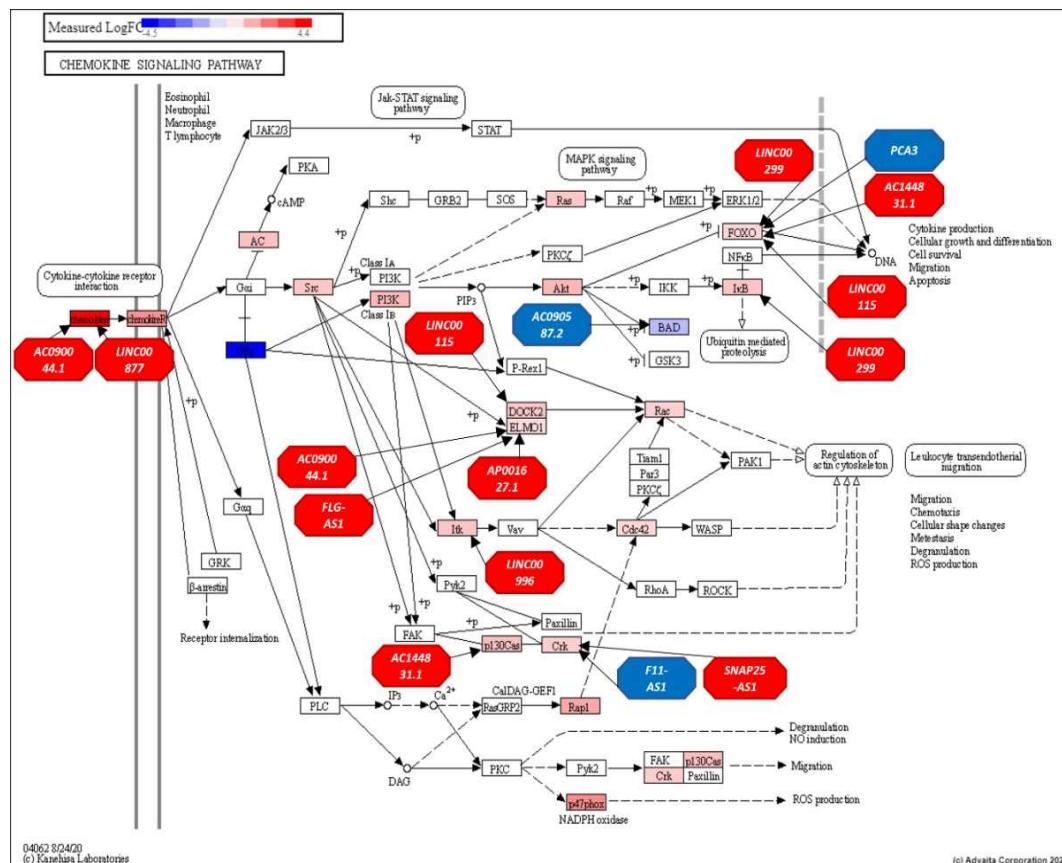
Figure 11. The Chemokine Signaling Pathway (KEGG: hsa04062) illustrates gene regulation differences between AF and European EU prostate cancer patients, highlighting the influence of lncRNAs identified through structural equivalence analysis. RED: upregulated, BLUE: downregulated.
