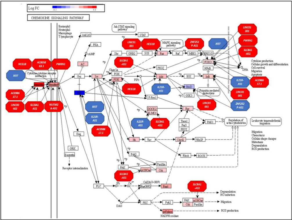
Figure 7. displays the Chemokine signaling pathway with all top ranking lncRNAs and their interaction with pathway genes.
