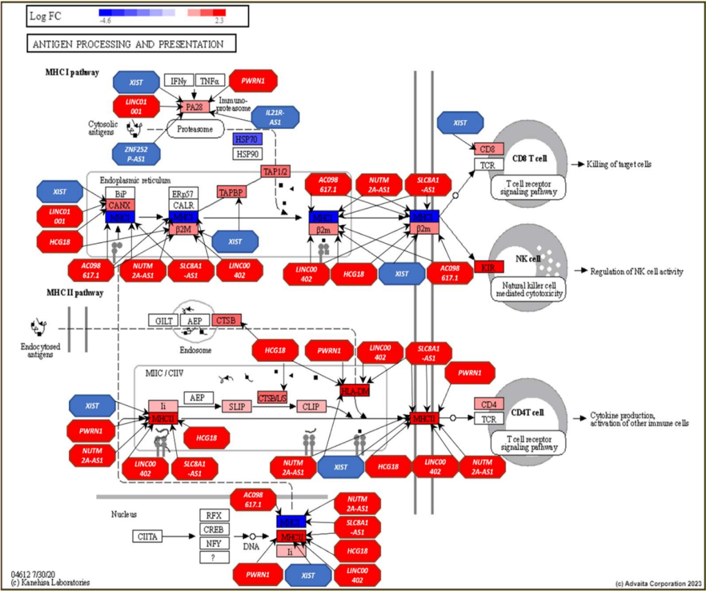
Figure 6. Antigen processing and presentation pathway (KEGG: 04612) displaying DE gene expression between AU vs EU and the influence of the top ranking lncRNAs in the prostate. RED: upregulated, BLUE: downregulated.
