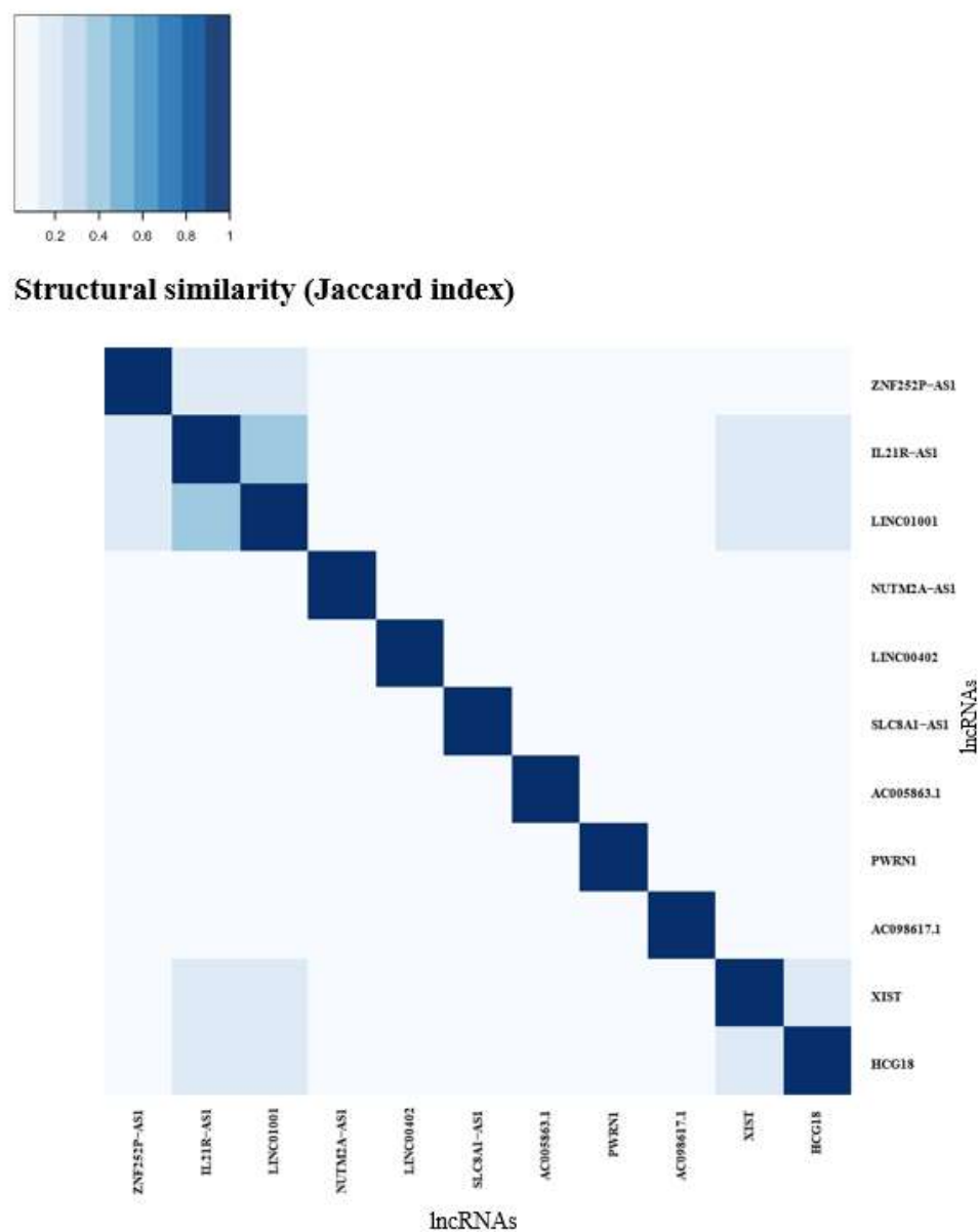
Figure 9. Structural equivalence of the top 11 ranking lncRNAs. Similarity plot of lncRNAs clustered by mRNA target similarity. Darker colors represent higher similarity among the target mRNAs.
