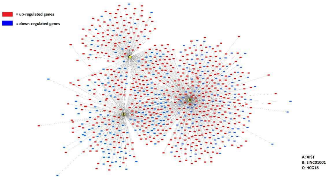
Figure 5. Top 3 ranking lncRNAs ( XIST , LINC01001 & HCG18 ) interacting with the greatest number of mRNA targets. Graphical representation of the top 3 lncRNAs (A: XIST , B: LINC01001 , C: HCG18 ) and their interaction with target mRNAs in AF men. RED: upregulated, BLUE: downregulated.
