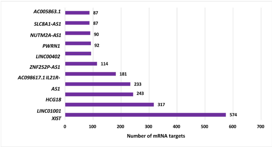
Figure 4. Top ranking lncRNAs. The top 11 long non-coding RNAs (lncRNAs) were ranked based on their centrality. These interactions were constructed using the TCGA Prostate Adenocarcinoma (PRAD) dataset, applying the LongHorn algorithm, and incorporating DE lncRNAs and mRNAs identified in AF patients compared to EU counterparts.
