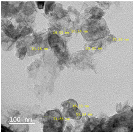
Figure 7. TEM of ZnO aminomodified by hydrothermal process.
