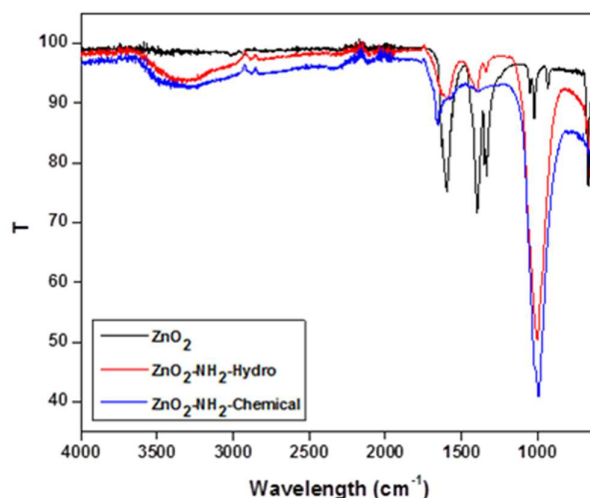
Figure 6. Comparative FTIR of amino functionalised ZnO.
