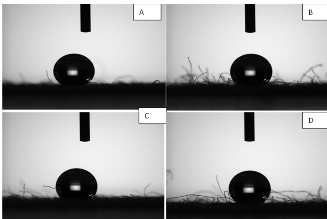
Figure 9. Cotton fabric coated with enzyme-ZnO-PMMA polymer nanocomposite coatings.
