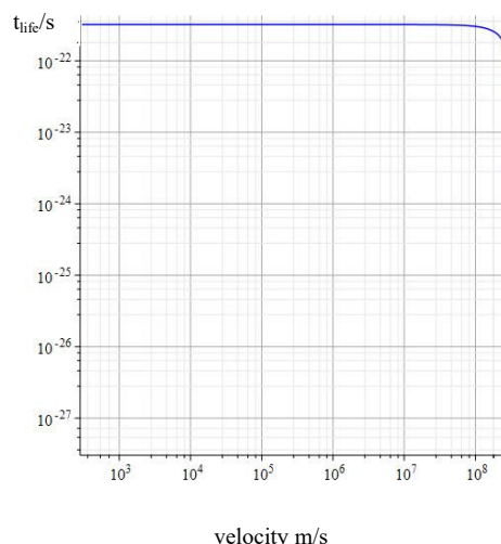
Figure 3. Lifetime of virtual e^-e^+ pairs (Appendix A has Maple™ script).
