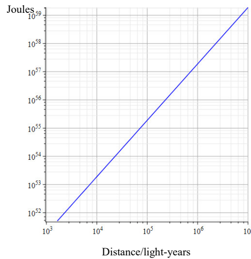
Figure 6. Total Dark-energy vs. distance from galactic centre in light-years (Appendix A has Maple™ script).
