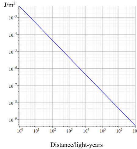
Figure 5. Dark-energy density vs. distance from galactic centre in light-years seen by a distant observer (Appendix A has Maple™ script).
