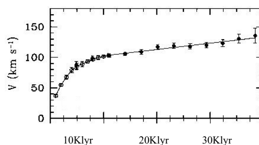
Figure 1. (from [5]) shows a typical velocity distribution curve for a galaxy, in this case, M33 (“Triangulum Galaxy”, some 30 Klyr in radius). There seems to be a perhaps linear increase after 10 kilo-light years or perhaps some other power law. A simple consideration with the mass of the galaxy concentrated at the centre and the centripetal force would arrive at v \propto r^{-0.5} , even if we had a somewhat centrally distributed mass in the galaxy (the initial slow rise of the graph). Use of Gauss’ Law and a uniform, spherical distribution of matter would give v \propto r . A general distribution of matter (for non-relativistic considerations: Newtonian Gravity (NG), which is mostly the case) would involve this integral:
