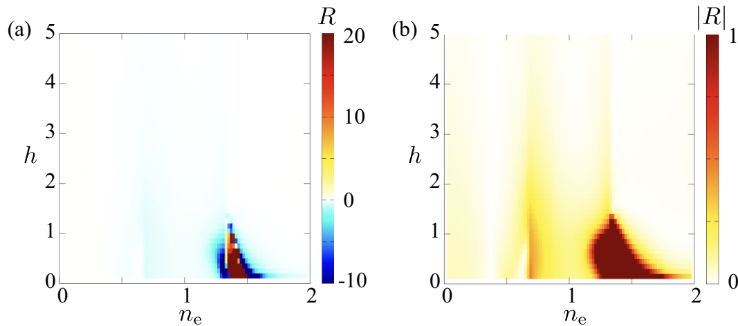
Figure 6. (a) n_e and h dependence of the ratio R = \sigma_{y;xy}^s / \sigma_{y;x}^s at t = 1 , t' = 0.5 , and \tau^{-1} = 0.01 . (b) Enlarged figure of (a) for 0 \leq |R| \leq 1 .
