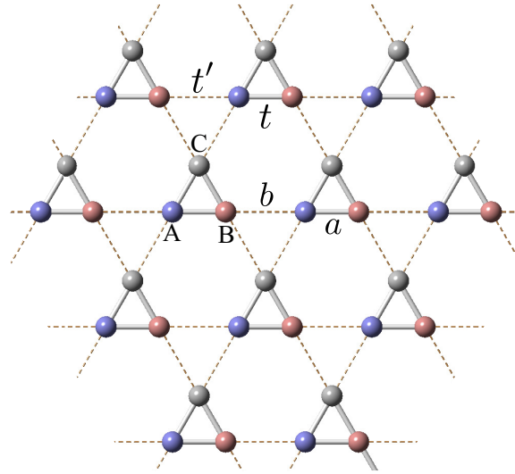
Figure 2. Two-dimensional breathing kagome structure with the lattice constant a + b . The red and blue spheres represent the collinear spin moments along the z direction. t and t' stand for the intra- and inter-sublattice hoppings, respectively.
