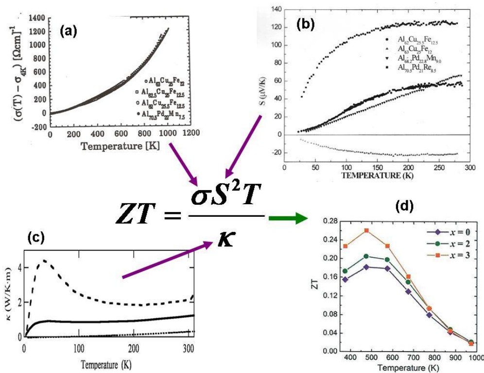
Figure 11. Collage picture illustrating the contribution of each transport coefficient (magenta arrows) to the resulting ZT value (green arrow). Note that panels (a) – (d) correspond to different i-QCs representatives, each one showing an optimal behavior for the considered physical magnitude: (a) Temperature dependence of the electrical conductivity for four different i-QCs up to 1000 K. (Reprinted figure with permission from Mayou, D.; Berger, C.; Cyrot-Lackmann, F.; Klein, T.; Lanco, P. Evidence for unconventional electronic transport in quasicrystals. Phys. Rev. Lett. 1993, 70, 3915-3918. Copyright (1993) by the American Physical Society); (b) Temperature dependence of the Seebeck coefficient for different i-QCs. (Courtesy of Roberto Escudero); (c) Temperature dependence of the thermal conductivity for the i-Al 74.6 Re 17.4 Si 8 QC (solid line) and its 1/1-cubic approximant (dashed line). The contribution due to the electrons (estimated from the Wiedemann-Franz law, dotted line) is almost negligible as compared to that due to the phonons (Courtesy Tsunehiro Takeuchi); (d) ZT curves as a function of temperature for Al 71-x Ga x Pd 20 Mn 9 (x = 0, 2, 3) (Reprinted from Takagiwa, Y.; Kirihaara, K. Metallic-covalent bonding conversion and thermoelectric properties of Al-based icosahedral quasicrystals and approximants. Sci. Technol. Adv. Mater. 2014, 15, 044802; doi:10.1088/1468-6996/15/4/044802, Creative Commons Attribution-NonCommercial-ShareAlike 3.0 License).
