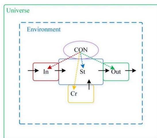
Figure 3. Structure of Standard Agent Model.
