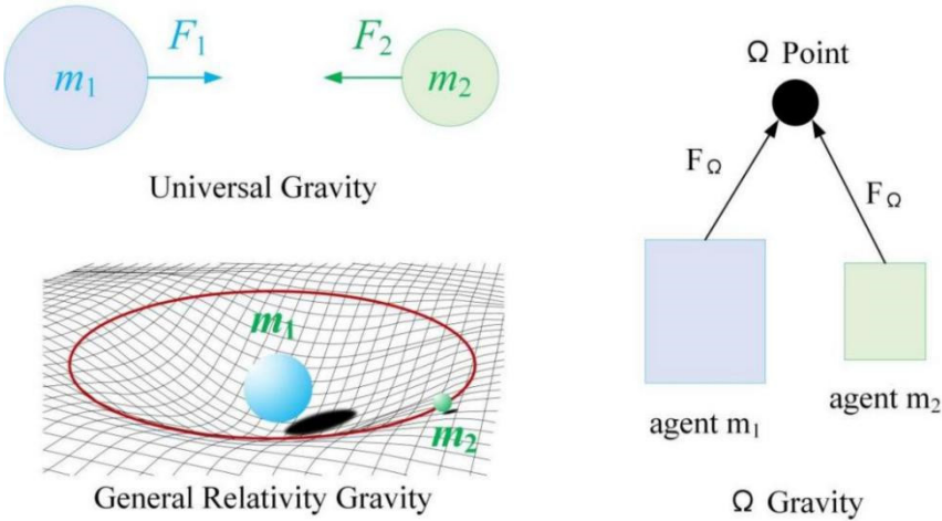
Figure 9. Illustrations of Universal Gravitation, General Relativity Gravity, and \Omega Gravity.
