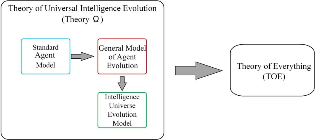
Figure 2. \Omega Theory and TOE.
