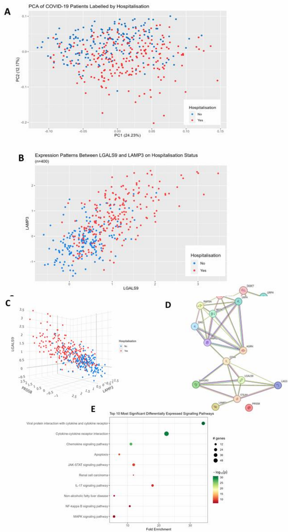
Figure 2: COVID-19 Patient Separation and Signaling Differences
