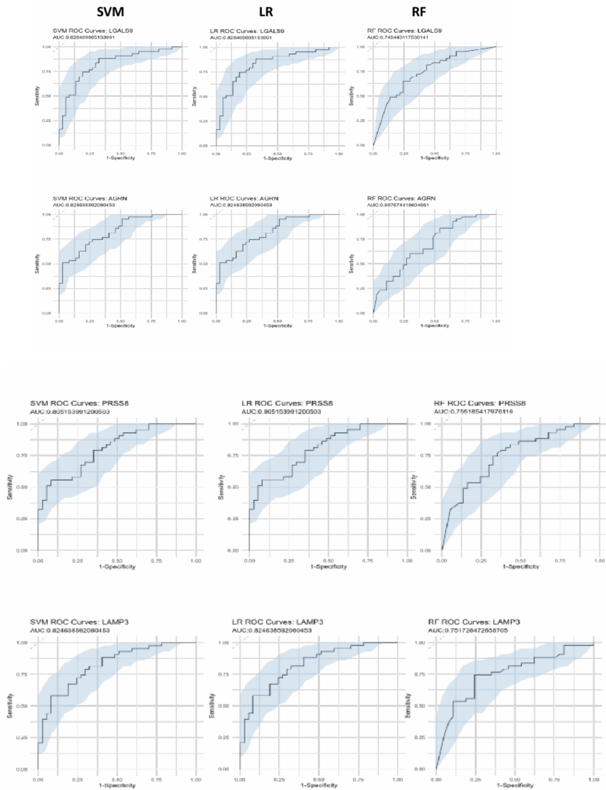
Figure 3. Univariate Machine Learning Predictions for Hospitalisation Risk. Univariate ROC curves from SVM, LR, and RF models for LGALS9, AGRN, PRSS8 and LAMP3 with labelled AUC scores and
