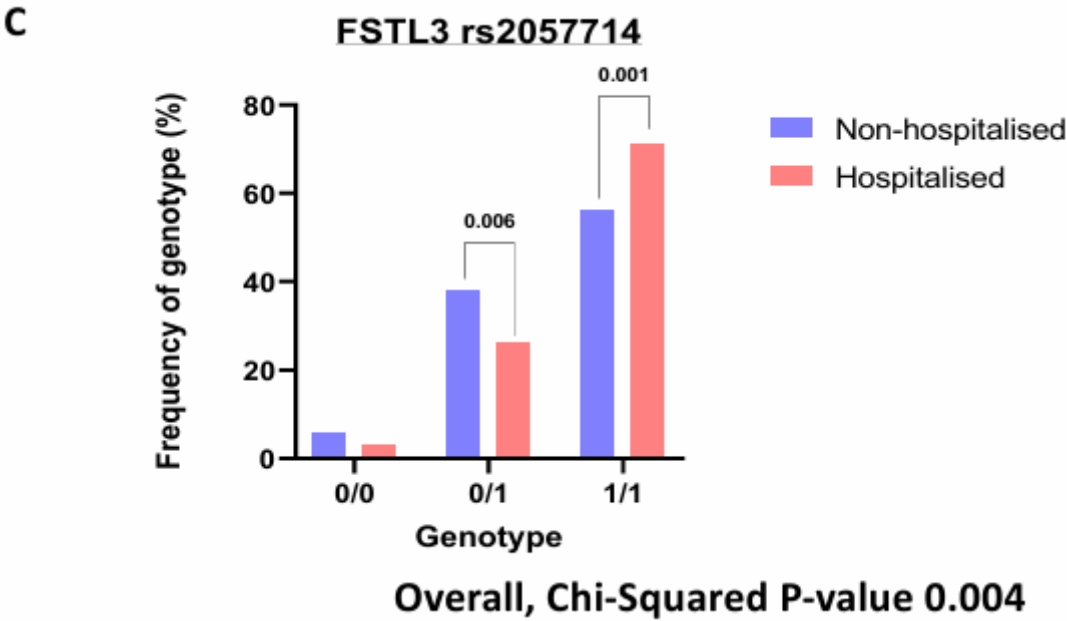
Figure 5. Genotyping Analysis on key Signatures. Bar charts demonstrating the percentage of each patient (hospitalised v non-hospitalised) and their genotypes respective to each rsID. Where 0/0 represents the homozygous reference genotype, 0/1 represents the heterozygous genotype and 1/1 represents the homozygous alternative genotype. (A). FSTL3 rs1046253. (B). FSTL3 rs2057713. (C). FSTL3 rs2057714.
