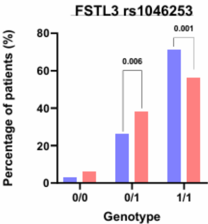
Figure 5: Genotyping analysis on key signatures
