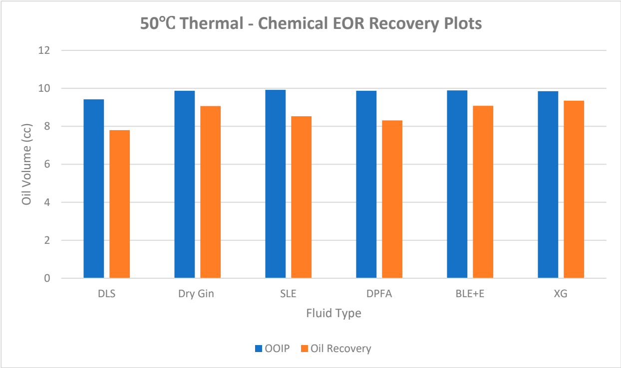
Figure 3. Graph of OOIP and Oil Recovery for the Fluid samples at 50°C.
