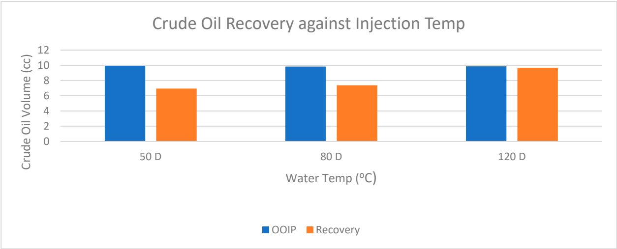
Figure 8. Graph of OOIP and Oil Recovery for varying hot water/steam temperatures.
