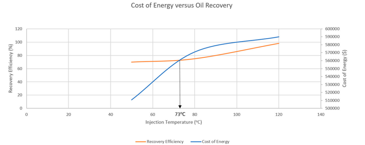
Figure 9. Graph of RE & COE for varying hot water/steam temperatures.
