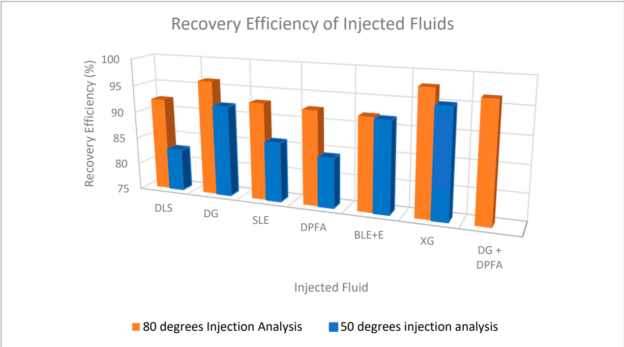
Figure 7. 80°C vs 50°C Chemical injection Oil Recovery efficiency comparison.
