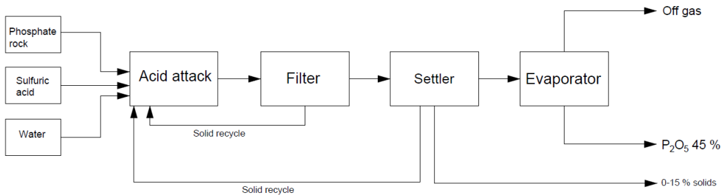
Figure 7. Simplified block flow diagram of Dihydrate process.
