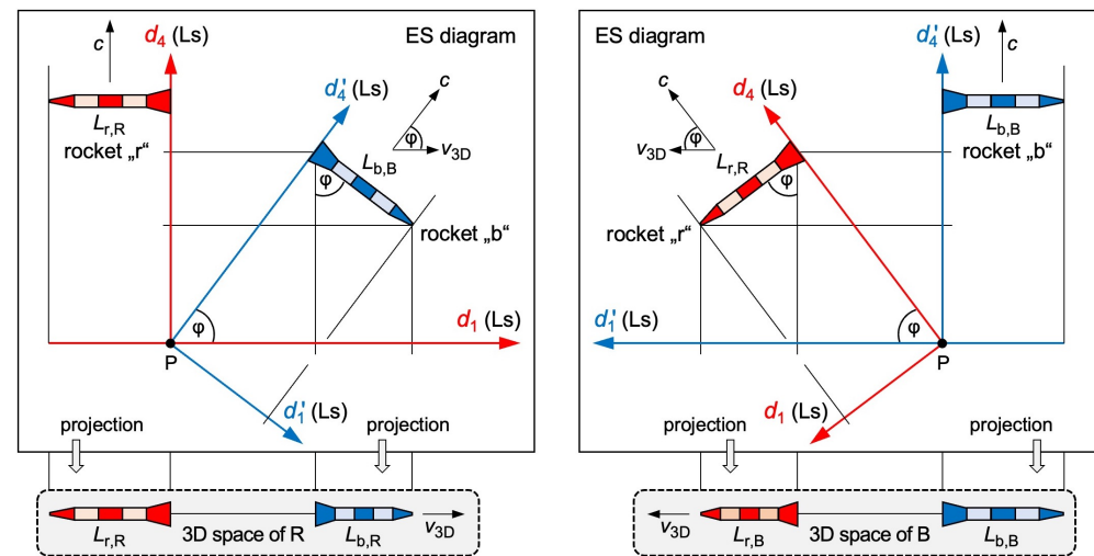
Fig. 3. ES diagrams of two rockets "r" and "b". Observer R (or B) is in the rear end of "r" (or else "b"). Left: "r" moves in the d_4 axis. "b" moves in the d'_4 axis. In the 3D space of R, "b" contracts to L_{b,R} . Right: The ES diagram has been rotated only. In the 3D space of B, "r" contracts to L_{r,B} .
