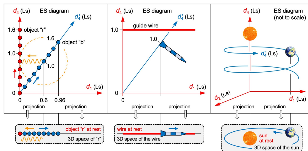
Fig. 5. Three problems. Left: In ES, an energy taking a detour (blue/orange arrow) does not collide with an energy moving straight (red arrow). In the 3D space of "r", it does. The circle shows a signal emitted by "b". Center: In ES, the wire escapes from the rocket. In the 3D space of the wire, it does not. Right: In ES, the sun escapes from Earth's orbit. In the 3D space of the sun, it does not.
