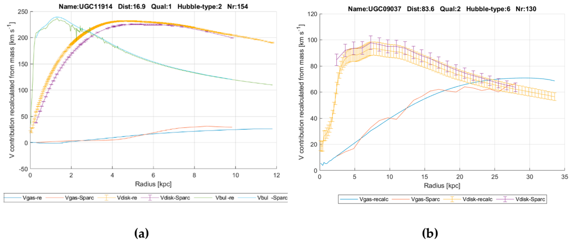
Figure 2. V_{gas} , V_{disk} and V_{bulge} from SPARC team and from author assuming mass-light-ratio Y_{ml} = 1 (a) UGC11914; (b) UGC09037; the complete figure set of 175 figure is available in Annex 1.
