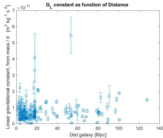
Figure 6. G_L for all 175 galaxies.
