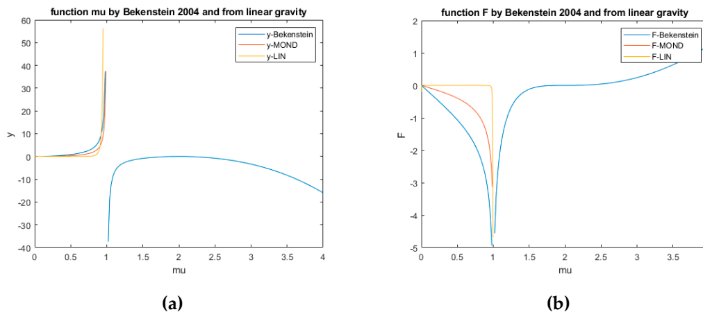
Figure 7. Function y(\mu) of Bekenstein and linear gravity (a) Function F(\mu) of Bekenstein and linear gravity (b).
