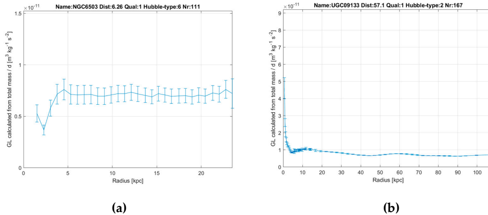
Figure 5. G_L as function of radius in galaxy examples (a) NGC6503; (b) UGC09133; the complete figure set of 175 figure is available in Annex 2.
