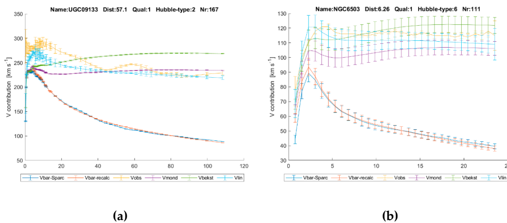
Figure 10. Examples of rotation curves with MOND, TeVeS and linear gravity predictions; (a) UGC09133, (b) NGC 6503; the complete figure set of 175 figure is available in Annex 3.
