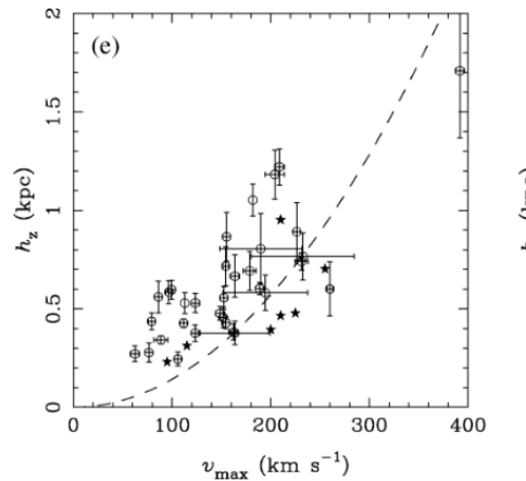
Figure 4. Vertical disk scale length vs. V_{\text{obs}} after de Kregel et al [32].
