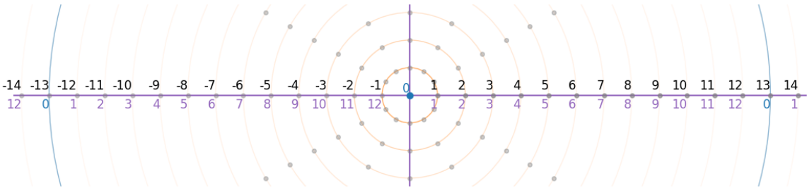
Figure 2. Class of signed pseudo-integers \mathbb{Z} over the finite framed field \mathbb{Z}_{13} . Black labels indicate the newly defined signed integers z \in \mathbb{Z} , while the purple labels represent the corresponding elements k(z) \in \mathbb{Z}_{13} . The blue line indicates the periodicity of the finite field. The unlabeled gray dots indicate the off-axis elements of \mathbb{Z}_{13} as they are observed from the top of the 2D spheroid described in Figure 1.
