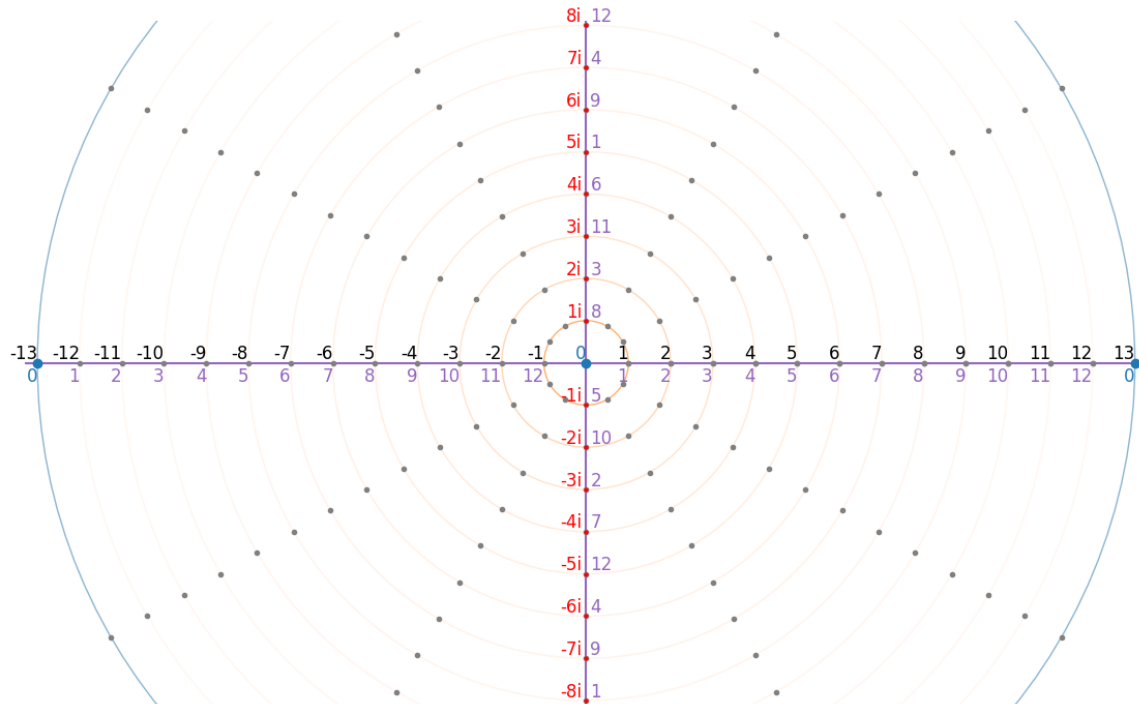
Figure 5. Pseudo-complex numbers plane \mathbb{C}_p in a finite framed field \mathbb{Z}_{13}(0,1) . Horizontal axis represents the pseudo-reals \mathbb{R}_p on the prime meridian and the vertical axis represents the imaginary numbers c = z \cdot i indicated by their respective red labels. The corresponding elements k(c) are depicted in purple. The blue line indicates the periodicity of the finite field.
