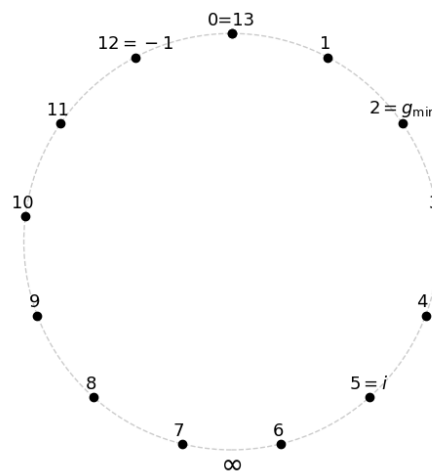
Figure 6. State space of a finite framed field \mathbb{F}_{13} , visualized as a circle on a 2D plane with the major structural elements -1, 0, 1, g_{\min}, i , as well as \infty indicated.
