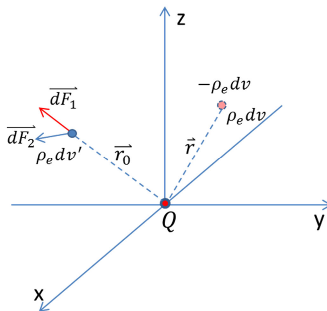
Figure 3. Sketch illustrating some of the charge interactions within a polarized vacuum. Charge Q exerts a force \vec{F}_1 on charge \rho_e dv' in the vacuum, while positive-negative charge pairs (\rho_e dv, -\rho_e dv) also exert a force \vec{F}_2 on charge \rho_e dv' .
