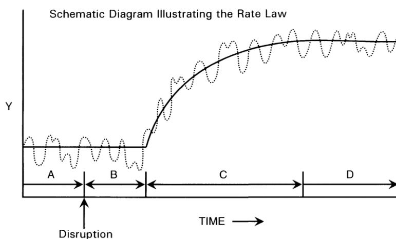
Figure 1. Representation of Rate Law [47].
