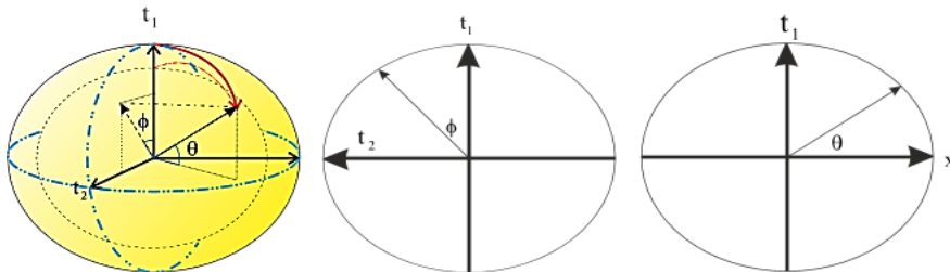
Figure 6. Figure 6: Variations in density lead to the eccentricity of the ellipse, and this eccentricity, in turn, generates an inner centrality within the closed manifold. Consequently, the rigid body co-rotates with the expansion of space around the mass field.
