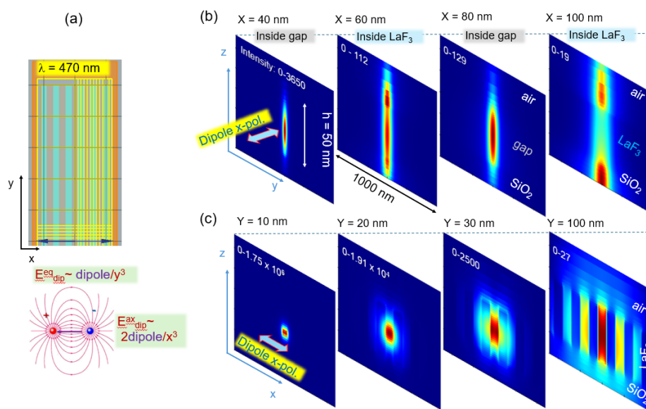
Figure 8. Toy-model. FDTD simulation of dipole field inside form-birefringent region with dipole along the n_e (fast axis). (a) Top-view scene with parameters: \Lambda = 40 nm period, dipole location is at (x, y) = (0, 0) and middle of the structure at z = 25 nm. The perfectly matched layer (PML) conditions were used with different-sized meshing for high resolution. Bottom-inset shows the dipole, and its E-fields on axis and equator. (b) E-field enhancement on (Y, Z) -plane at different X -position. (c) E-field enhancement as the emitted power ratio on the (X, Z) -plane at different Y -positions. The enhancement range of the cold-hot maps is shown as intensity in (c,d).
