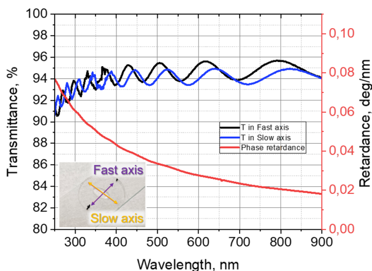
Figure 4. Transmittance along fast and slow axes and phase retardance \Gamma_\lambda = \frac{360^\circ}{\lambda \Delta n} [degrees/nm] for linearly polarised beams. The inset shows the un-capped sample with a drop of RhD6G solution. For \lambda = 300 nm, the thickness of \lambda/4 -plate d = 360^\circ / \Gamma_\lambda = 1.5 \mu\text{m} ; where \Gamma_\lambda = 0.06 deg/nm.
