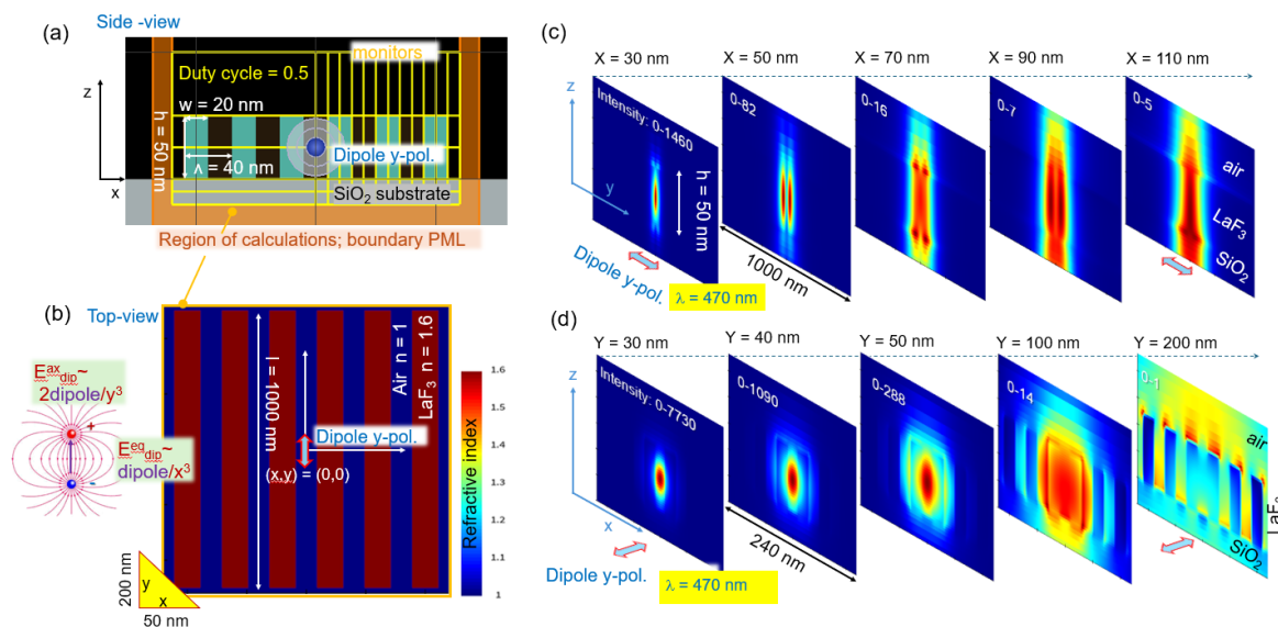
Figure 7. Toy-model. FDTD simulation of dipole field inside form-birefringent region. (a) Side-view scene with parameters: \Lambda = 40 nm period, dipole location is at (x, y) = (0, 0) and middle of the structure at z = 25 nm. (b) Top-view of refractive index monitor over the entire calculation region with perfectly matched layer (PML) conditions. The inset shows the dipole, and its E-fields on axis and equator. (c) E-field enhancement on (Y, Z) -plane at different X -position. (d) E-field enhancement as the emitted power ratio on the (X, Z) -plane at different Y -positions. The enhancement range of the cold-hot maps is shown as intensity in (c,d).
