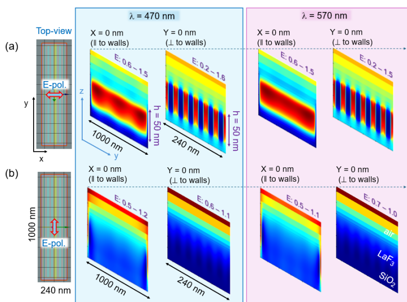
Figure A1. Toy-model. FDTD simulation of plane wave illumination of the form-birefringent structure at two perpendicular polarisations along fast-axis (a) and slow-axis (b)(the same structure was used in Figures 7-8). The periodic boundary conditions (PBC) were used with different-sized meshing for high resolution. Incident E-field is normalised |E| = 1 .
