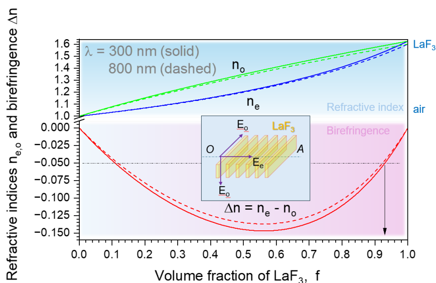
Figure 5. Form birefringence (negative) \Delta n = n_e - n_o of \text{LaF}_3 3D grating with volume fraction of material f = w/\Lambda , where w is the width of the \text{LaF}_3 plane and \Lambda is the period. Arrow marks f \approx 93\% volume fraction of |\Delta n| = 0.05 . Refractive indices used: 1.6253 (at \lambda = 300 \text{ nm} ) and 1.6007 (800 nm). Inset shows the geometry of the form birefringent structure.
