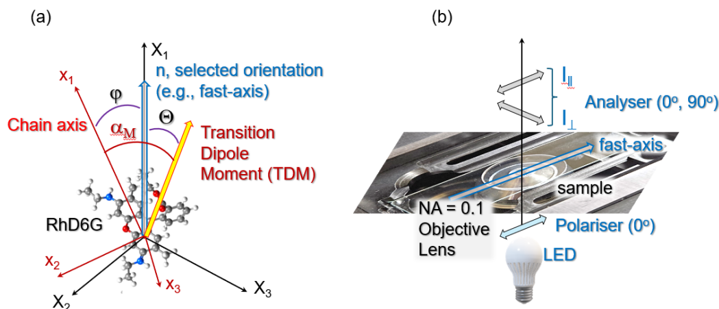
Figure 3. a Orientation of transition dipole moment (TDM) in respect to the selected direction, which is set to coincide with X_1 -axis of the coordinate system X_1X_2X_3 . The orientation of molecular (or chain) direction is selected along the x_1 -axis, where \alpha_M is the orientation angle of the dipole. The angle \varphi defines the tilt between two coordinate systems. (b) FLIM methodology: polarised incident light excites fluorescence of selected (aligned) molecular dipoles and emission is measured in two perpendicular orientations.
