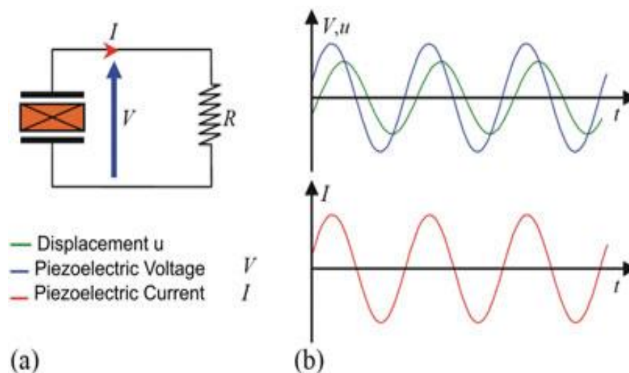
Figure 1. Standard approach Alternating Current (AC) to energy harvesting : (a) standard network and (b) standard waveforms.
