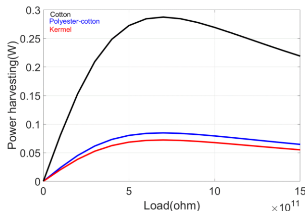
Fig.3. The power harvested as a function of resistive load for cotton, polyester-cotton and Kermel substrates when applying force F=80\text{N} at 6\text{Hz} .
