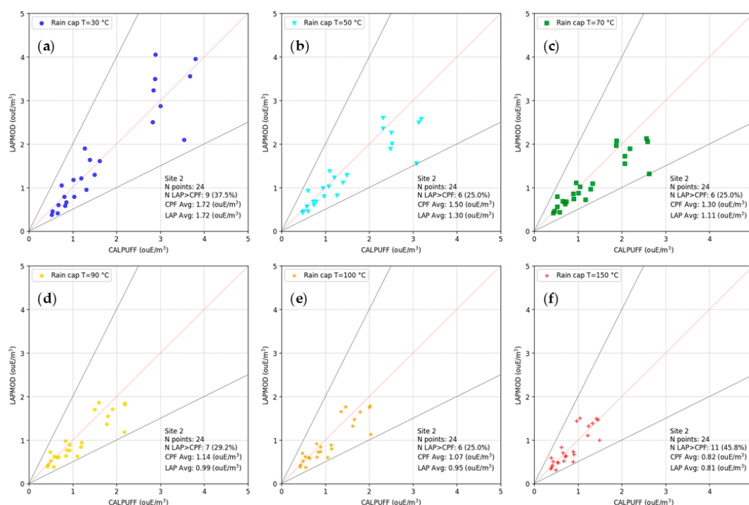
Figure 8. Site 2. Scatter plot of the 98 th percentile of hourly peak concentrations of LAPMOD versus CALPUFF for different emission temperatures: (a) T=30 °C; (b) T=50 °C; (c) T=70 °C; (d) T=90 °C; (e) T=100 °C; (f) T=150 °C. Vertical stack with rain cap.
