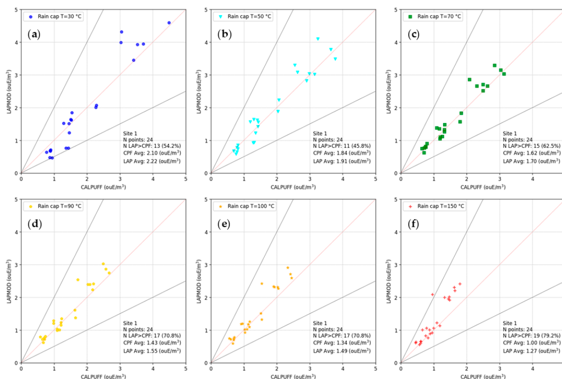
Figure 6. Site 1. Scatter plot of the 98 th percentile of hourly peak concentrations of LAPMOD versus CALPUFF for different emission temperatures: (a) T=30 °C; (b) T=50 °C; (c) T=70 °C; (d) T=90 °C; (e) T=100 °C; (f) T=150 °C. Vertical stack with rain cap.
