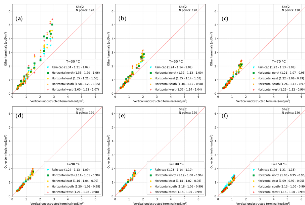
Figure 10. Site 2. Scatter plot of the 98 th percentile of hourly peak concentrations predicted by LAPMOD for different terminal types versus those predicted for a vertical unobstructed stack for different emission temperatures: (a) T=30 °C, (b) T=50 °C; (c) T=70 °C; (d) T=90 °C; (e) T=100 °C; (f) T=150 °C.
