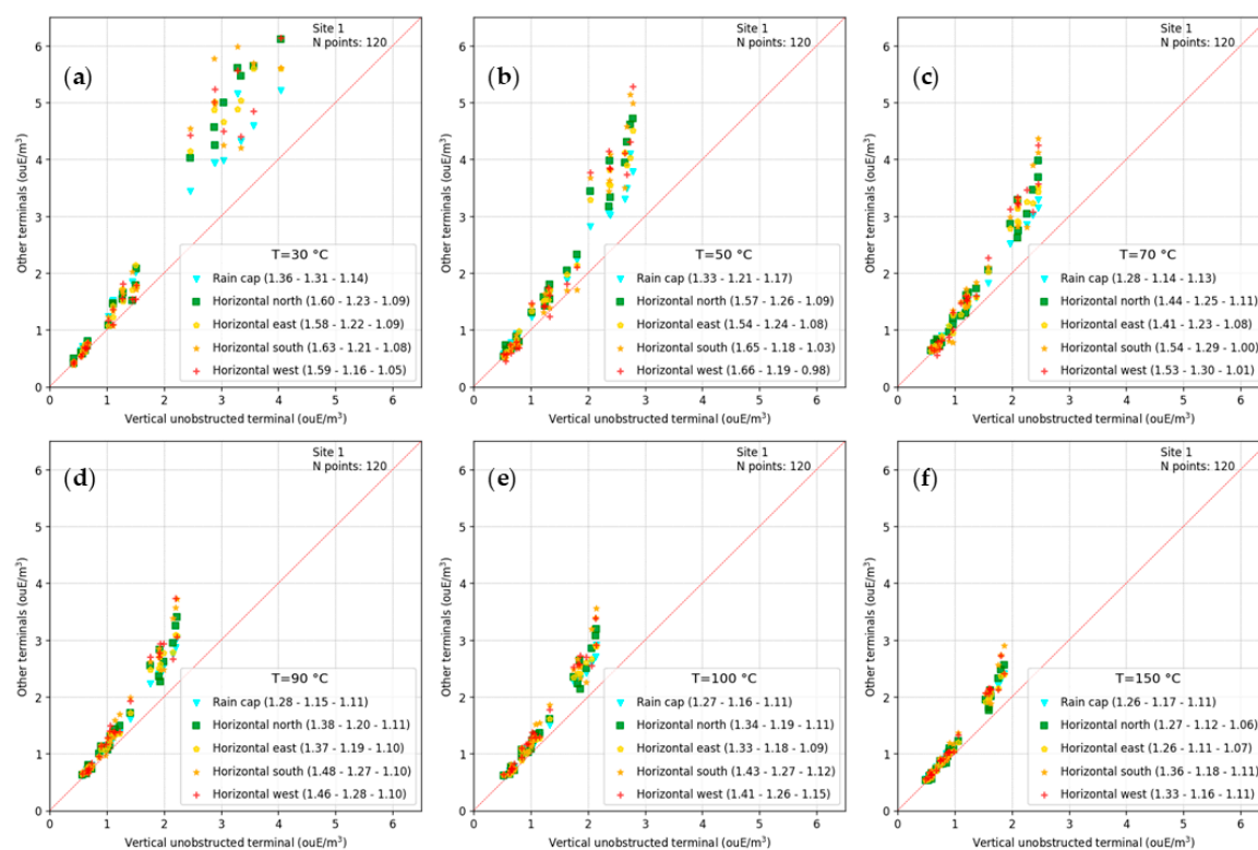
Figure 9. Site 1. Scatter plot of the 98 th percentile of hourly peak concentrations predicted by LAPMOD for different terminal types versus those predicted for a vertical unobstructed stack for different emission temperatures: (a) T=30\text{ }^{\circ}\text{C} ; (b) T=50\text{ }^{\circ}\text{C} ; (c) T=70\text{ }^{\circ}\text{C} ; (d) T=90\text{ }^{\circ}\text{C} ; (e) T=100\text{ }^{\circ}\text{C} ; (f) T=150\text{ }^{\circ}\text{C} .
