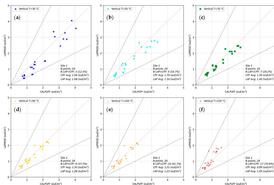
Figure 5. Site 1. Scatter plot of the 98 th percentile of hourly peak concentrations of LAPMOD versus CALPUFF for different emission temperatures: (a) T=30 °C, (b) T=50 °C; (c) T=70 °C; (d) T=90 °C; (e) T=100 °C; (f) T=150 °C. Vertical unobstructed stack.
