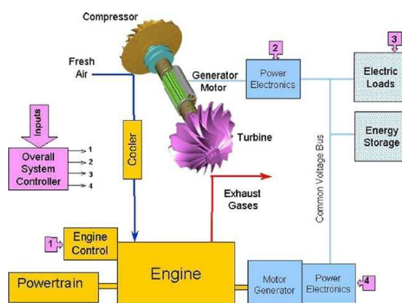
Figure 5. Schematic of electric turbo compound [14].
