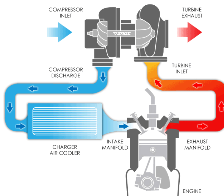
Figure 1. Connection between turbocharger and engine [4].
