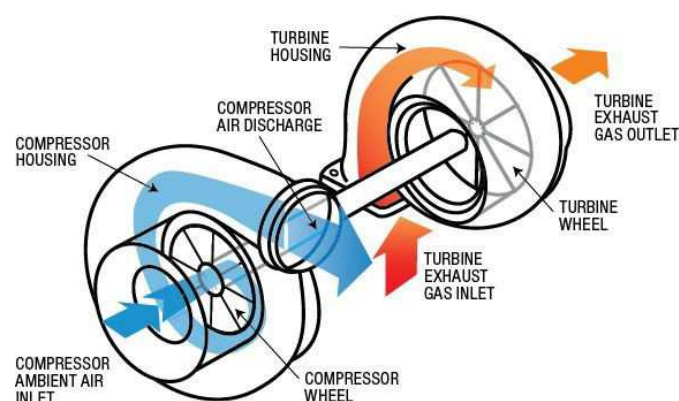
Figure 3. Turbocharger assembly [10].
