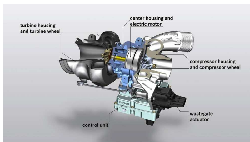
Figure 7. Different manufacturer's construction solution [23].
