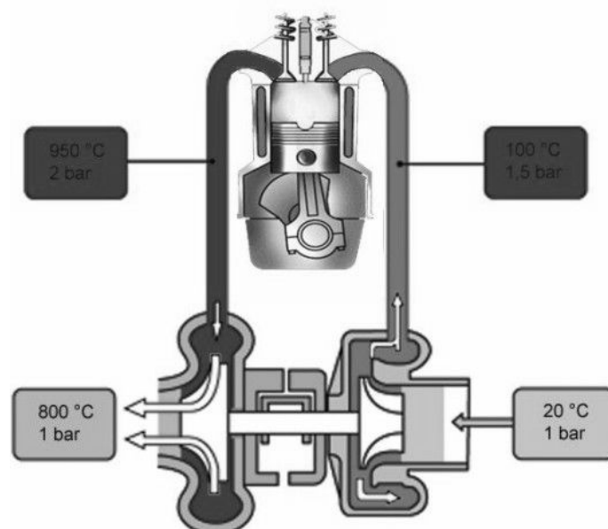
Figure 2. Turbocharger block diagram [7].
